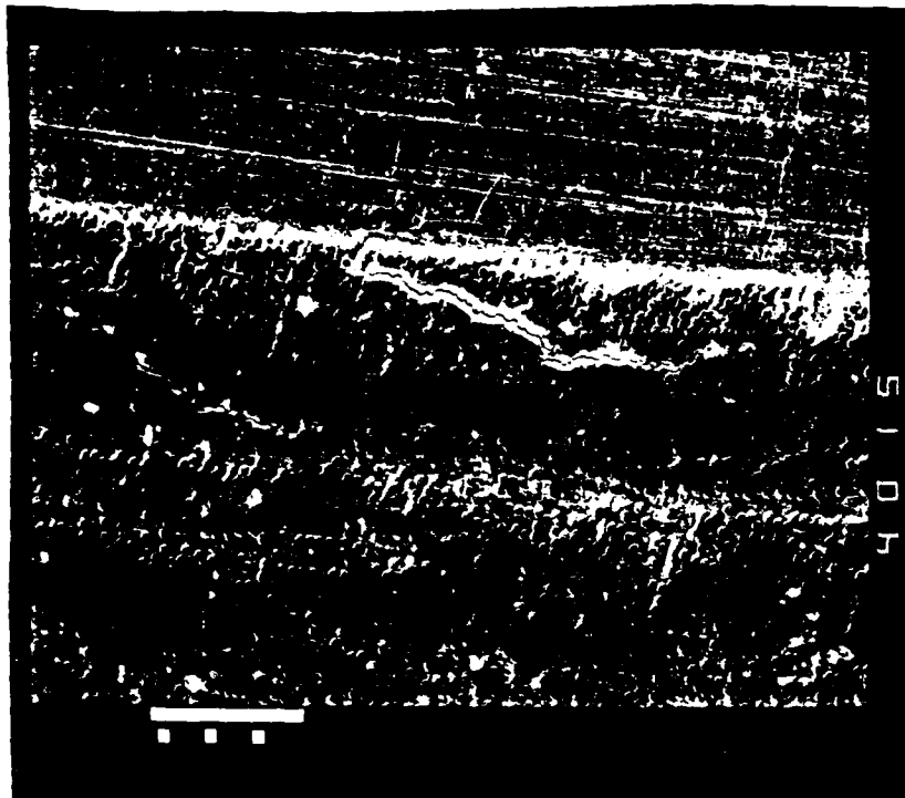
Figure 8. Two major horizontal cracks in the laminate subjected to the same conditions as listed in Fig. 4.
