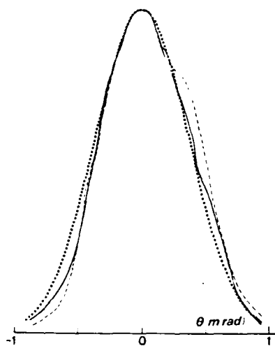
Fig. 6. — Experimental laser horizontal (—) and vertical (---) transverse profiles and the calculated (...) cavity \text{TEM}_{00} profile
