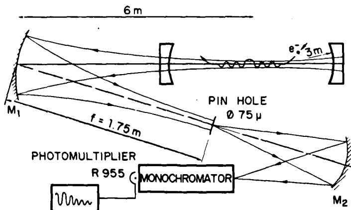
Figure 1. Experimental set-up
