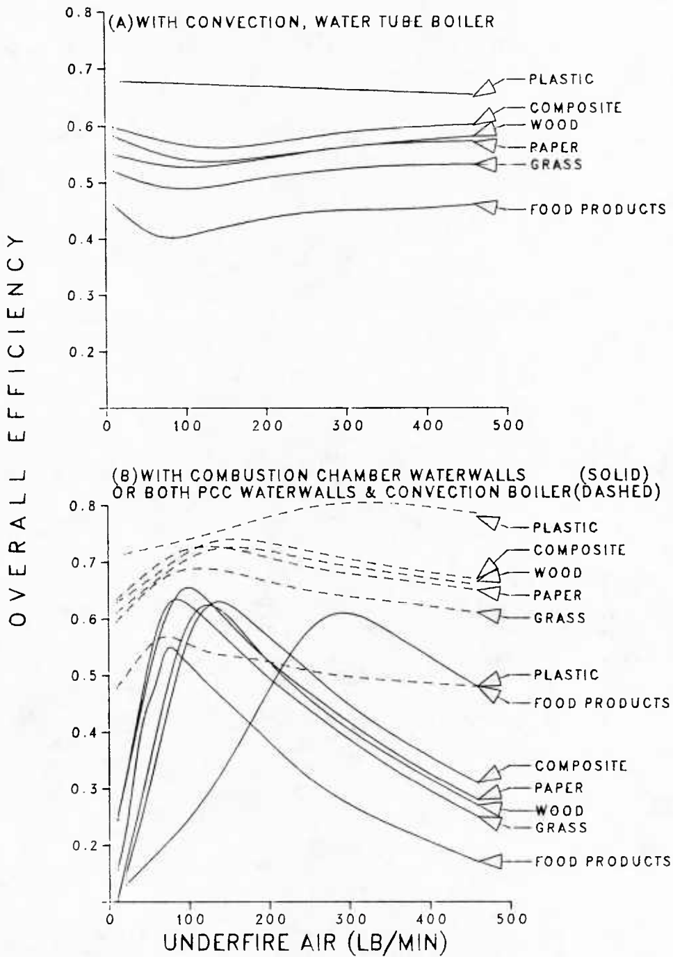
Figure 11. Effect of type of waste on the overall thermal efficiency of an energy recovery incinerator.
