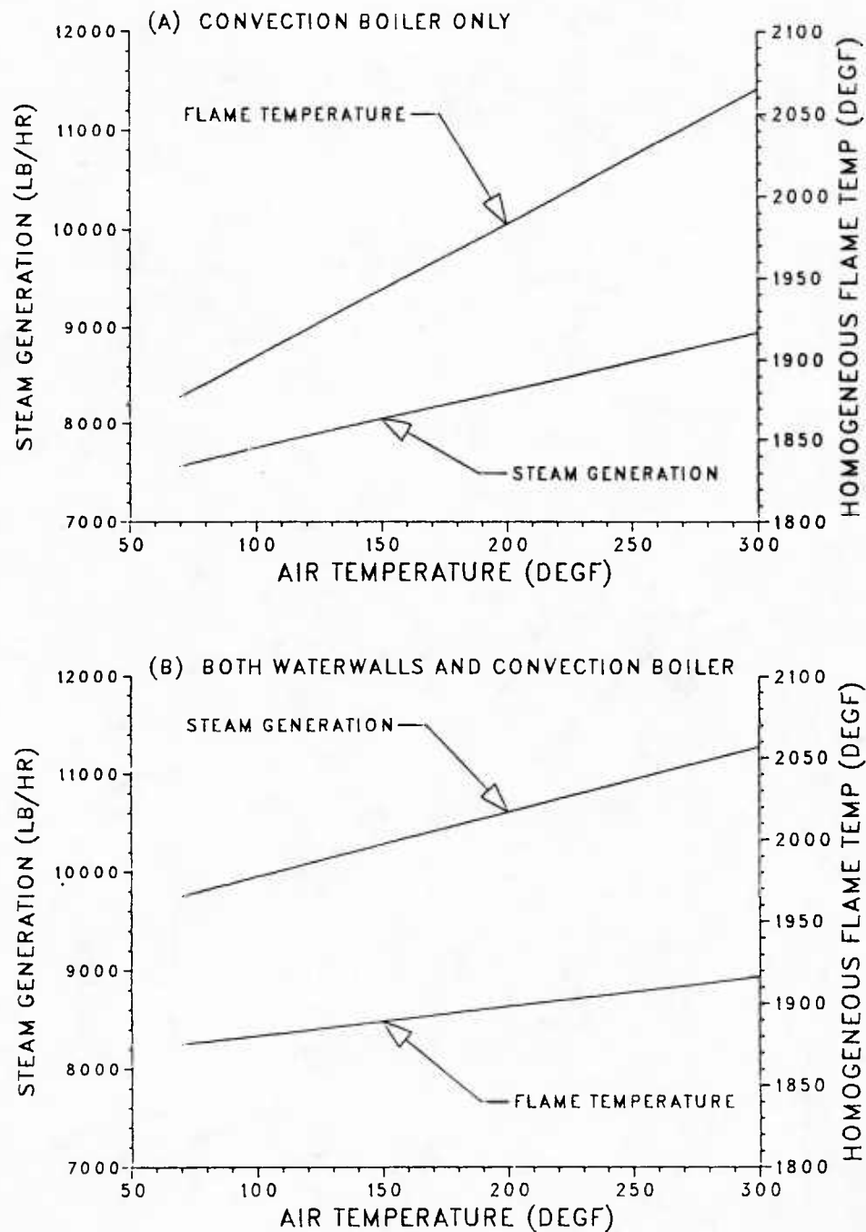
Figure 7. Effect of initial temperature of the combustion air on incinerator operation.
