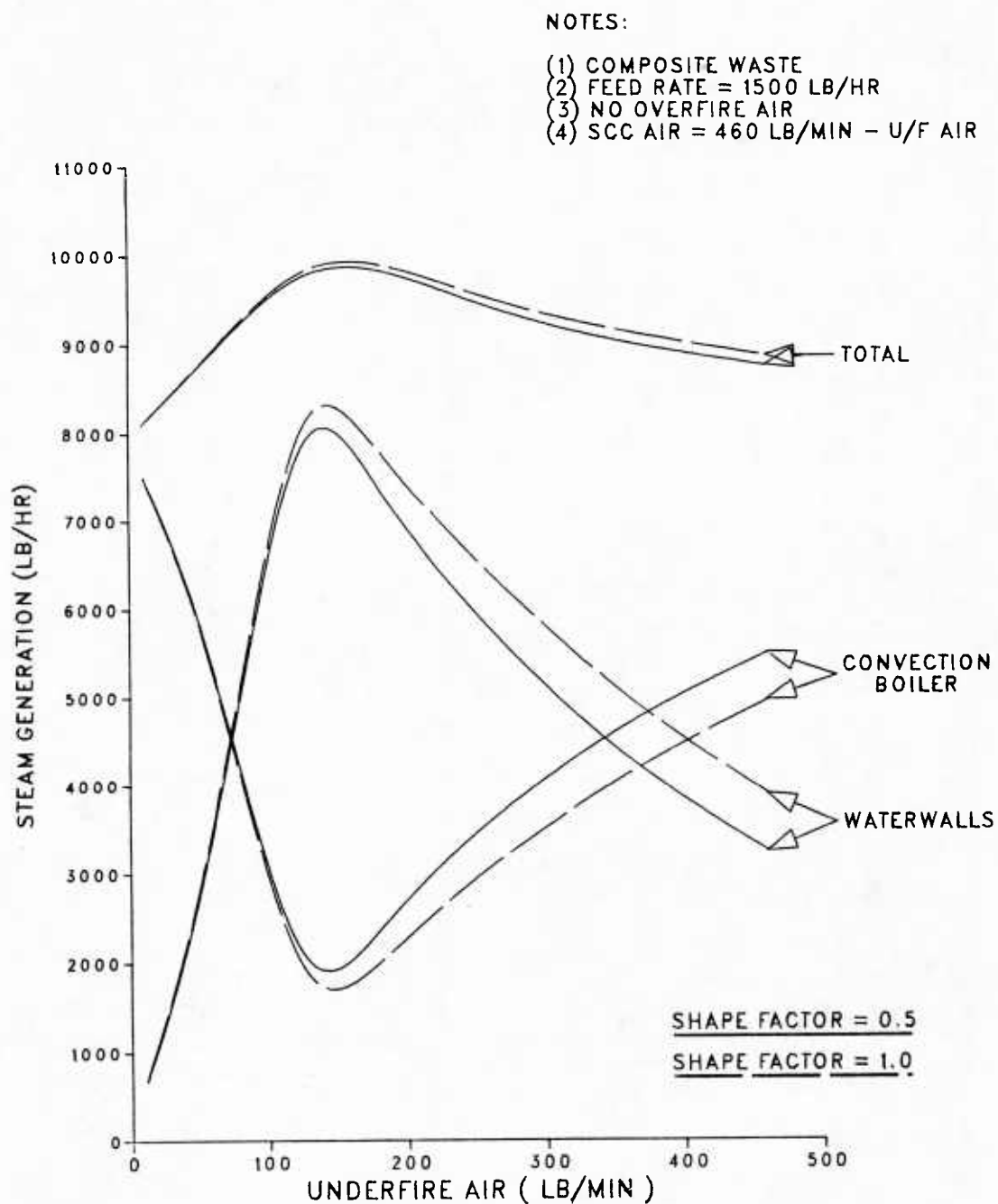
Figure 21. Effect of radiation shape factor between flame and waterwalls on incinerator steam generation rates.
