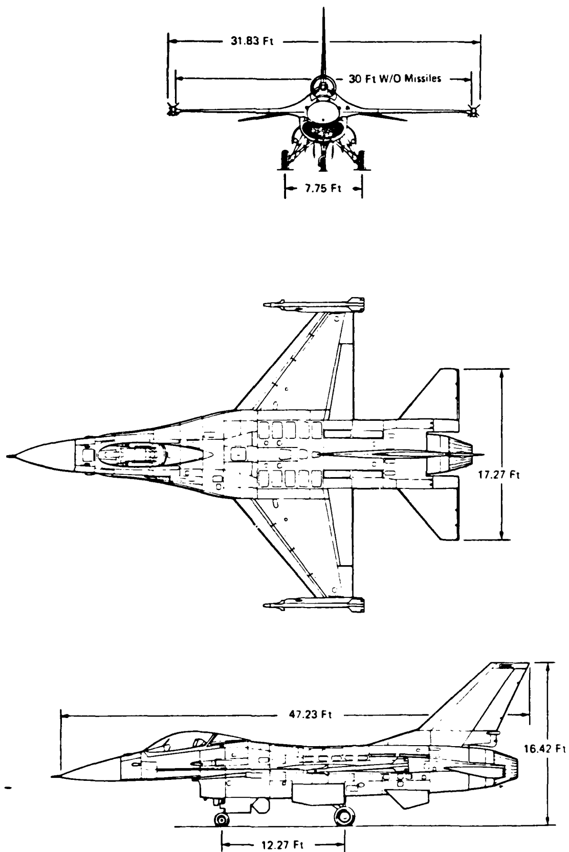
FIGURE 1. F-16 AIRCRAFT
