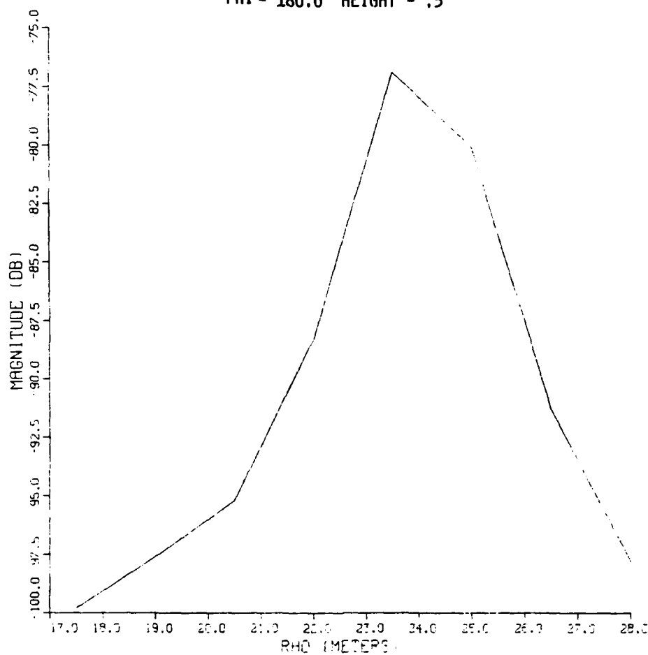
PLOT OF |EY| IN DB .VS. RHO NO GROUND REFLECTION, NO SCATTERER PHI - 180.0 HEIGHT - .5
