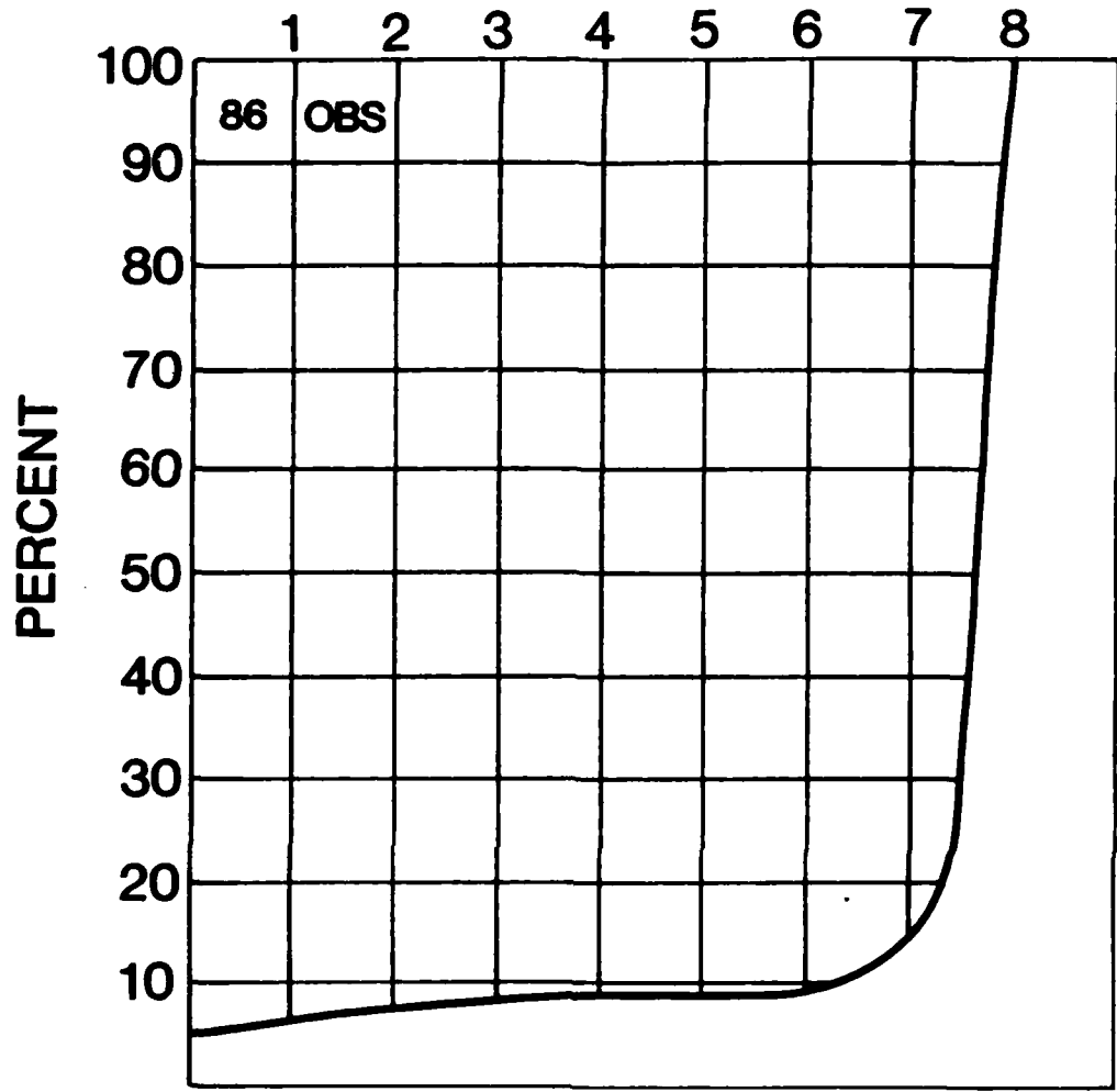
Fig. 5. Cloud Amount Distribution Over the Water (U.S. Navy, 1963)
