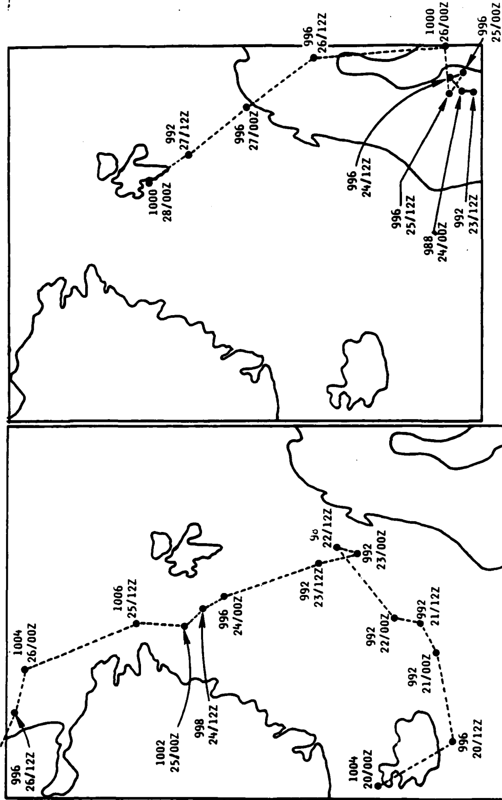
Fig. 23. Track of Storm Number 4
