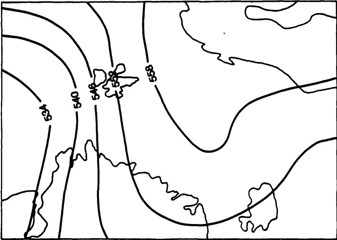
Fig. 39. (a) (Left) 500 mb Analysis for 0000 GMT on 12 July 84 (b) (Above) Surface Plot for 0000 GMT on 12 July 84
