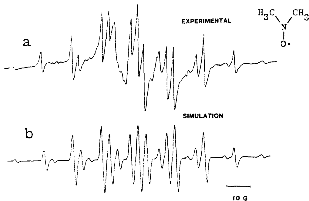
Fig. 2. The first derivative e.s.r. spectrum of a dimethyl nitroxyl radical is shown. This spectrum remains stable for ca. 30 minutes. A simulated spectrum using the couplings listed in the text is shown for comparison.
