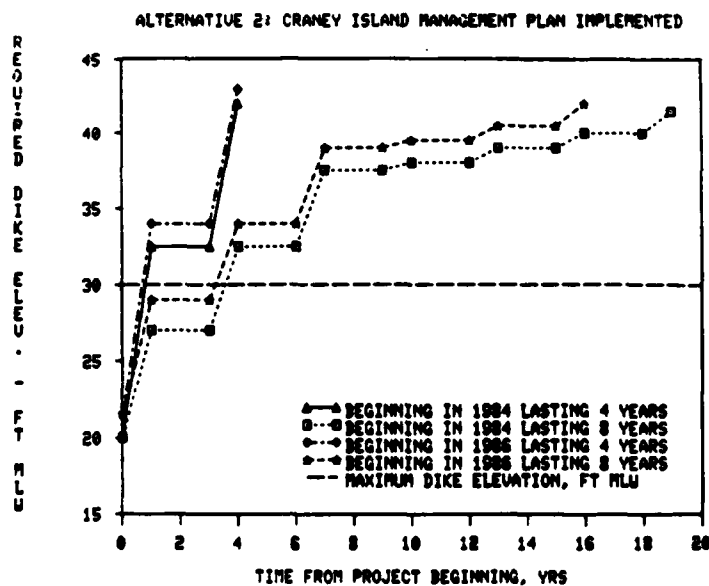
Figure 3. Dike raising requirements for Alternative 2.
