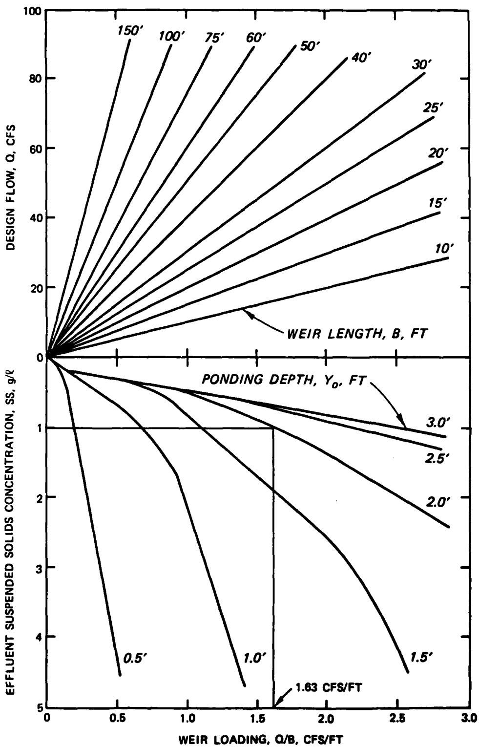
Figure 17: Nomogram relating weir design parameters (after Walski and Schroeder 1978).
