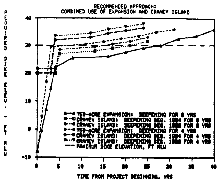
Figure 6. Dike raising requirements for the recommended approach.
