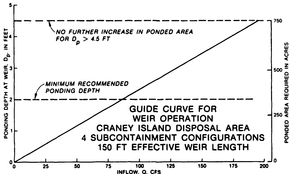
Figure 7. Guide curve for weir operation, 150-ft effective weir length four-subcontainment area configuration
