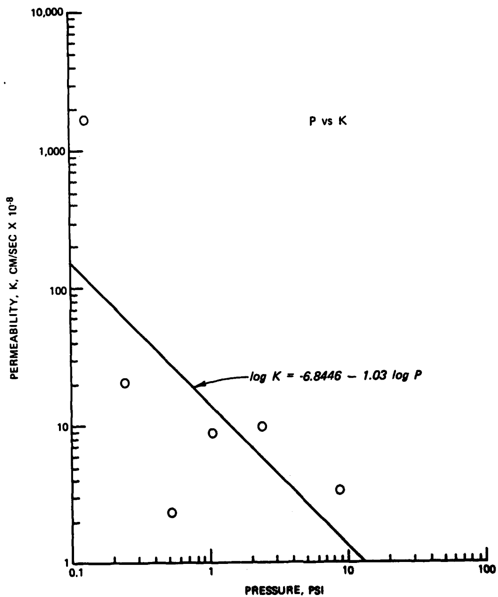
Figure 21: Coefficient of permeability versus log pressure.
