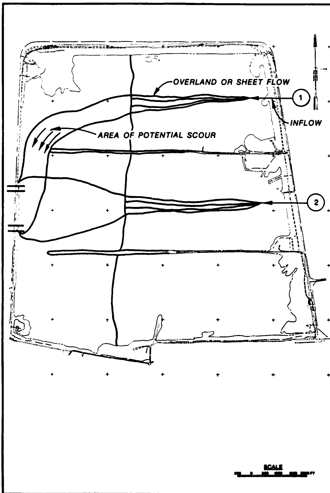
Figure 18: Points of inflow and weirs for interim operation (from CIMP).
