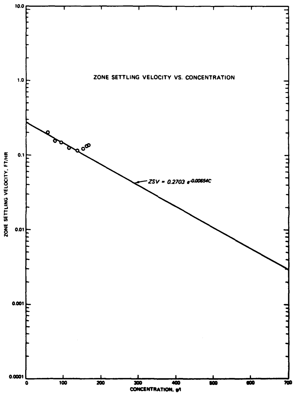
Figure 14: Zone settling velocity versus concentration for new work sediment.
