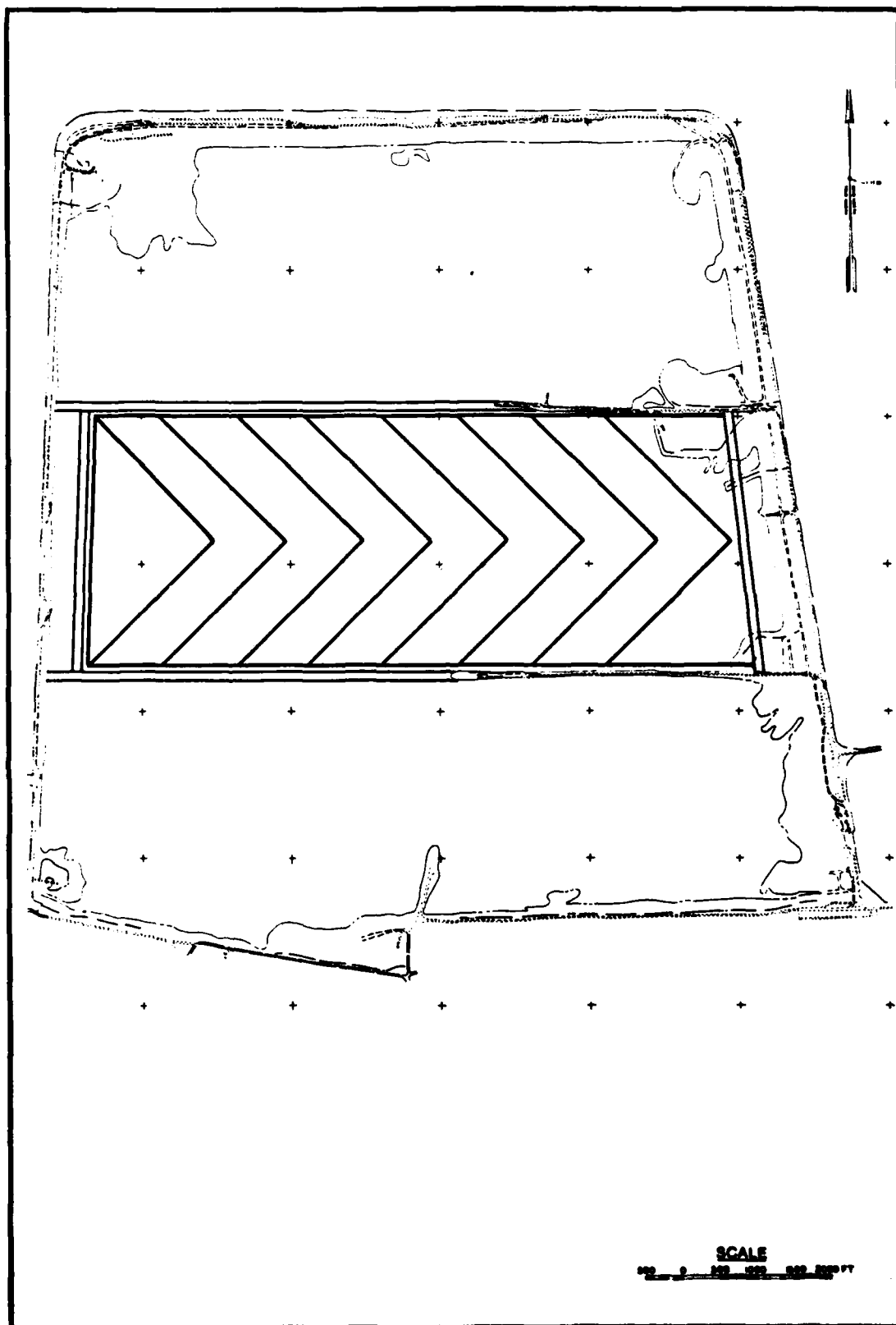
Figure 9. Interior trench layout for dredged material dewatering (from CIMP)
