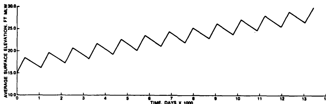
Figure 29. Extended storage capacity projection for three-subcontainment configuration with surface water management and active dewatering (from CIMP).
