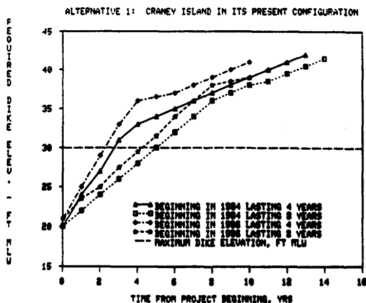
Figure 2. Dike raising requirements for Alternative 1.
