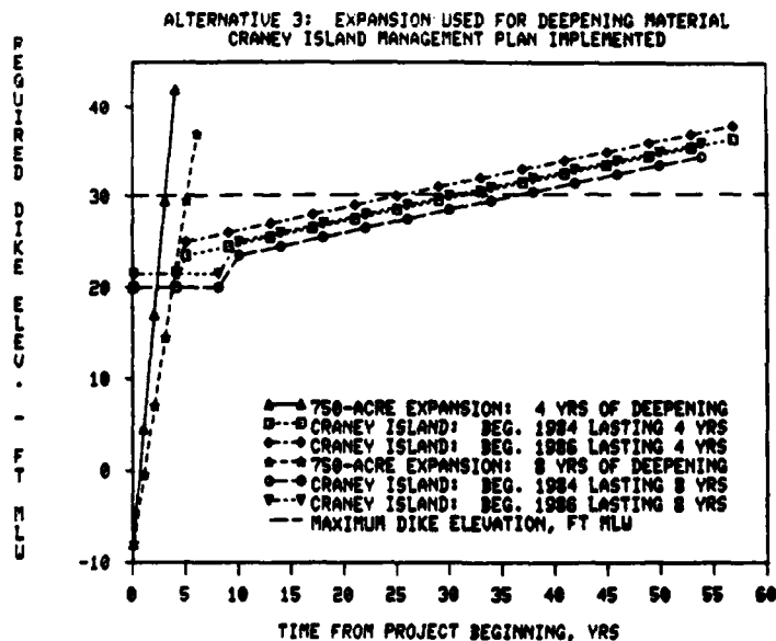
Figure 5. Dike raising requirements for Alternative 3.
