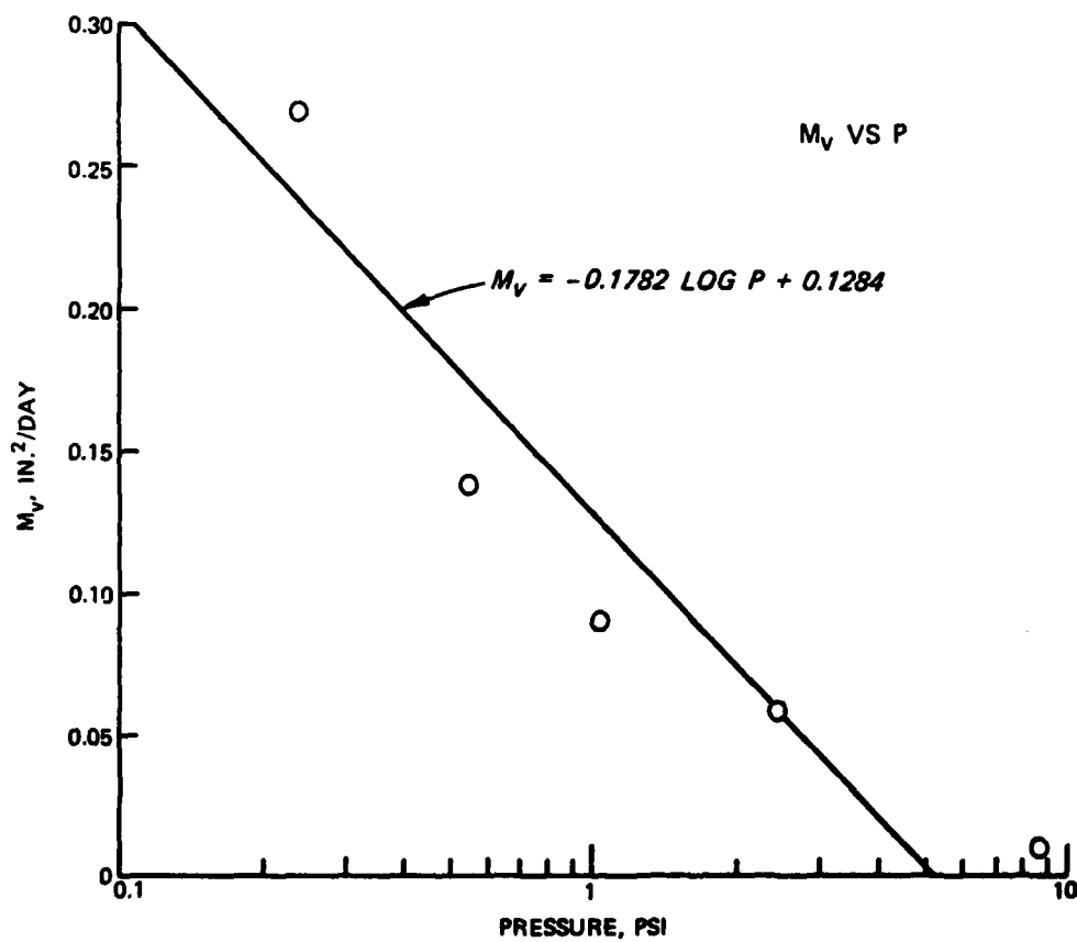
Figure 19: Coefficient of volume compressibility versus log pressure.
