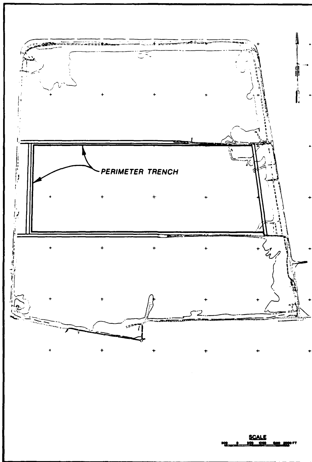
Figure 8. Periphery trench layout for dredged material dewatering (from CIMP)
