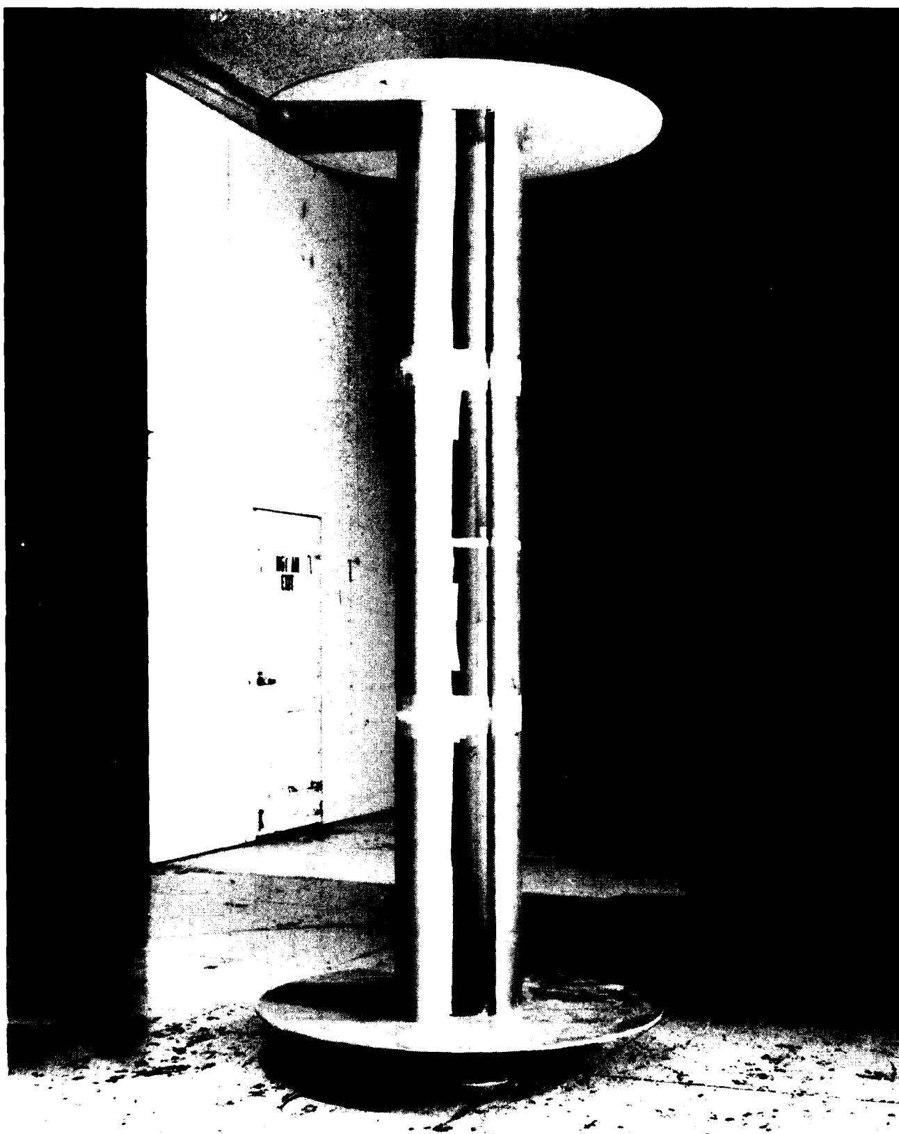
Figure 4. Two-dimensional test apparatus in the Langley 4- by 7-Meter Tunnel. AH-64 cross section shown.
