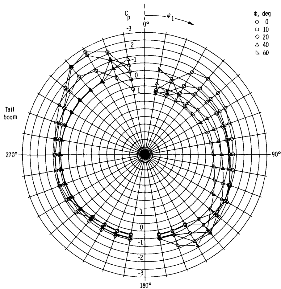
Figure 25. Effects of flow incidence on pressure distributions on UH-60 shape without TRSC at q = 15 psf.
