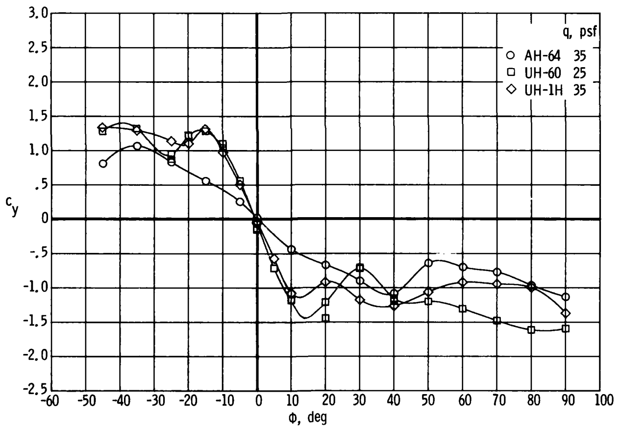
Figure 7. Comparison of effects of flow incidence on drag and side force of AH-64, UH-60, and UH-1H shapes with TRSC on.
