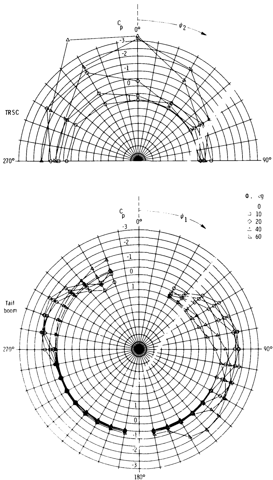
Figure 16. Effects of flow incidence on pressure distributions for the AH-64 shape with TRSC at q = 35 psf.
