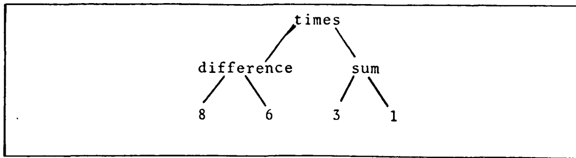
Figure 1.1 S-expression Tree.
