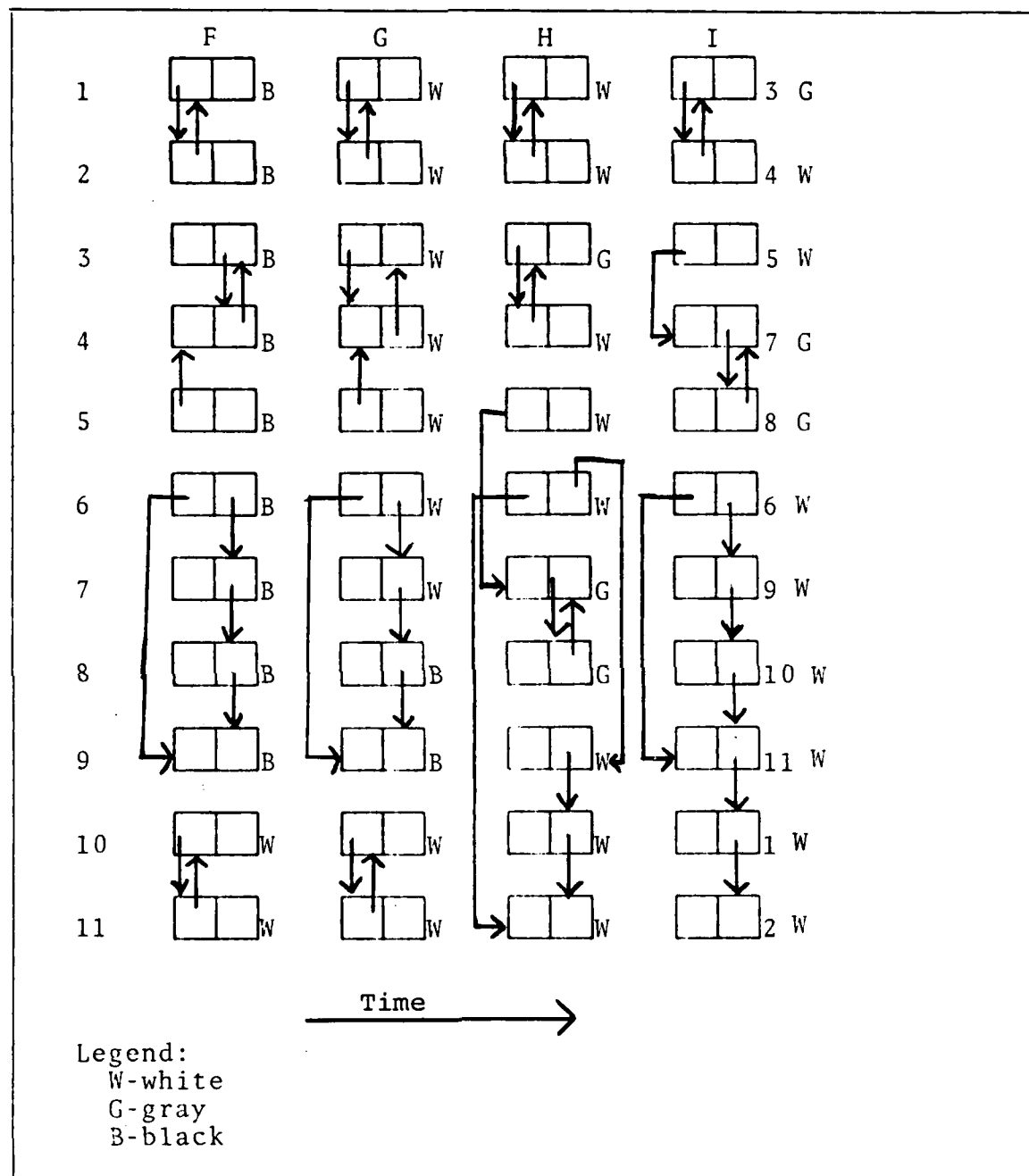
Figure 5.3 Memory Snapshot During the Scan Phase.
