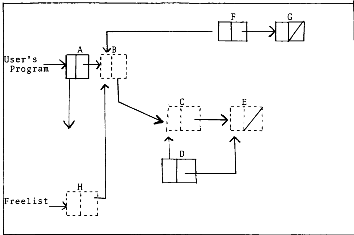
Figure 2.1 Dangling Reference Example.
