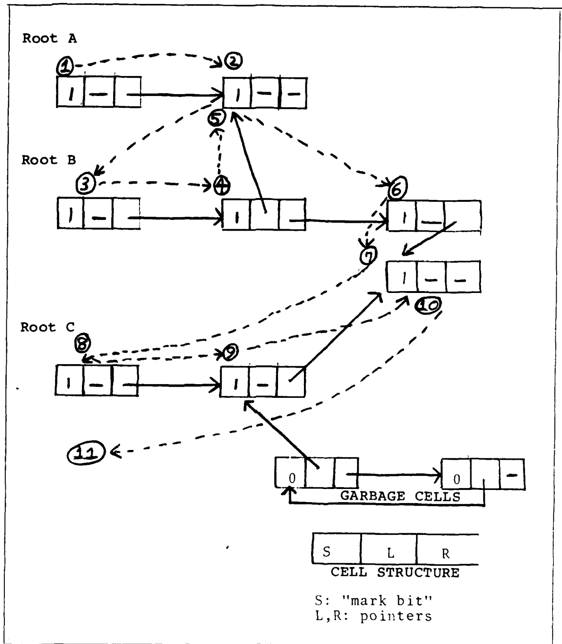
Figure 3.2 Marking Phase Example.
