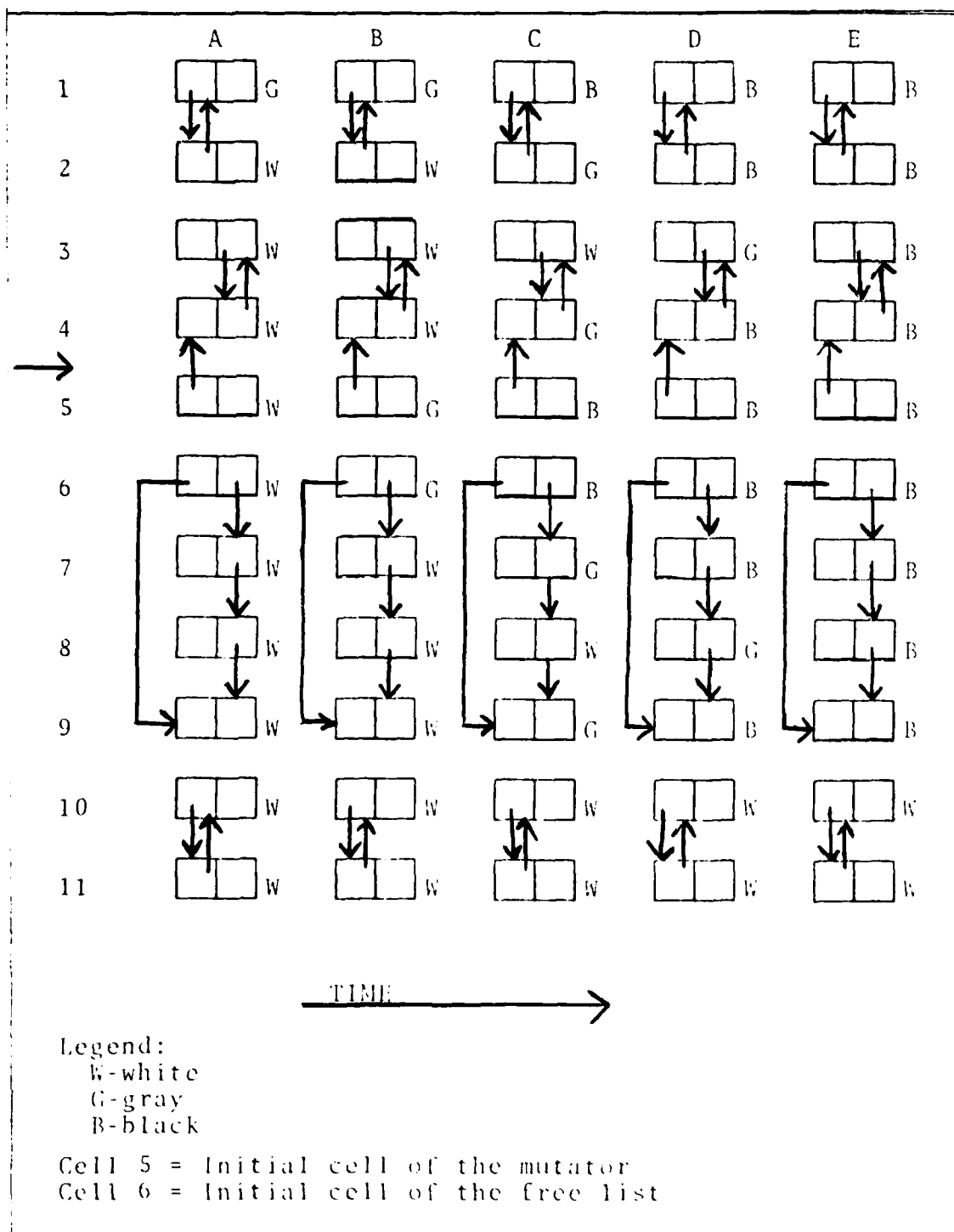
Figure 5.2 Memory Snapshot During Mark Phase.
