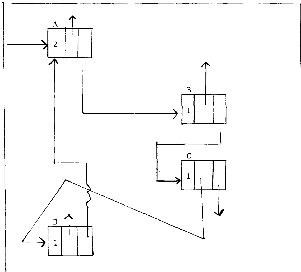
Figure 2.3 Circular List Structure.
