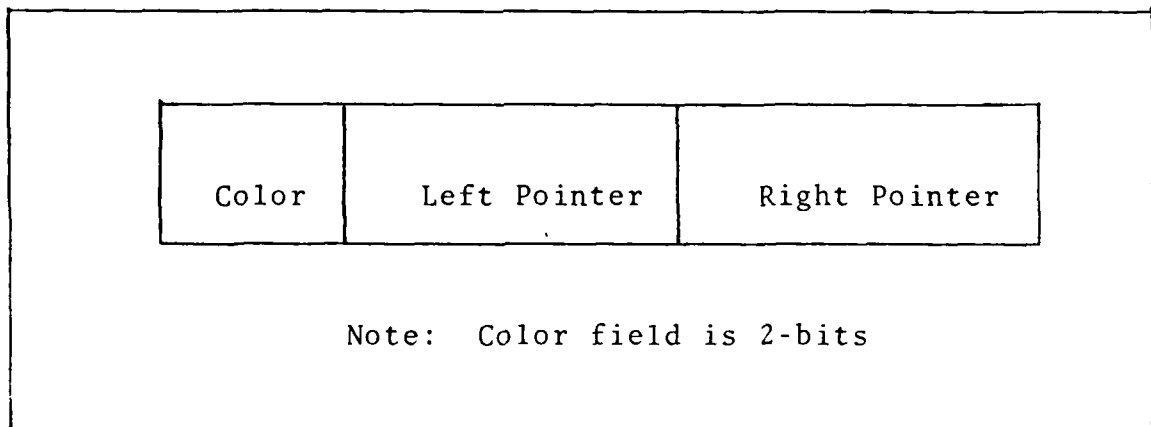
Figure 5.1 Three-Color Cell Format.
