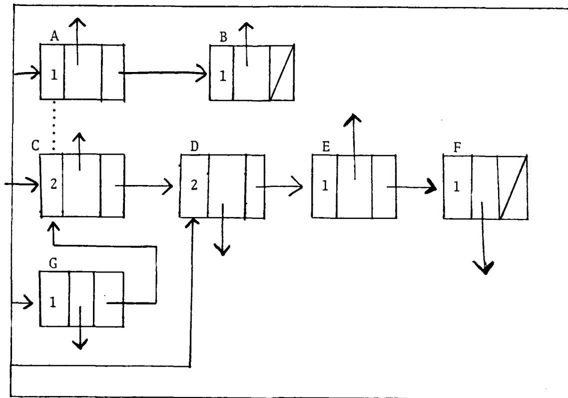
Figure 2.2 Reference Count Example.
