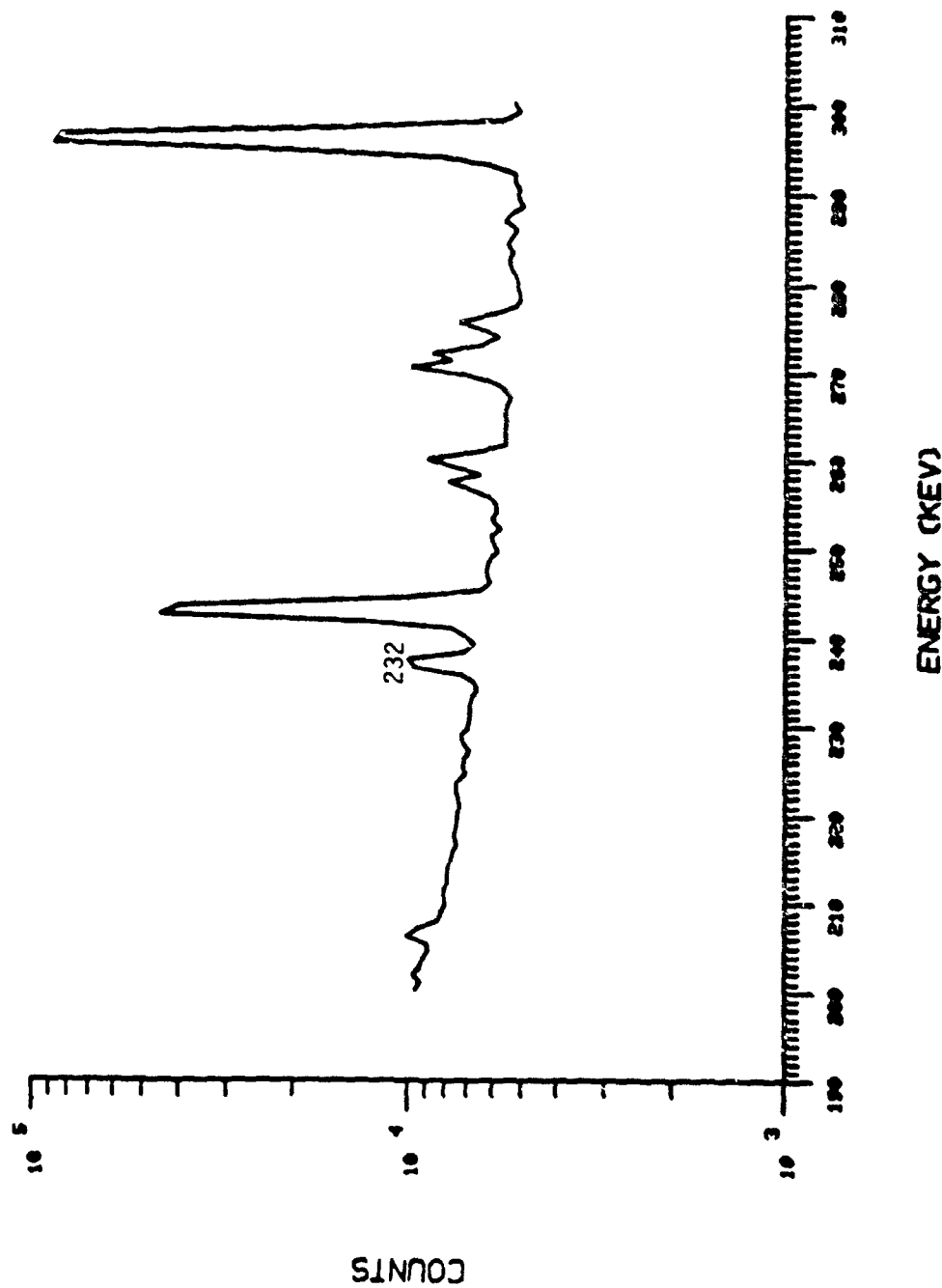
Figure 1. Soil Spectrum Low Energy
