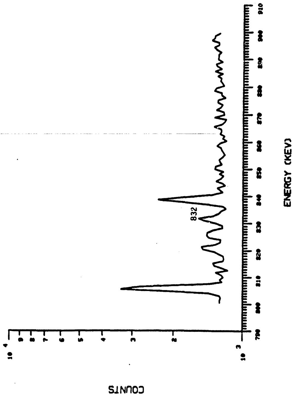
Figure 2. Soil Spectrum Middle Energy
