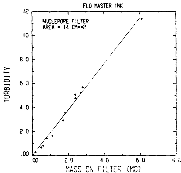
Fig. 8. Measurements of the turbidity of a Flo-Master ink aerosol collected on a 14 cm 2 Nuclepore filter vs the mass on the filter.
