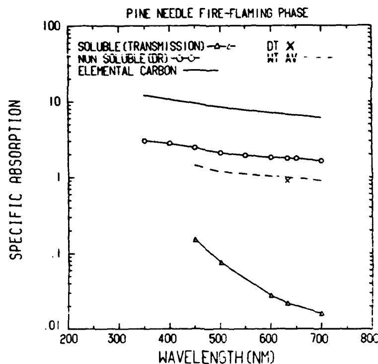
Fig. 10. Measurements of the absorption properties of smoke emissions from flaming combustion. The solid line with circles (-o-o-) represents the wavelength dependent B_s measured for the non-soluble component determined by diffuse reflectance. The lower solid line with triangles (-Δ-Δ-) represents the B_s measured for the soluble component by solution transmission. The dashed line represents a weighted average of the two components. The x represents a measurement made by the diffuse transmission technique for a total filter sample. The upper solid line is the B_s expected for a pure graphitic carbon aerosol.
