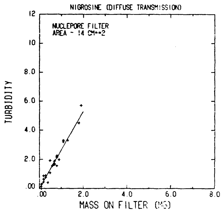
Fig. 7. Measurements of the turbidity of a Nigrosine aerosol collected on a 14 cm 2 Nuclepore filter vs the mass on the filter.
