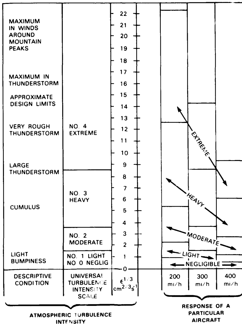
Figure IV-7. Turbulence scale suggested by MacCready 6 .
