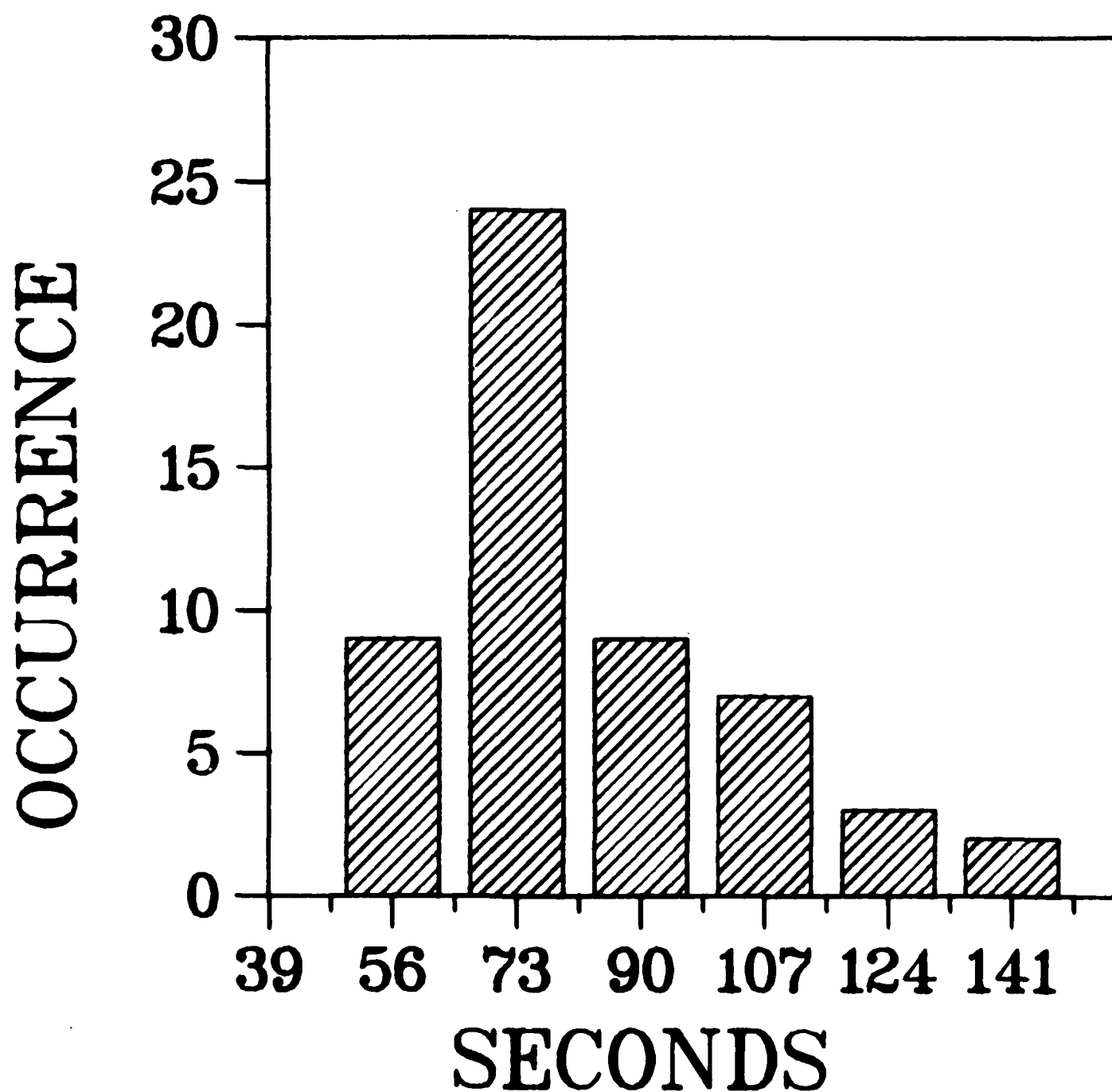
Figure 4. Rise times for mid-latitude Pi2s (after Samson et al. [1985]). The rise time is from the 1/e maximum to the maximum.
