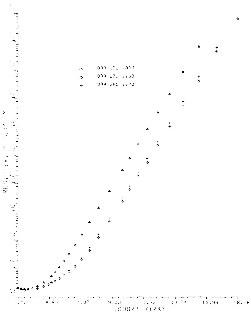
Figure 6. Comparison of Resistivity Data for Samples 1093 (Electron Irradiated), 1130 (As-Grown) and 1120 (As-Grown) Plotted Versus Reciprocal Temperature
