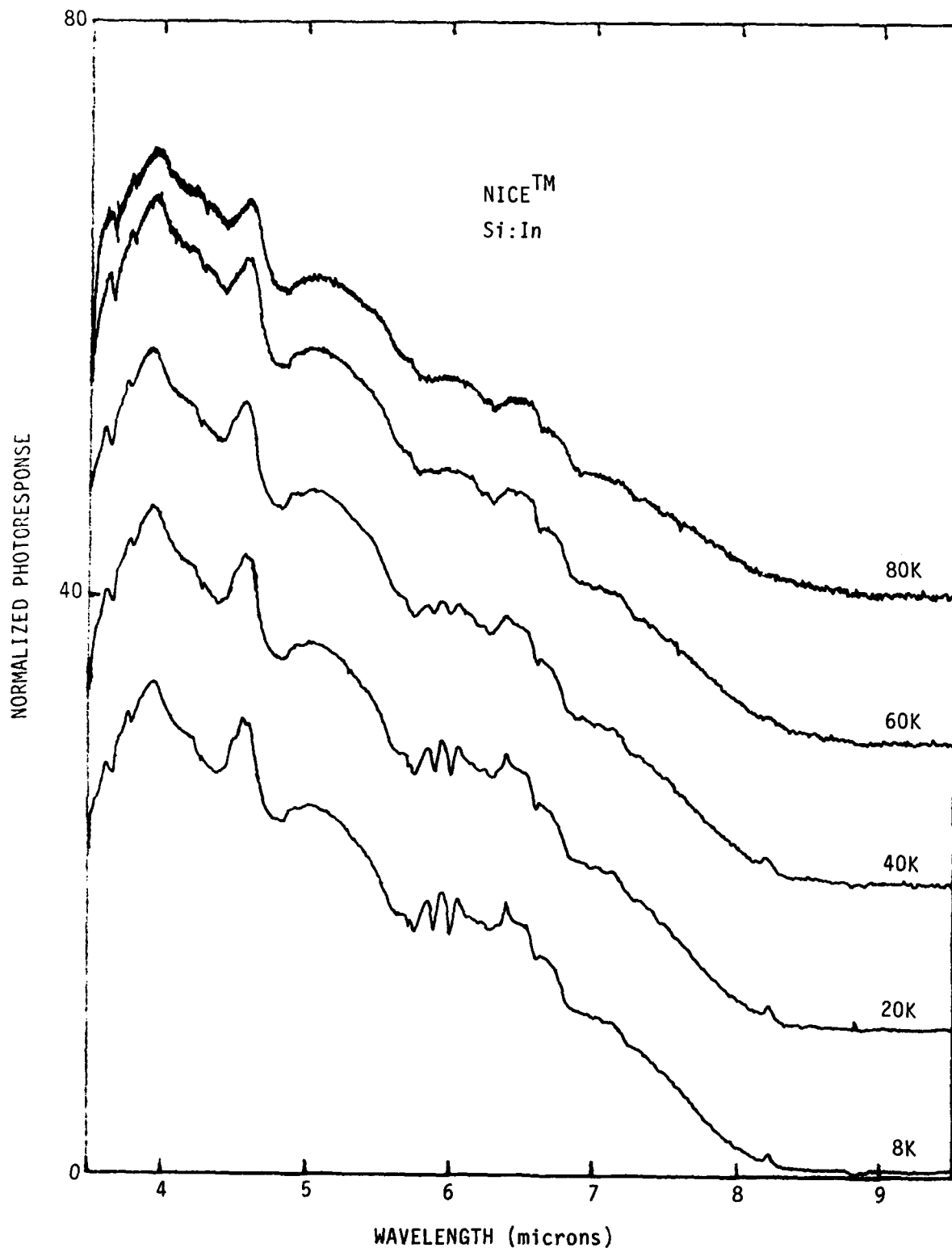
Figure 13. Normalized Photoresponse Versus Wavelength for Electron Irradiated Si:In Sample 0746 from 8K to 80K
