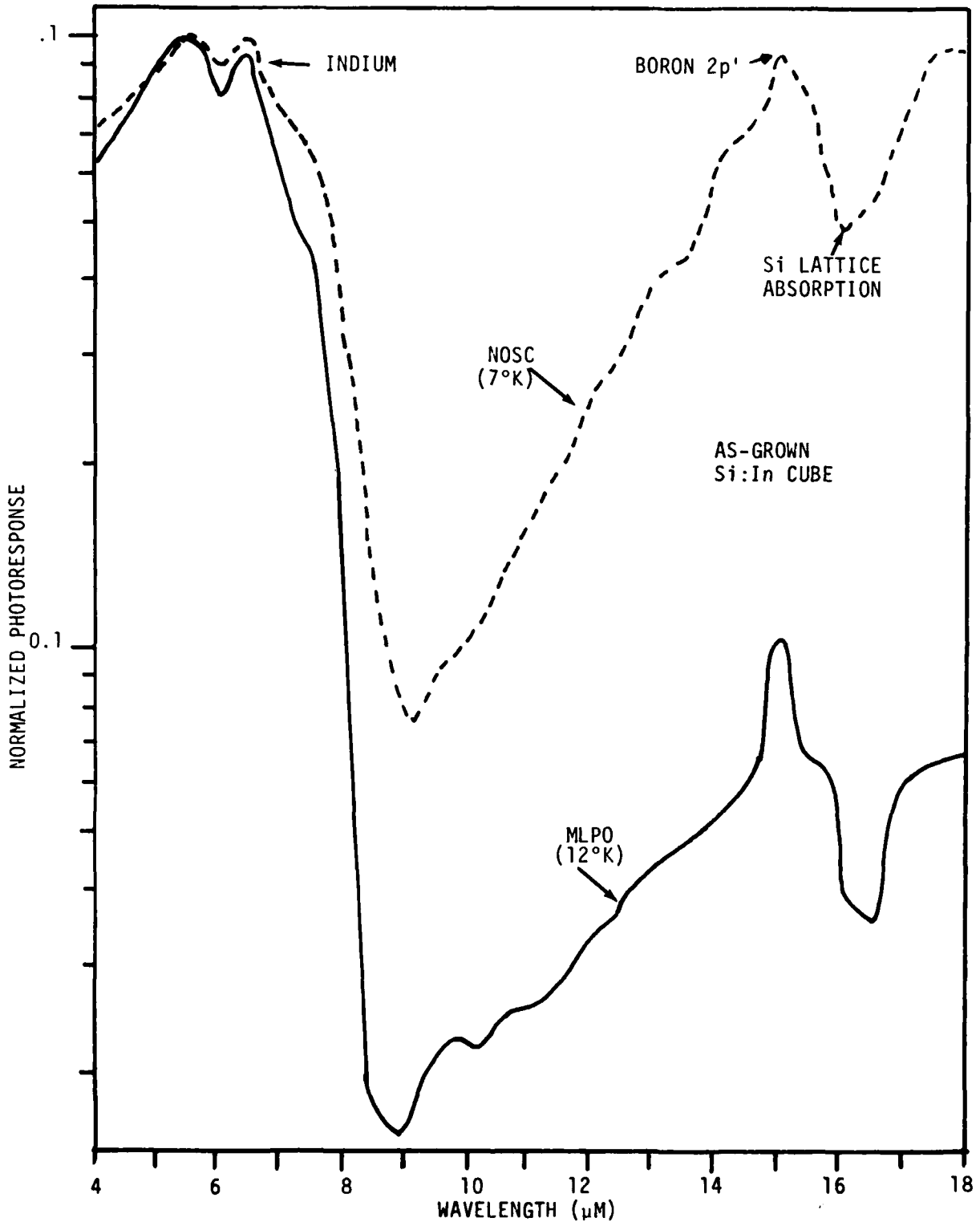
Figure 26. Comparison of NOSC and MLPO Measured Photoresponse of As-Grown Si:In Cube
