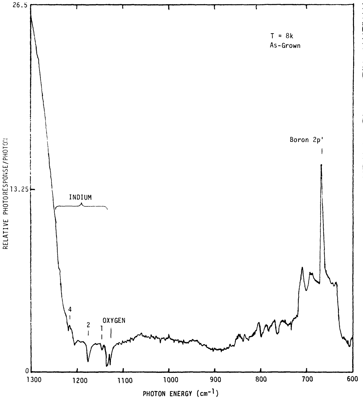
Figure 19. Photoconductivity Spectrum of As-Grown Si:In Sample 1043
