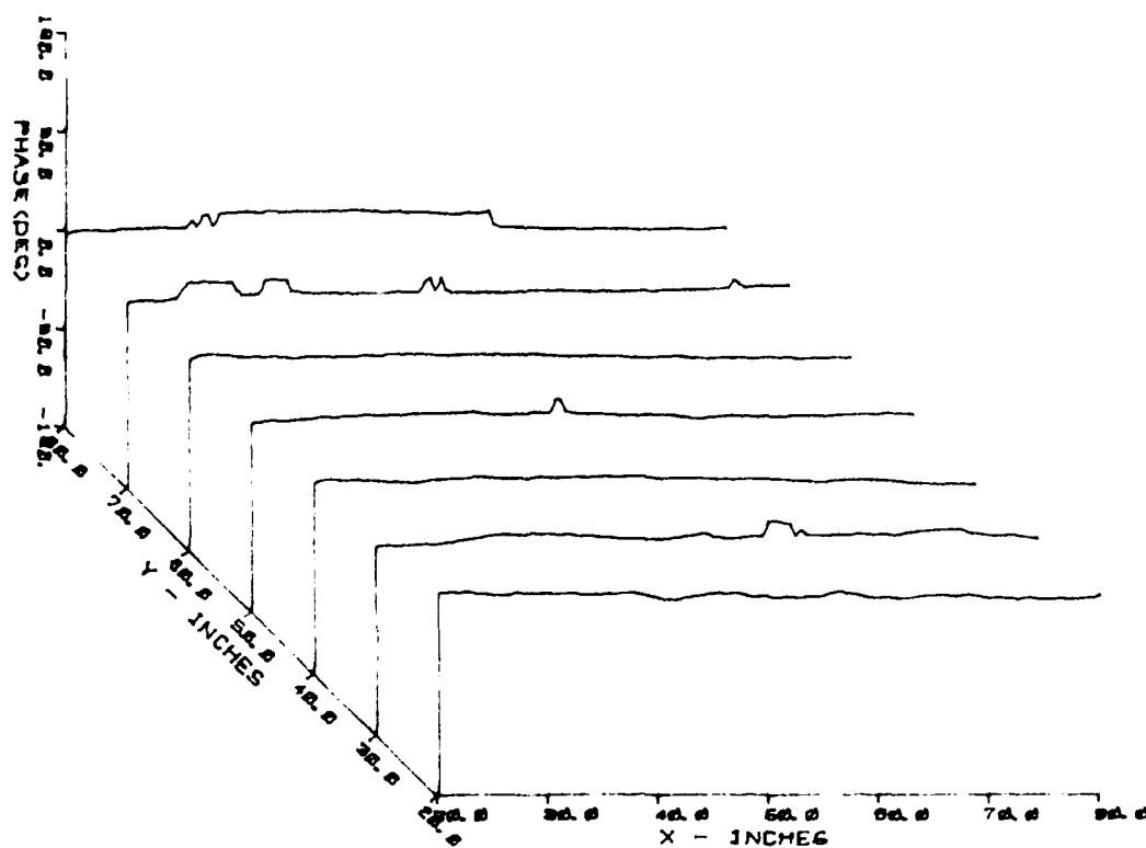
Figure A.59. 3D X-Plane Amplitude and Phase Field Probe Plot Taken at 18.0 GHz. H-Polarization, Using the Horn Probe
