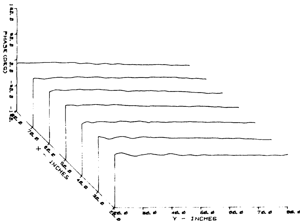
Figure A.36. 3D Y-Plane Amplitude and Phase Field Probe Plot Taken at 12.4 GHz, H-Polarization, Using the Horn Probe
