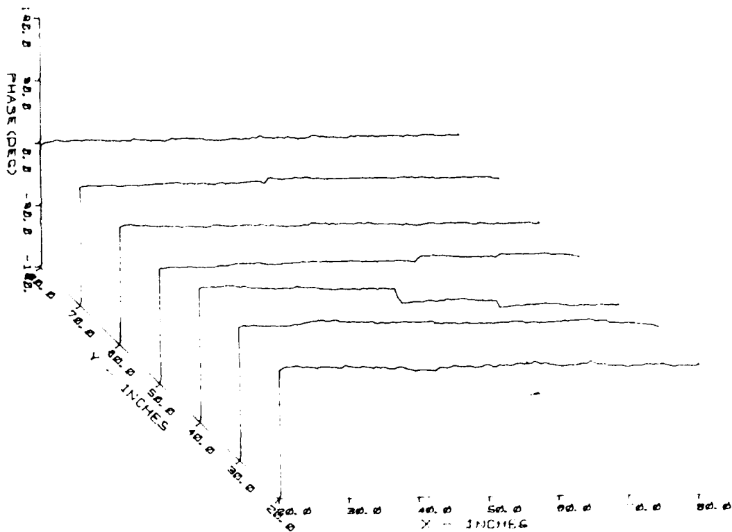
Figure A.47. 3D X-Plane Amplitude and Phase Field Probe Plot Taken at 18.0 GHz, H-Polarization, Using the Horn Probe
