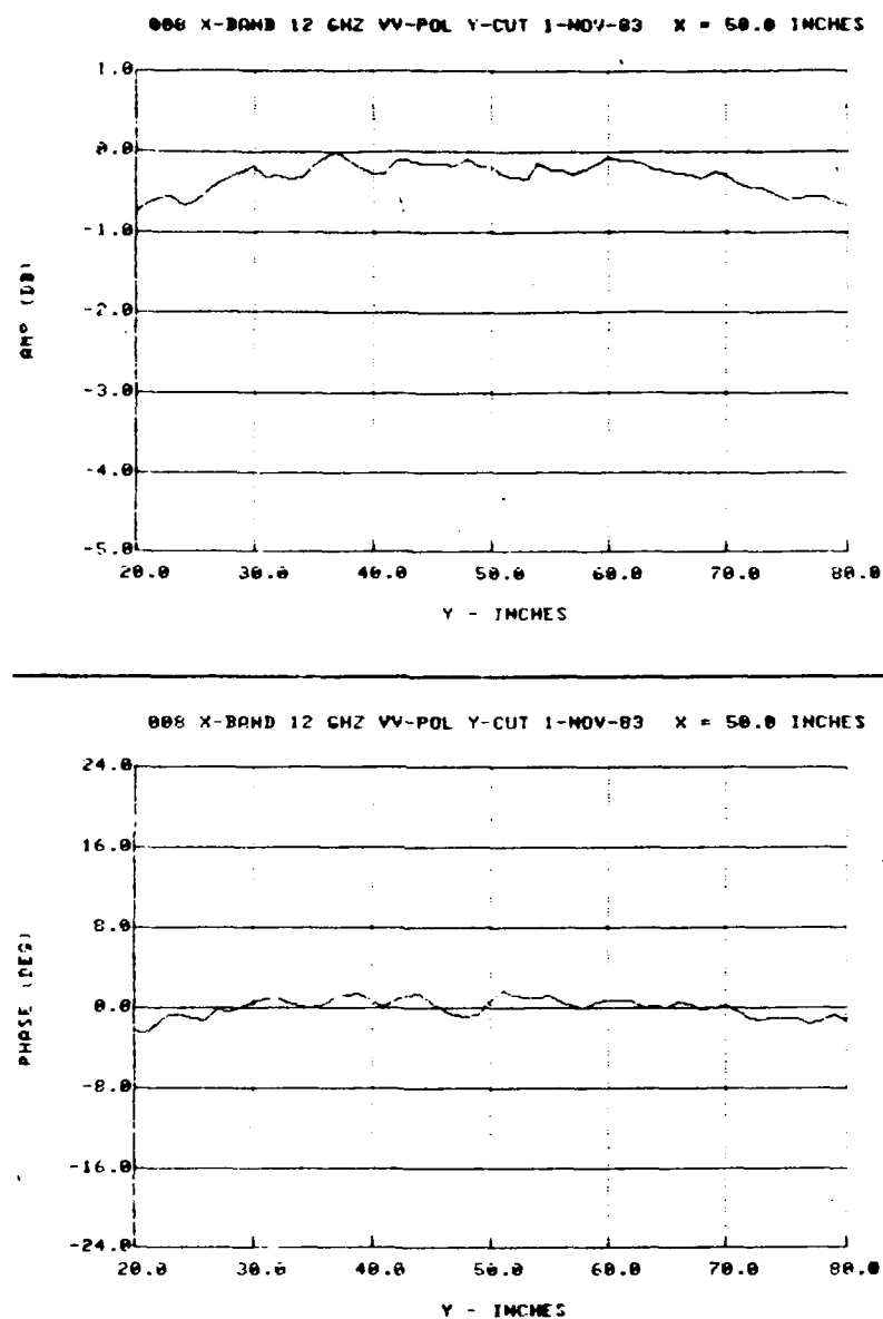
Figure 17. Y-Plane Amplitude and Phase Field Probe Plot Taken at 12.0 GHz, V-Polarization, Using the Horn Probe
