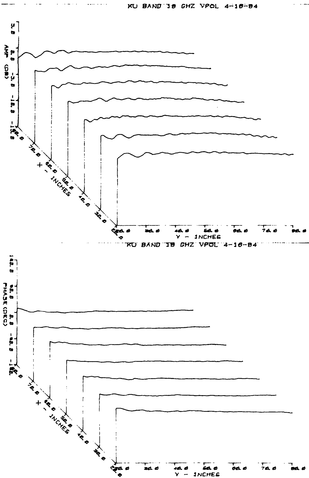
Figure A.42. 3D Y-P'ane Amplitude and Phase Field Probe Plot Taken at 18.0 GHz, V-Polarization, Using the Horn Probe
