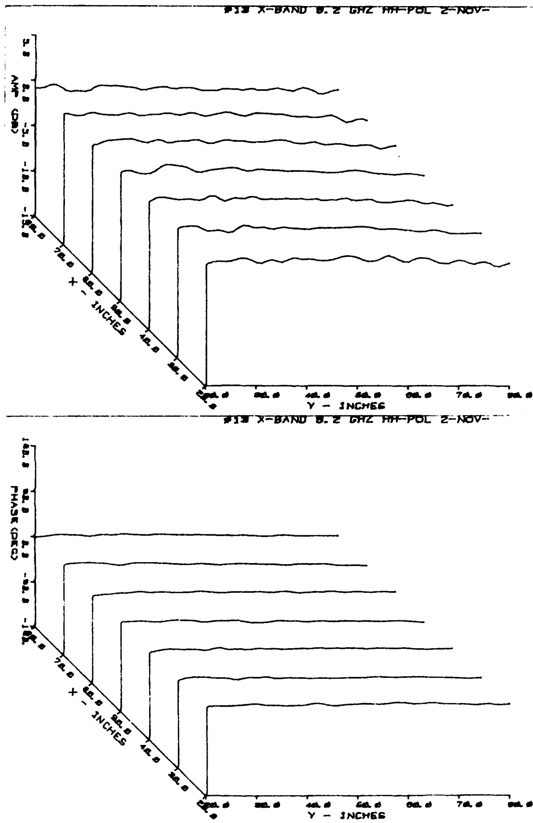
Figure A.12. 3D Y-Plane Amplitude and Phase Field Probe Plot Taken at 8.2 GHz, H-Polarization, Using the Horn Probe
