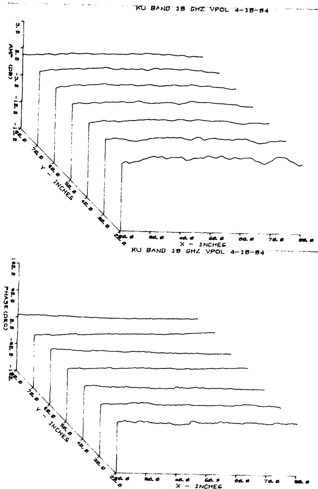
Figure A.41. 3D X-Plane Amplitude and Phase Field Probe Plot Taken at 18.0 GHz, V-Polarization, Using the Horn Probe
