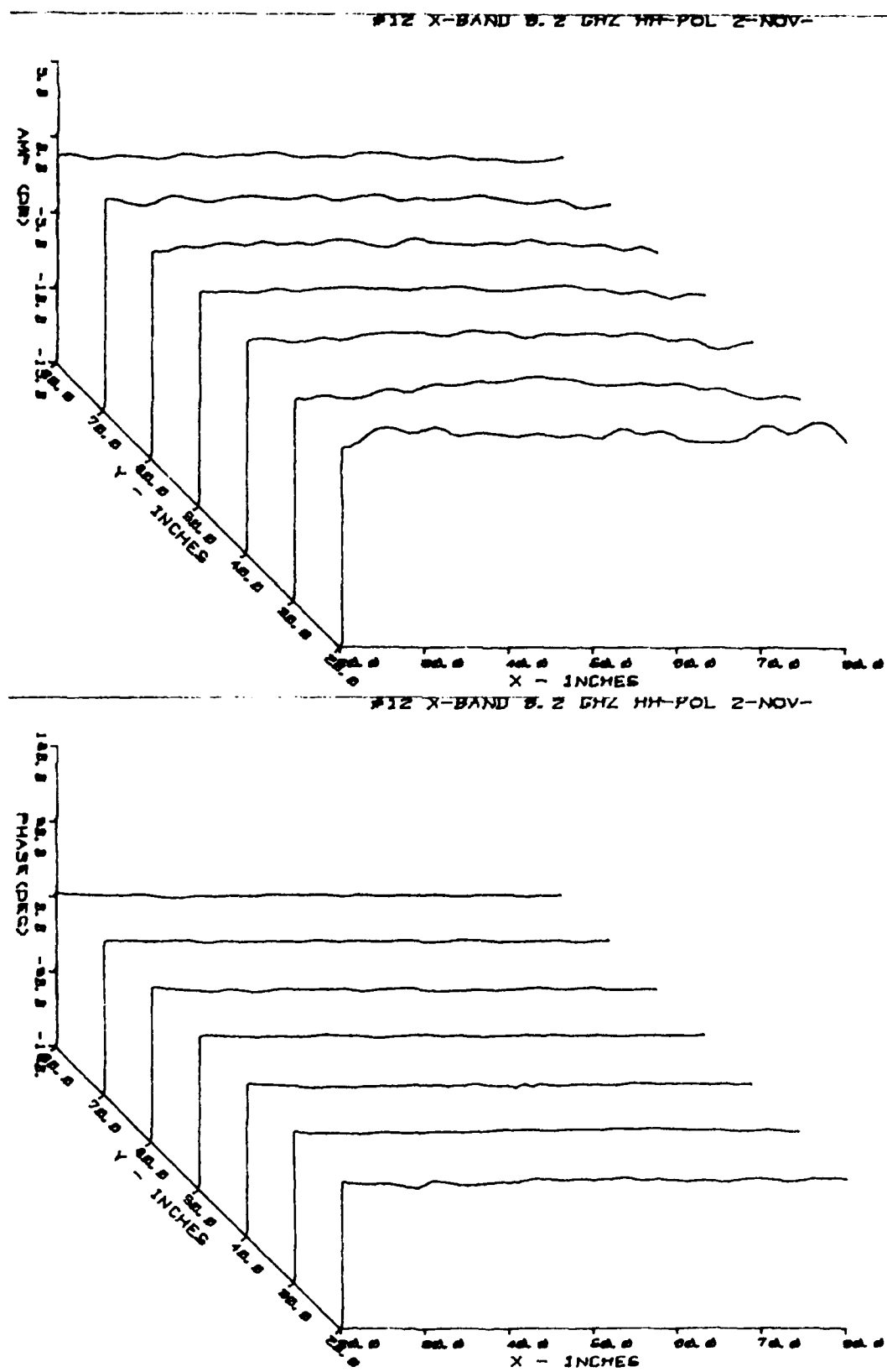
Figure A.11. 3D X-Plane Amplitude and Phase Field Probe Plot Taken at 8.2 GHz, H-Polarization, Using the Horn Probe
