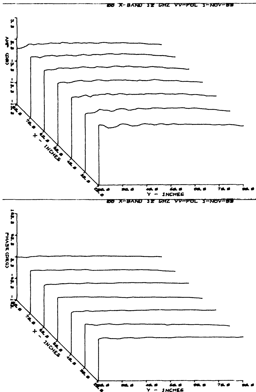
Figure A.18. 3D Y-Plane Amplitude and Phase Field Probe Plot Taken at 12.0 GHz, V-Polarization, Using the Horn Probe
