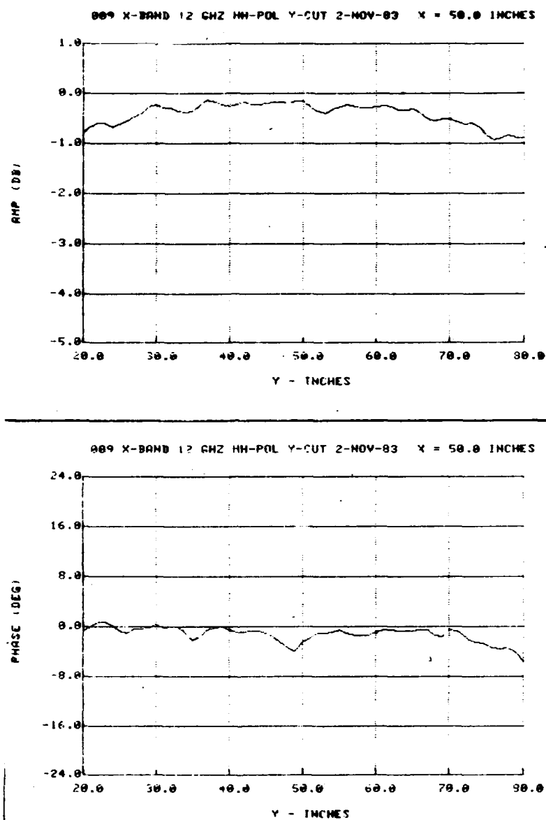
Figure A.20. Y-Plane Amplitude and Phase Field Probe Plot Taken at 12.0 GHz, H-Polarization, Using the Horn Probe
