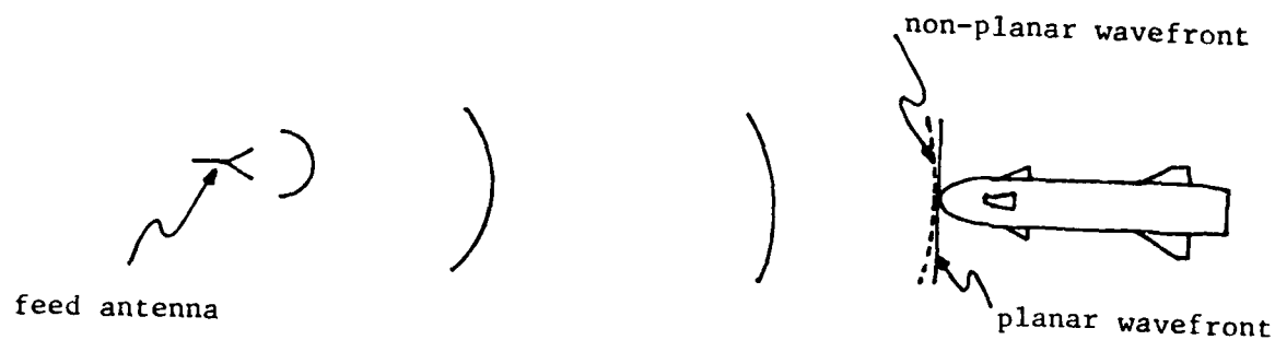
Figure 1. Planewave Approximation to Diverging Spherical Wavefront (Far Field)
