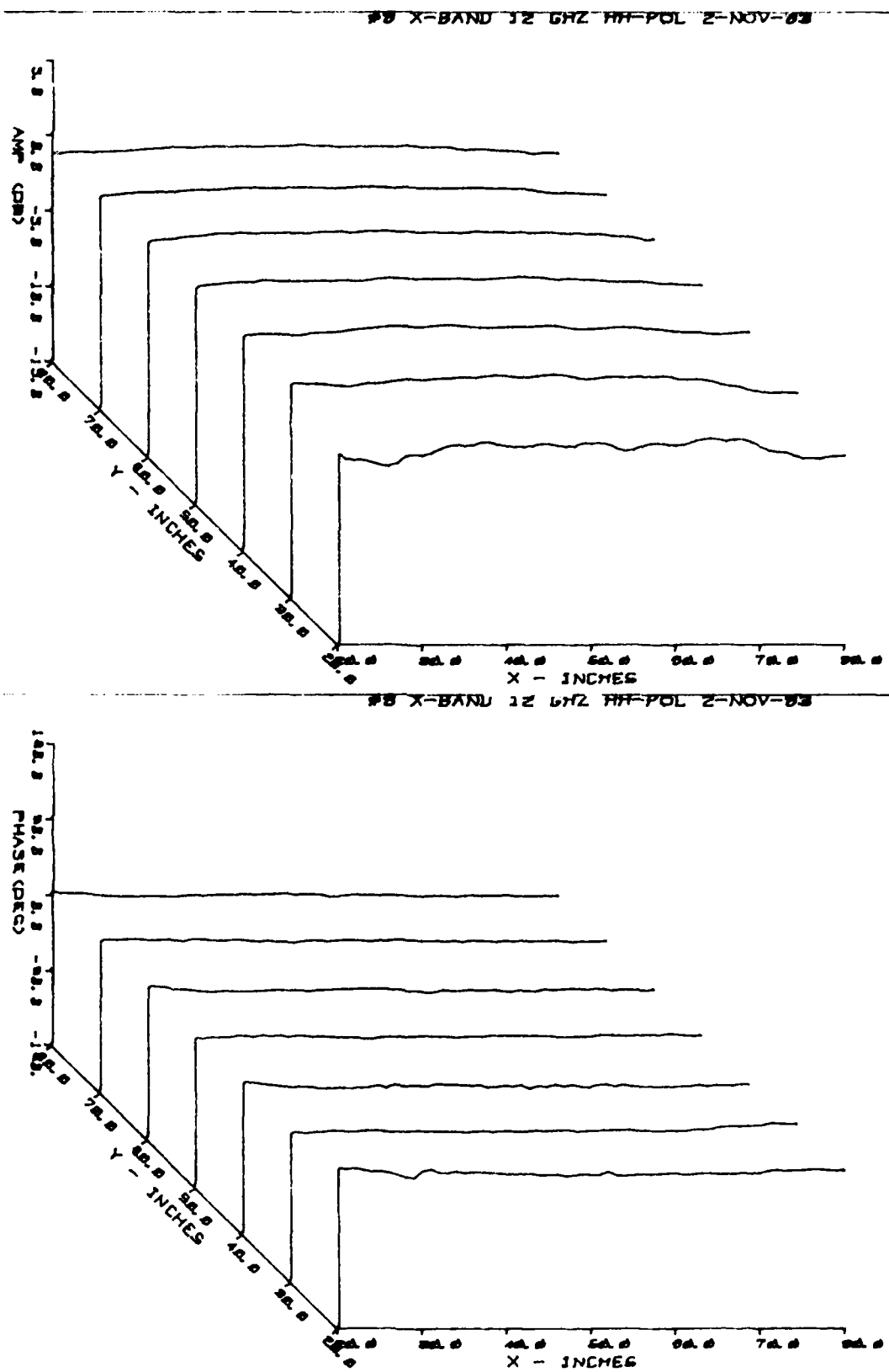
Figure A.23. 3D X-Plane Amplitude and Phase Field Probe Plot Taken at 12.0 GHz, H-Polarization, Using the Horn Probe
