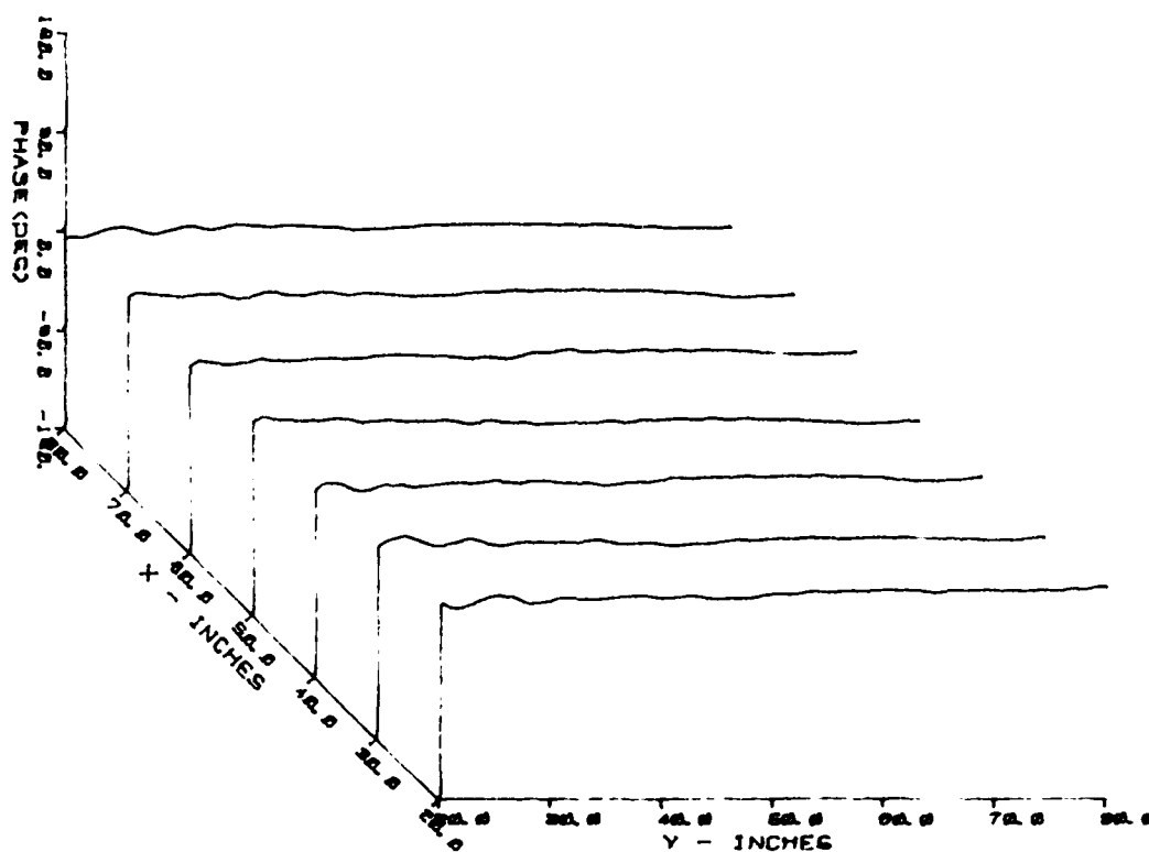
Figure A.54. 3D Y-Plane Amplitude and Phase Field Probe Plot Taken at 18.0 GHz, V-Polarization, Using the Horn Probe
