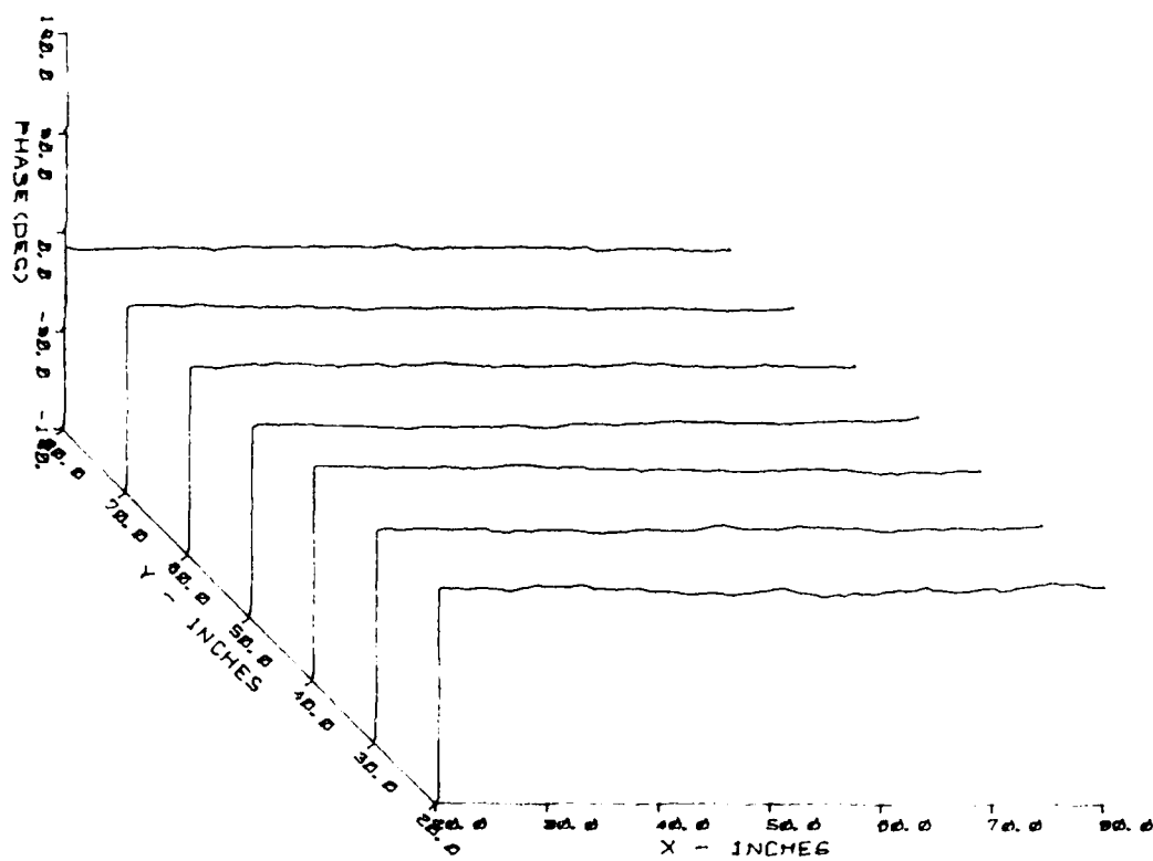
Figure A.35. 3D X-Plane Amplitude and Phase Field Probe Plot Taken at 12.4 GHz, H-Polarization, Using the Horn Probe
