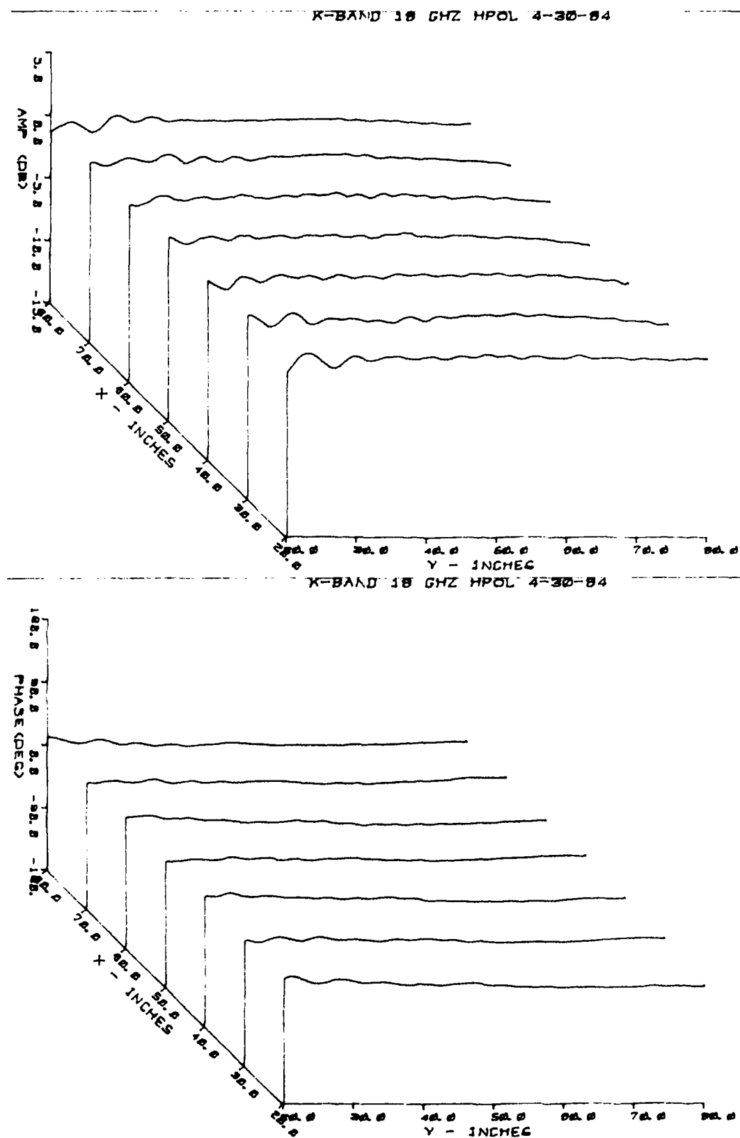
Figure A.60. 3D X-Plane Amplitude and Phase Field Probe Plot Taken at 18.0 GHz, H-Polarization, Using the Horn Probe
