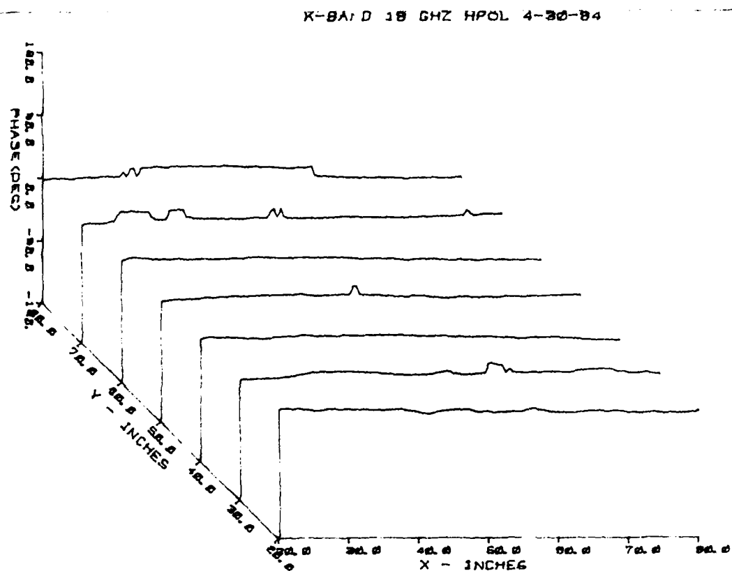
Figure 29. 3D X-Plane Phase Field Probe Plot Taken at 18.0 GHz, H-Polarization, Using the Horn Probe (Note Phase Discontinuities)
