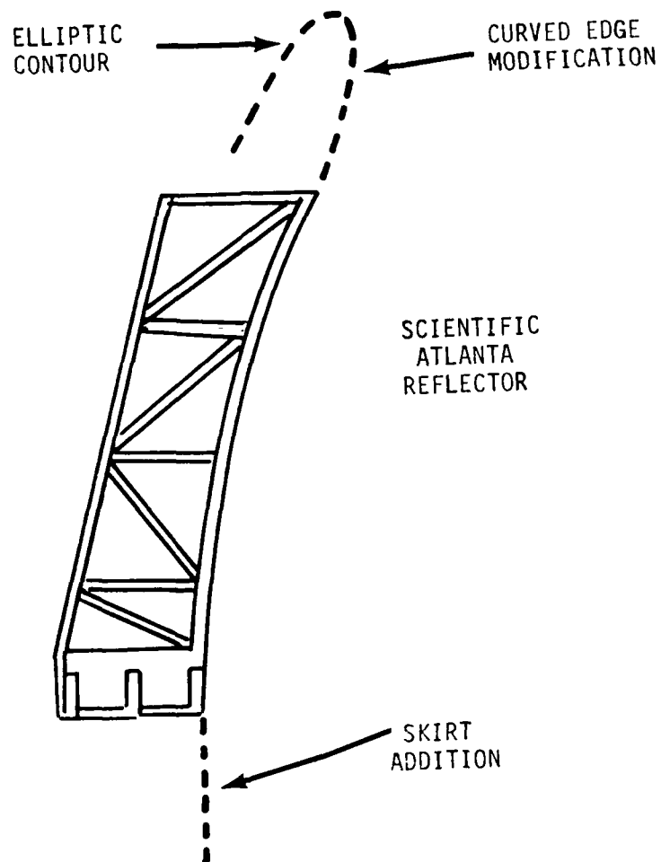
Figure 30. Side View of Elliptical Curved Edge Treatments for the OSU and NASA Compact Range Reflector Antenna
