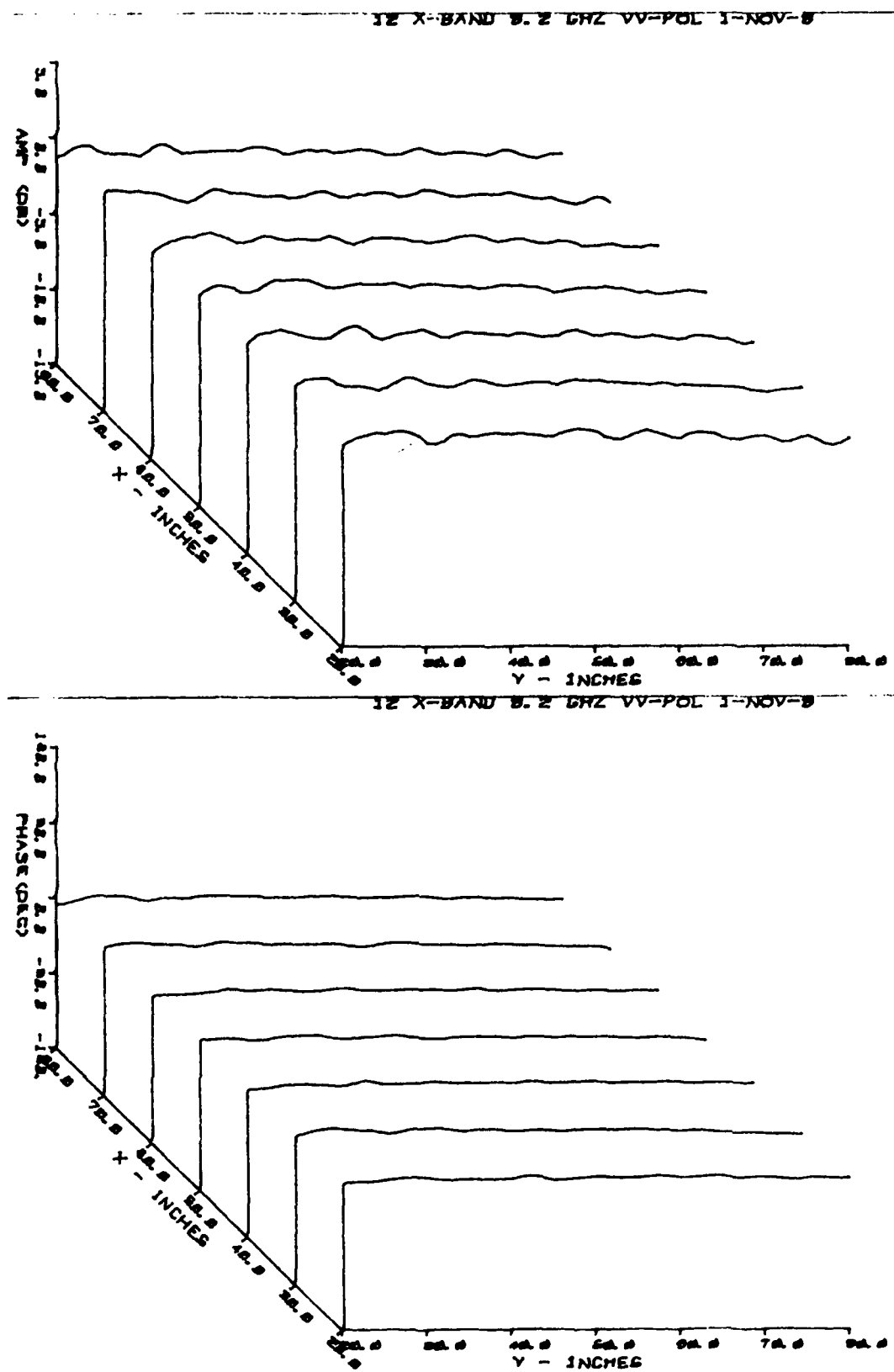
Figure A.6. 3D Y-Plane Amplitude and Phase Field Probe Plot Taken at 8.2 GHz, V-Polarization, Using the Horn Probe
