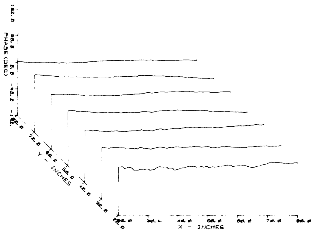
Figure A.63. 3D X-Plane Amplitude and Phase Field Probe Plot Taken at 26.0 GHz, V-Polarization, Using the Horn Probe
