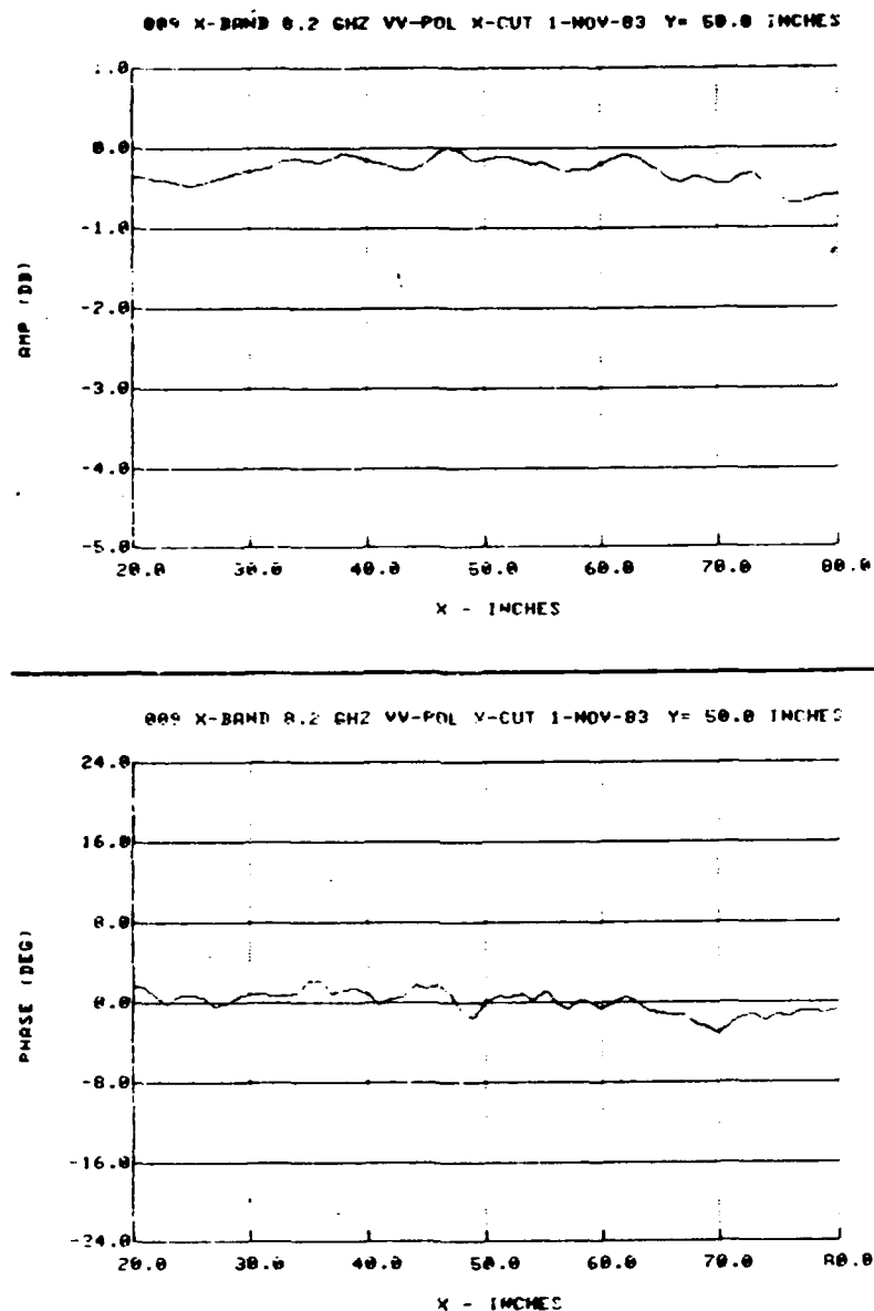
Figure 27. X-Plane Amplitude and Phase Field Probe Plot Taken at 8.2 GHz, V-Polarization, Using the Horn Probe
