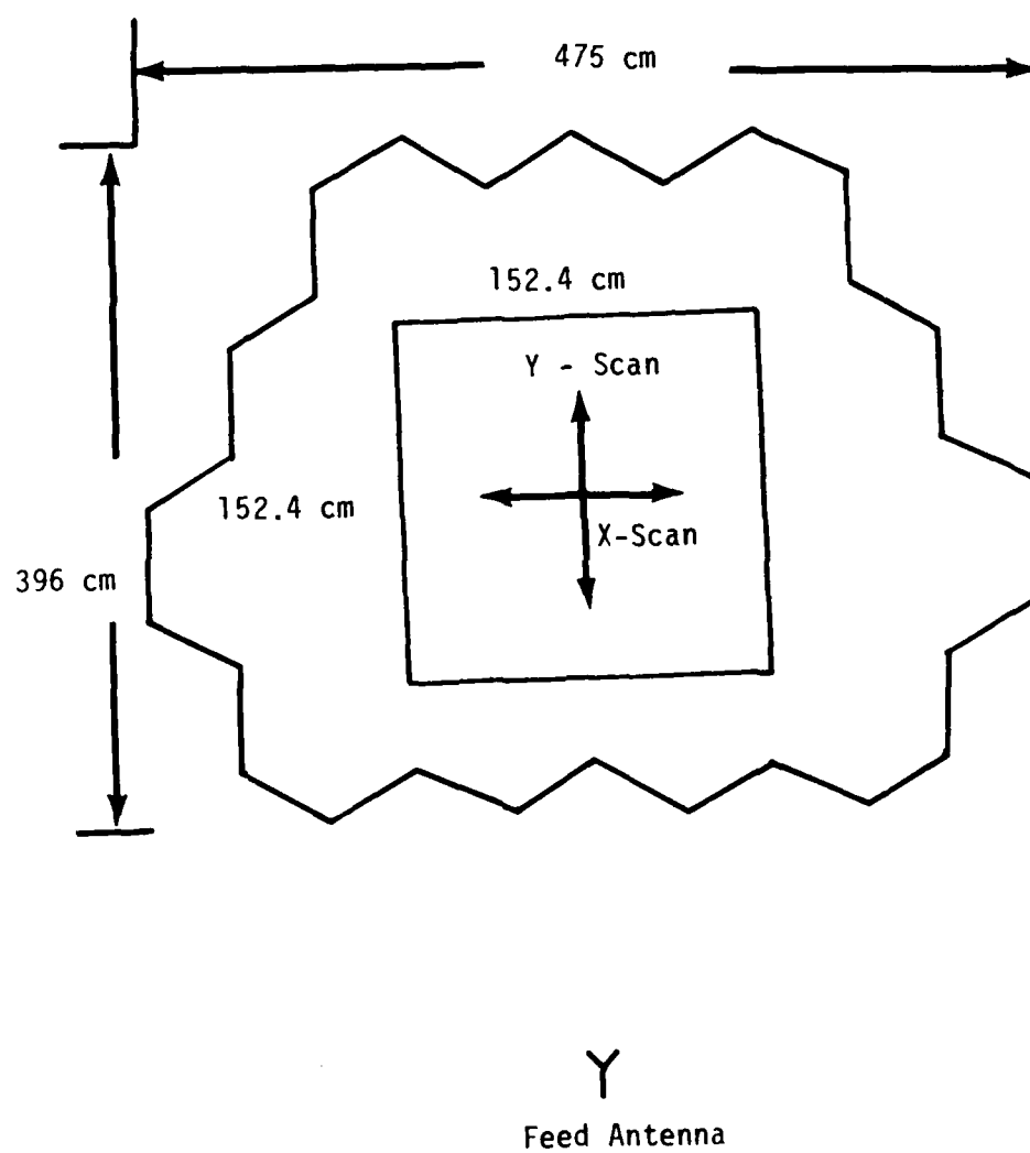
Figure 14. Principle Plane Measurements as Seen by the Field Probe
