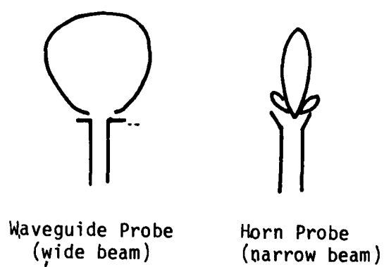
Figure 22. Radiation Patterns for the Selected Horn Probe (Right) and Waveguide Probe (Left)
