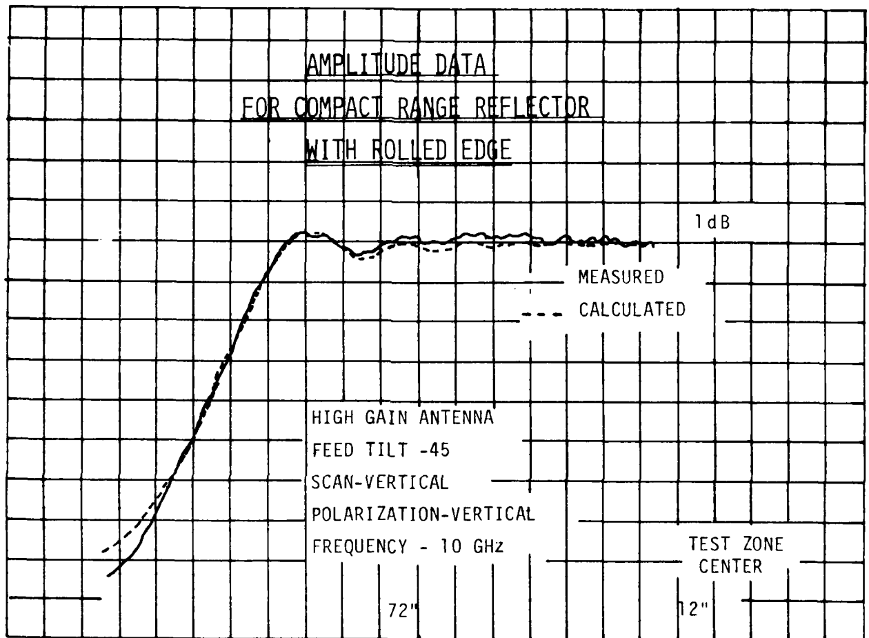
Figure 32. Amplitude Field Probe Taken Across a Modified Curved Edge Treatment (Measurements Compared to Moment Method Calculations at 10. GHz)
