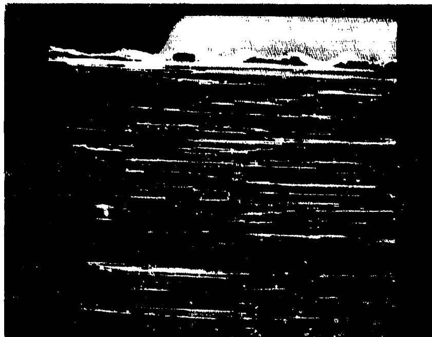
Figure 38. Fracture Surface of the 90° Flexural Specimen After the Fourth Paint Removal at 60 psi. MAG: 50X
