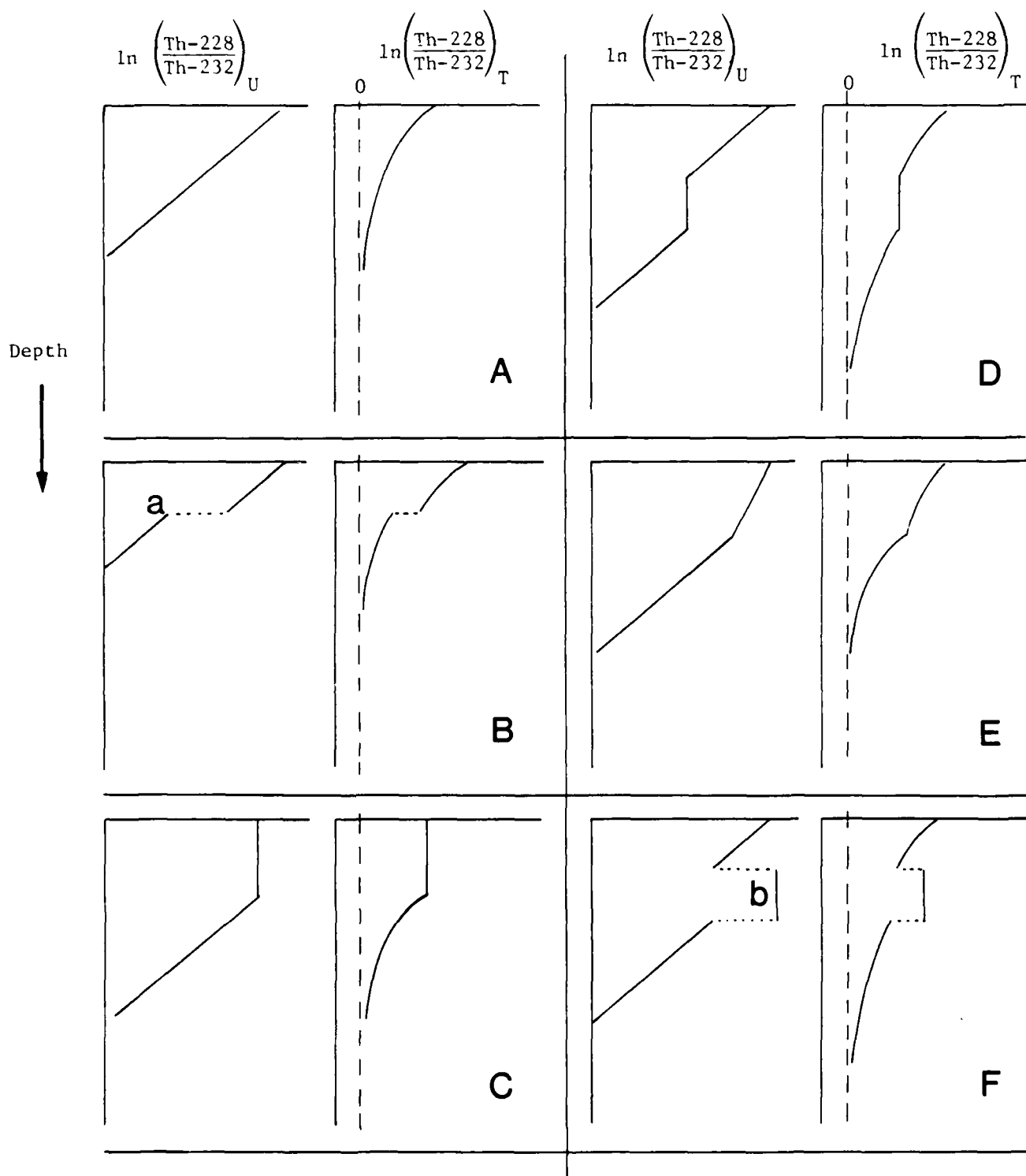
Figure 9. The effects of some sedimentary processes on the idealized depth profile of total Th-228/Th-232 ( (\text{Th-228/Th-232})_T ) and unsupported Th-228/Th-232 ( (\text{Th-228/Th-232})_U ). A) Particle-by-particle deposition. B) Particle-by-particle deposition disrupted by erosional event (point a). C) Homogenization of surface sediment by physical or biological mixing. D) Particle-by-particle deposition disrupted by slumping. E) Change in sedimentation rate. F) Particle-by-particle deposition disrupted by rapid deposition from a different source of material.
