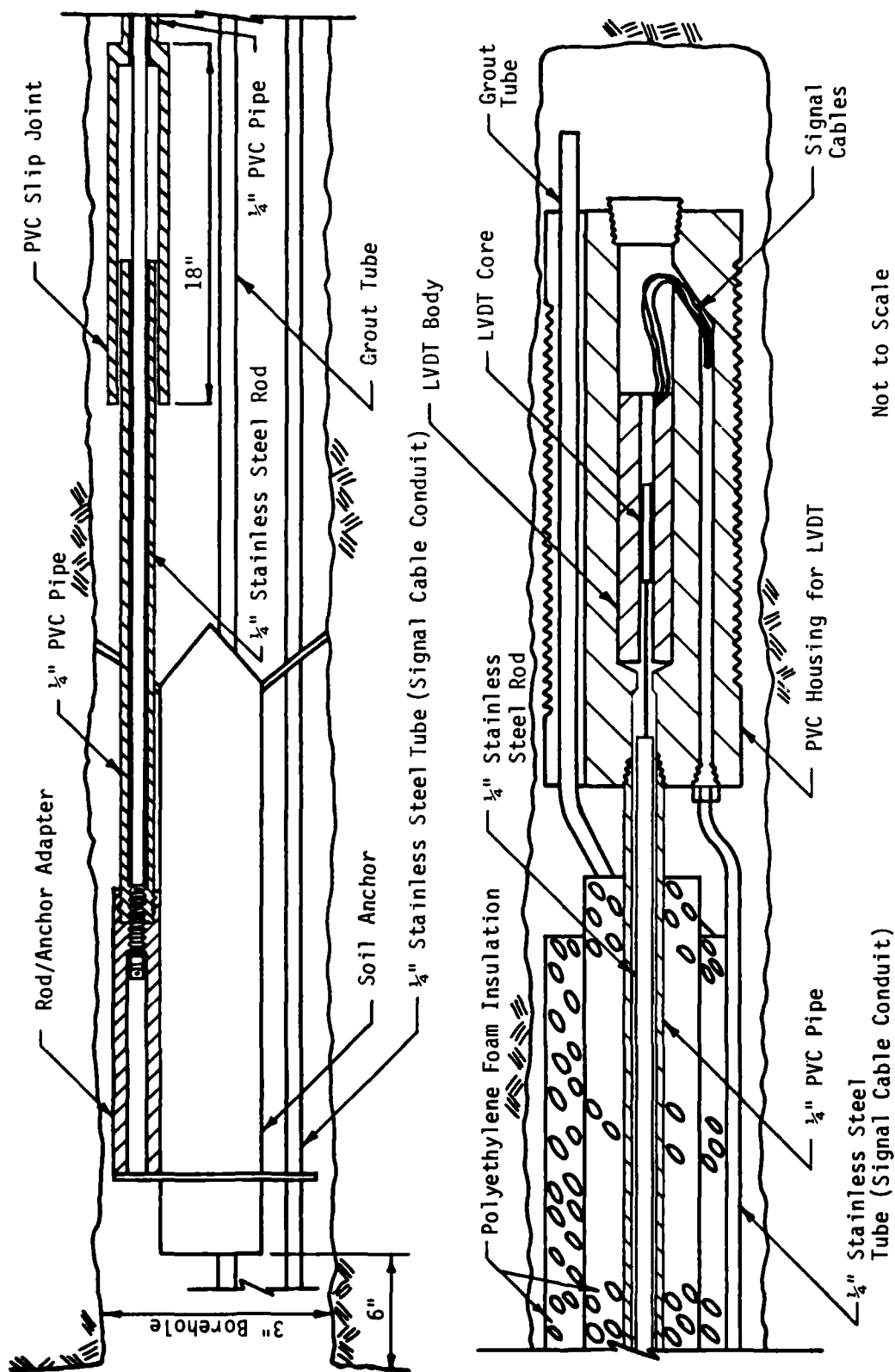
Figure 3-2. Dynamic relative displacement gage configured with transducer at far end of borehole.
