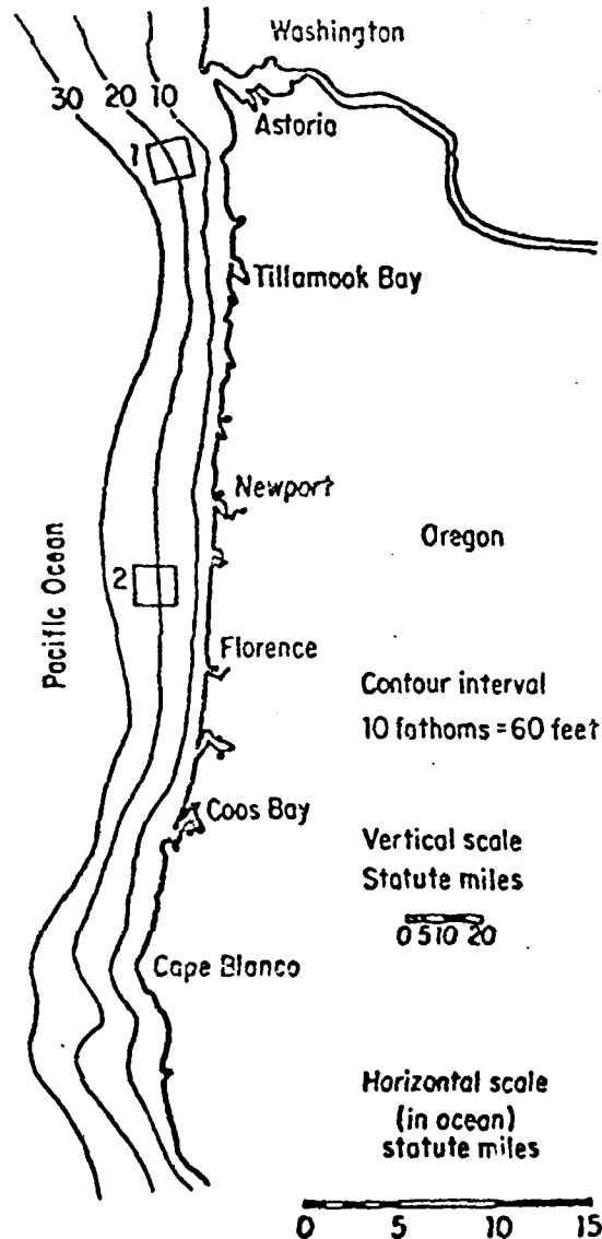
FIG. 1. The Oregon coast and the depth of offshore waters. Note the expansion of the horizontal scale relative to the vertical scale.
