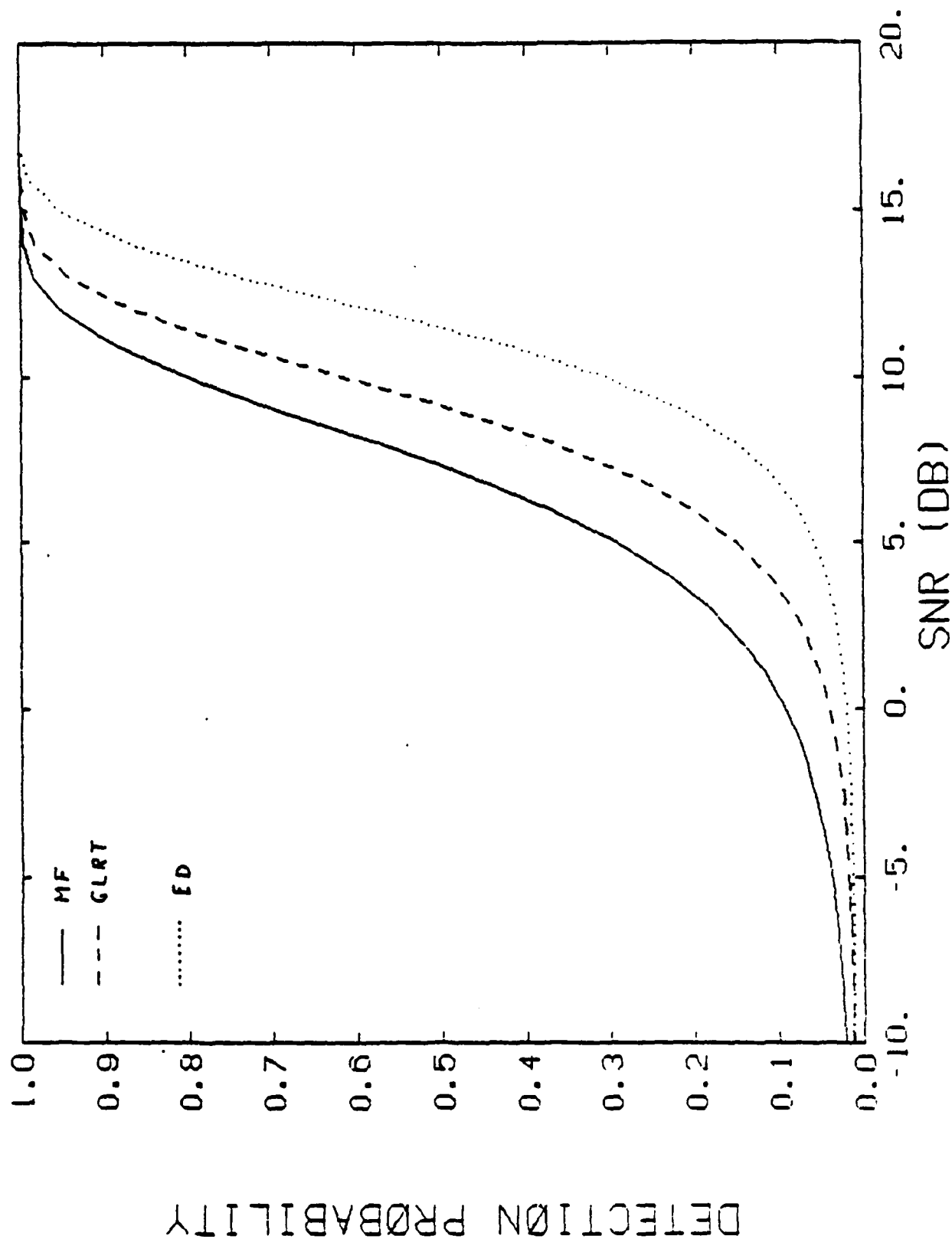
Figure 3. Performance Curves for Medium Band Signal, P_{FA} = 10^{-2} , N = 10
