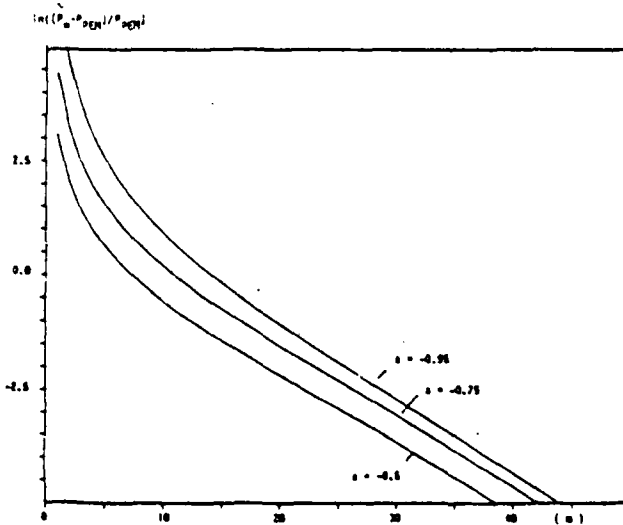
Fig. 2. The convergence of \hat{P}_m , c = -0.9 , varying a .
