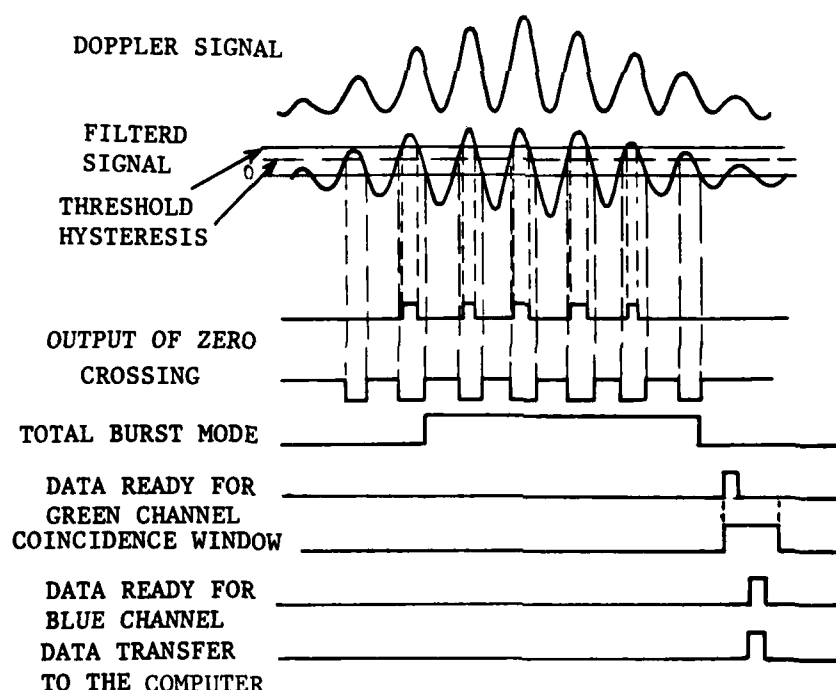
Fig. D-1 Valid burst processing and coincidence window operation.
