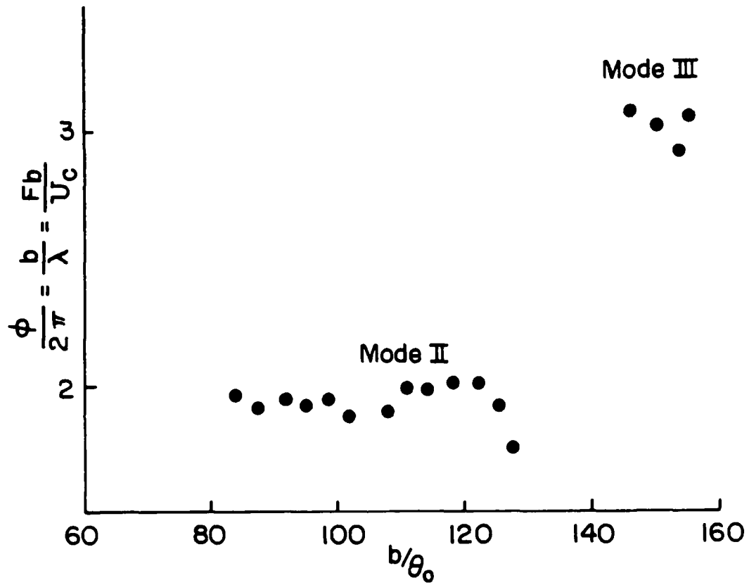
Fig. 12 Overall phase difference between two corners of the cavity for Modes II and III of the cavity flow oscillations.
