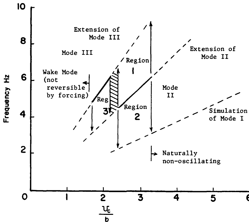
Fig. 67 Possible interactions with the cavity flow through external forcing
