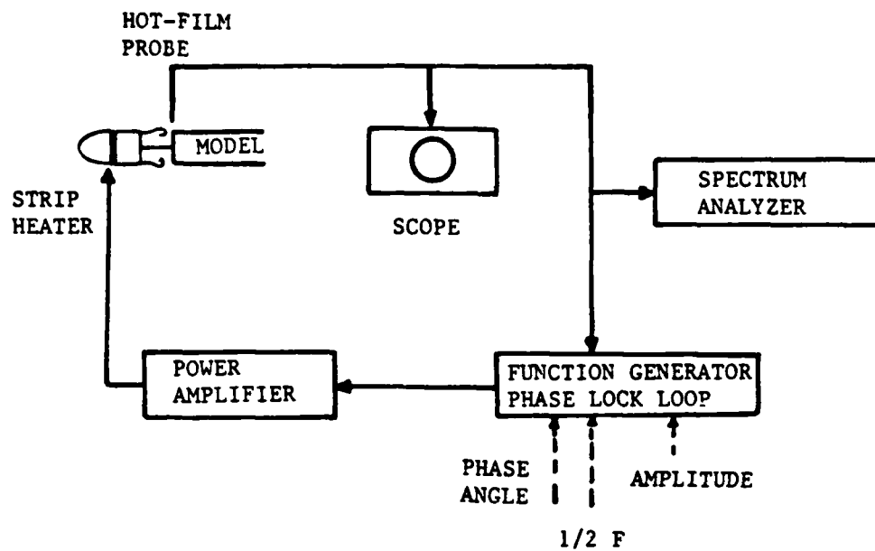
Fig. 68 Schematic of the cancellation set-up.
