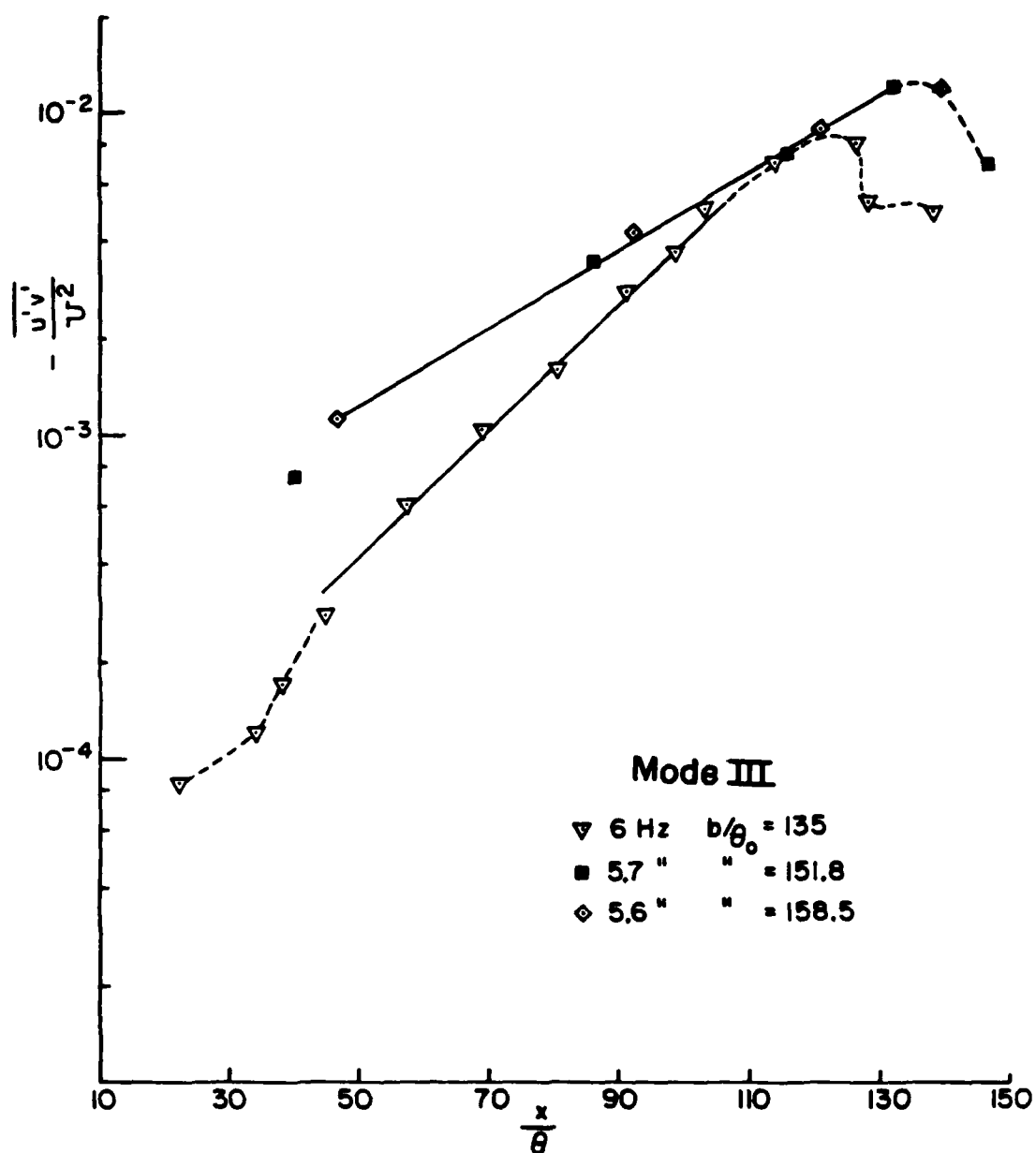
Fig. 30 Growth of the maximum shear stress in the cavity shear layer with downstream distance; Mode III, \frac{Fb}{U_c} \approx 3 .
