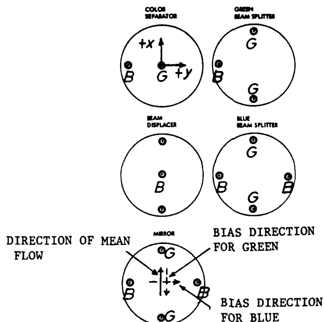
Fig. B-1 Measuring volume formation.
