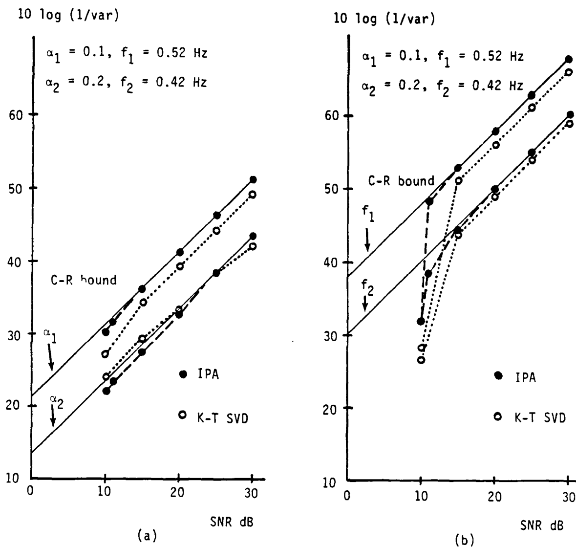
Figure 5. (a),(b) Comparison of pole estimators.
