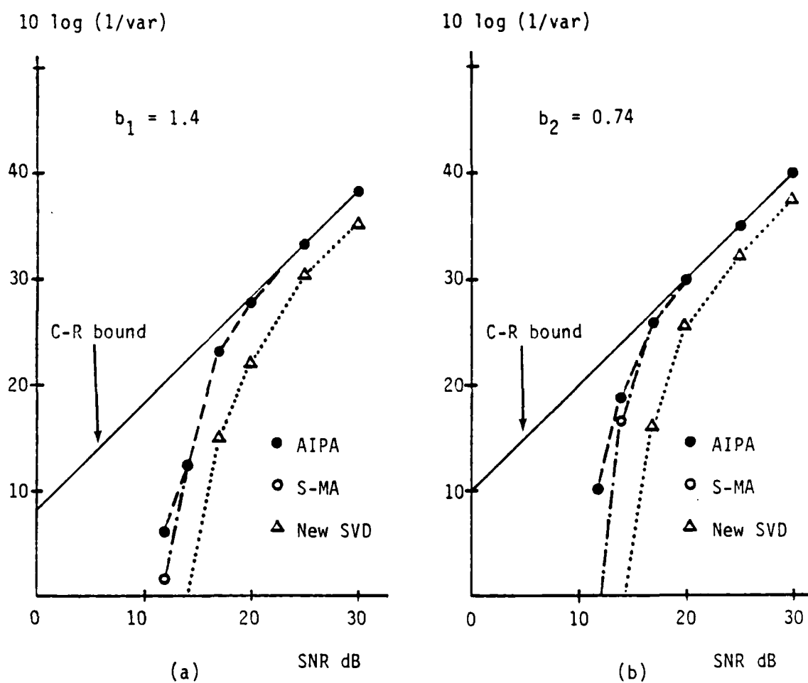
Figure 2. (a),(b) Comparison of pole estimators. (b_1 = 1.4, b_2 = 0.74)
