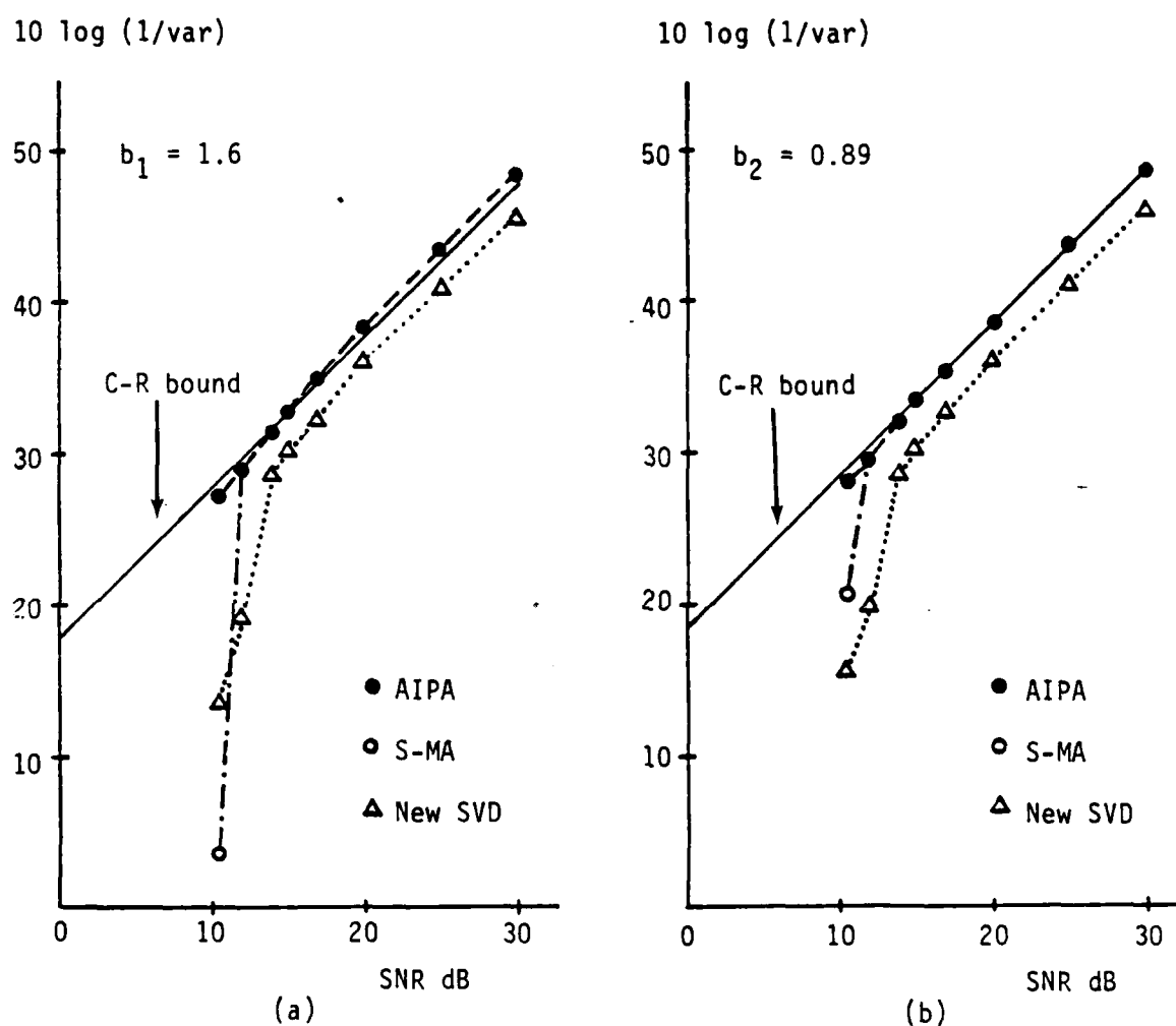
Figure 1. (a),(b) Comparison of pole estimators. (b_1 = 1.6, b_2 = 0.89)
