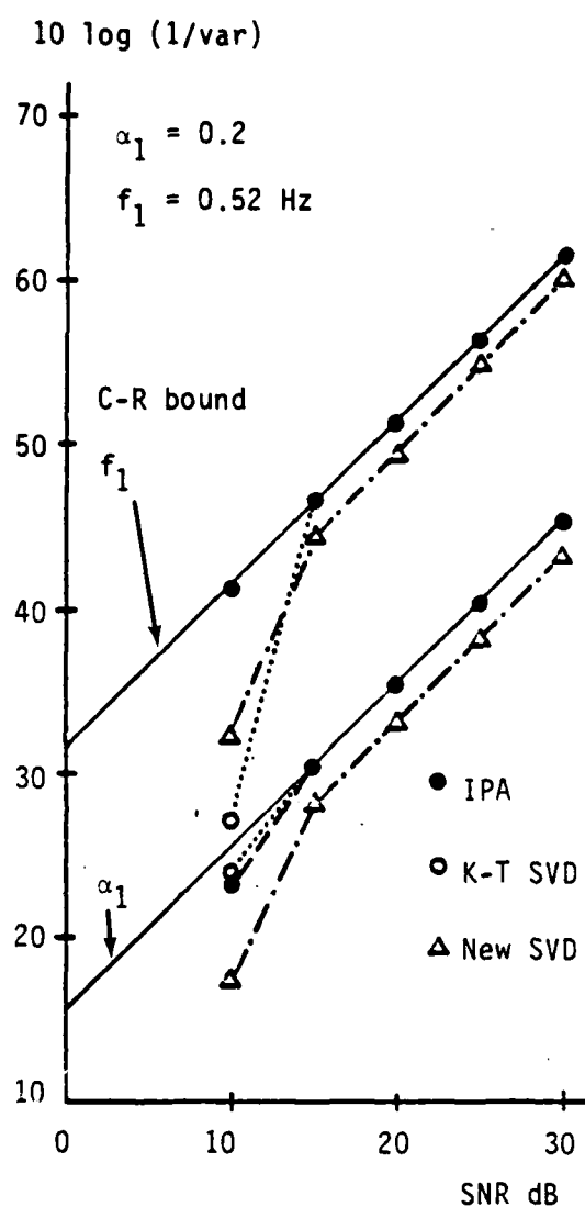
Figure 4. Comparison of pole estimators.
