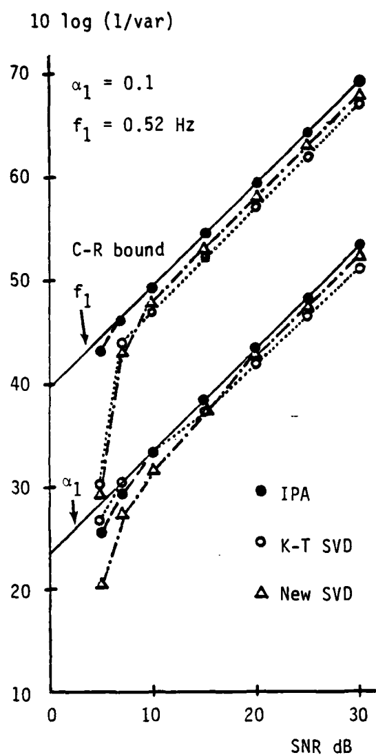
Figure 3. Comparison of pole estimators.
