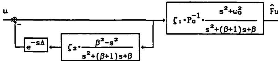
Figure 3. Realization of Optimal Compensator
