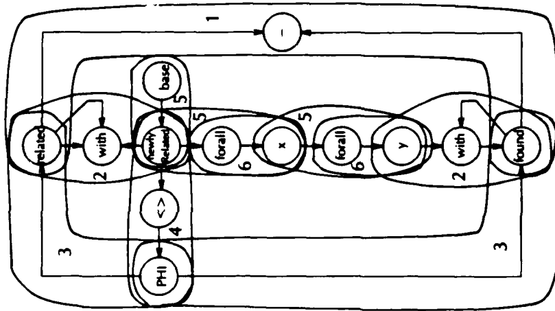
Figure 2.5 Matched data flow graph of sample program
