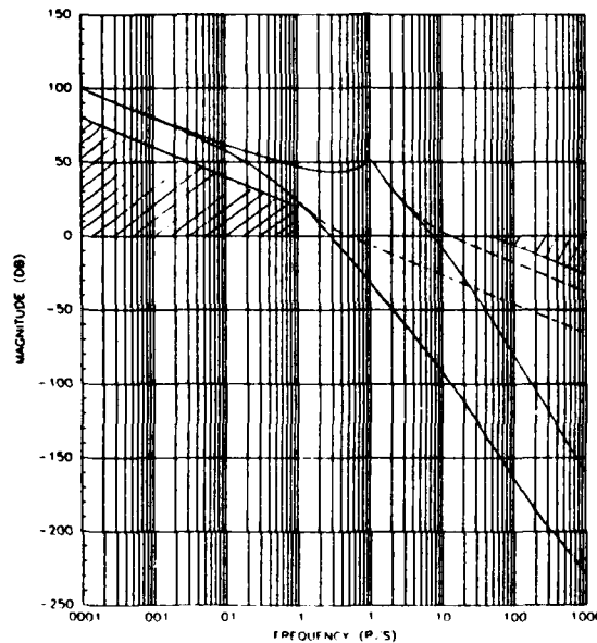
Fig 13.13 Singular Values of T_{FOL} and T_{KF} , Low Matching
