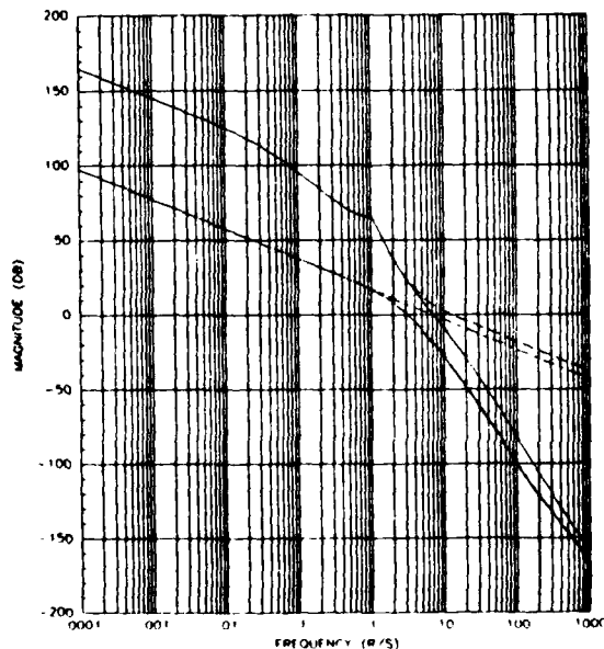
Fig 13.20 Singular Values of T_{FOL} and T_{KF} , \Gamma = R , \mu = 0.2
