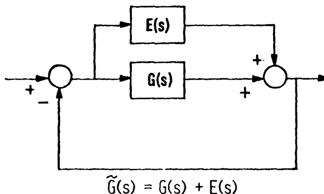
FIG. 1 ADDITIVE PERTURBATION
