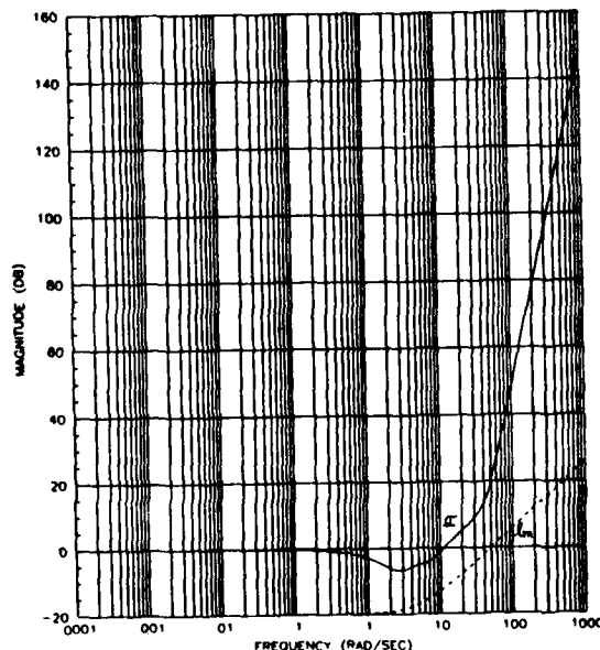
Fig 13.47 Singular Values of \ell_m and \sigma[J + (KG)^{-1}]
