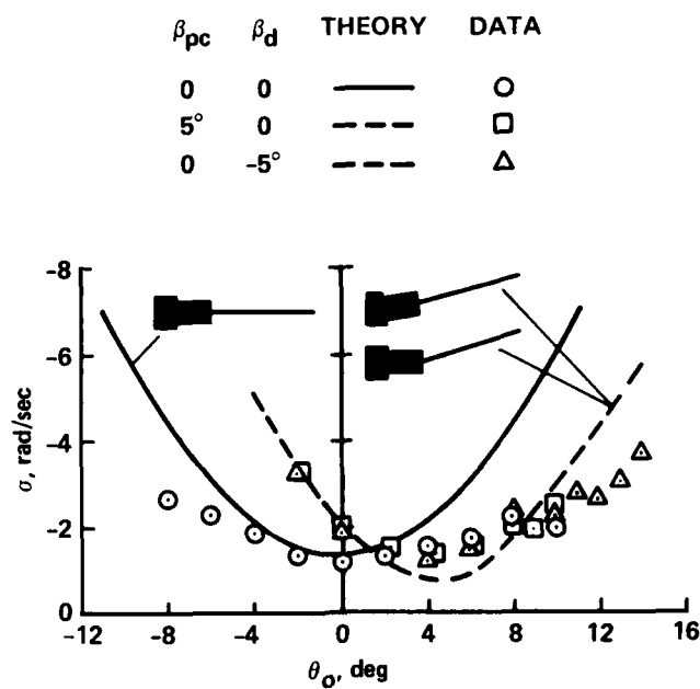
Figure 15.— Effect of precone and droop on lead-lag damping variation with pitch angle, stiff pitch flexure.
