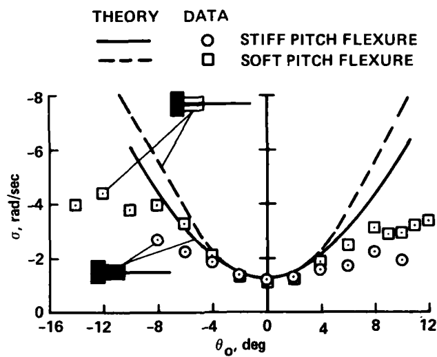
Figure 14.— Effect of pitch flexure stiffness on lead-lag damping variation with pitch angle, without precone or droop.
