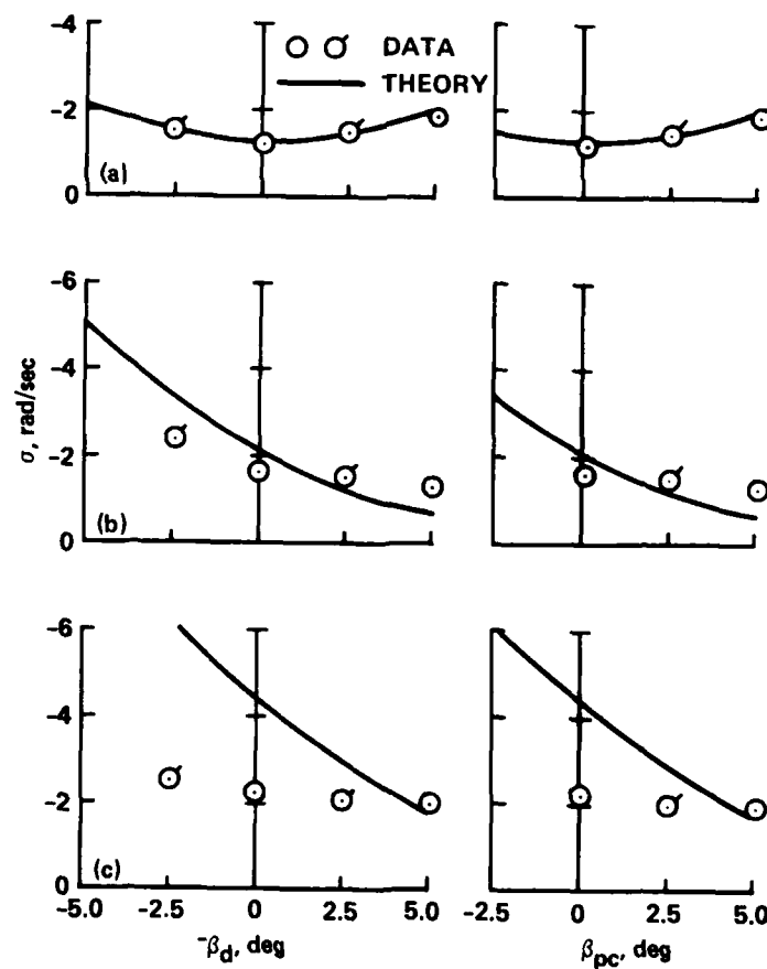
Figure 19.— Precone and droop effect on lead-lag damping at various pitch angles, stiff pitch flexure (flagged symbols represent blade set 1 data); a) \theta_o = 0^\circ , b) \theta_o = 4^\circ , c) \theta_o = 8^\circ .
