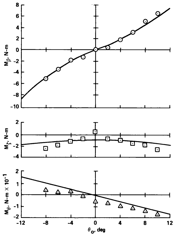
Figure 28.— Steady blade moments versus blade pitch angle, no precone or droop, stiff pitch flexure.
