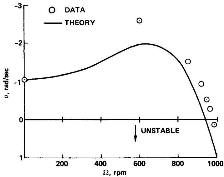
Figure 12.— Lead-lag damping versus rpm; 5^\circ precon, 0^\circ droop, \theta_o = 4^\circ , soft pitch flexure, blade set 2.
