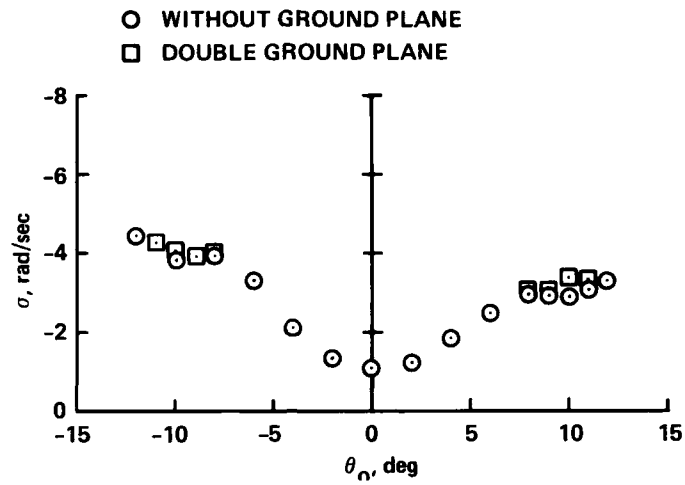
Figure 27.— Comparison of measured lead-lag damping with and without the double ground plane, lead-lag damping versus blade pitch angle, soft pitch flexure, no precone or droop.
