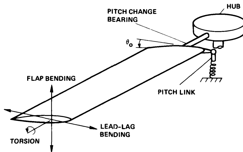
Figure 1.— Schematic of model rotor blade.
