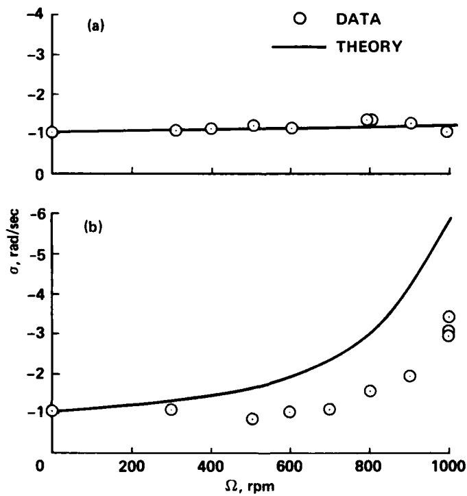
Figure 13.— Lead-lag damping versus rpm, without precon or droop, soft pitch flexures blade set 2; a) \theta_o = 0^\circ , b) \theta_o = 8^\circ .
