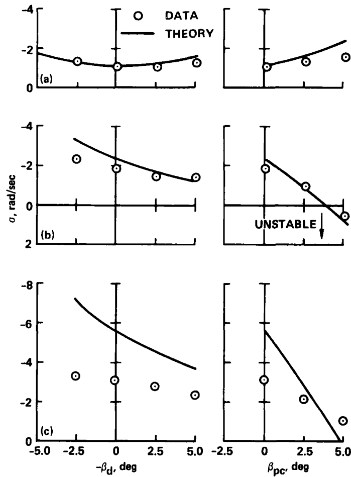
Figure 20.— Precone and droop effect on lead-lag damping at various pitch angles, soft pitch flexure; a) \theta_0 = 0^\circ , b) \theta_0 = 4^\circ , c) \theta_0 = 8^\circ .
