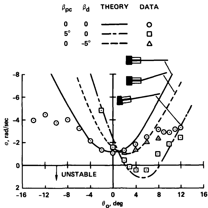
Figure 16.— Effect of precone and droop on lead-lag damping variation with pitch angle, soft pitch flexure.
