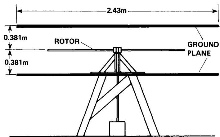
Figure 22.— Rotor stand with ground plane installations; a) Single ground plane, b) Double ground plane.
