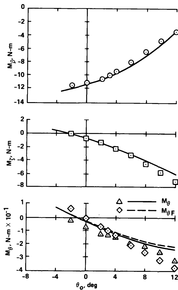
Figure 36.— Steady blade moment versus blade pitch angle, 5° precone, 0° droop, soft pitch flexure.
