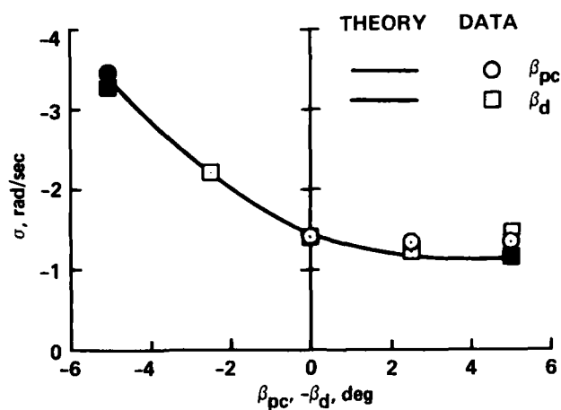
Figure 17.— Variation of lead-lag damping with precone and droop, \theta_o = 2^\circ , stiff pitch flexures (for solid dymbols, \theta_o = -2^\circ and the sign of the precone or droop angle has been reversed).
