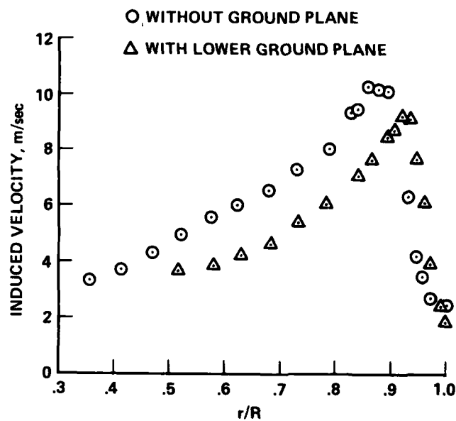
Figure 25.— Comparison of rotor induced velocity with and without ground plane, induced velocity versus radial station, \theta_0 = 10^\circ , h = 2.5 cm.
