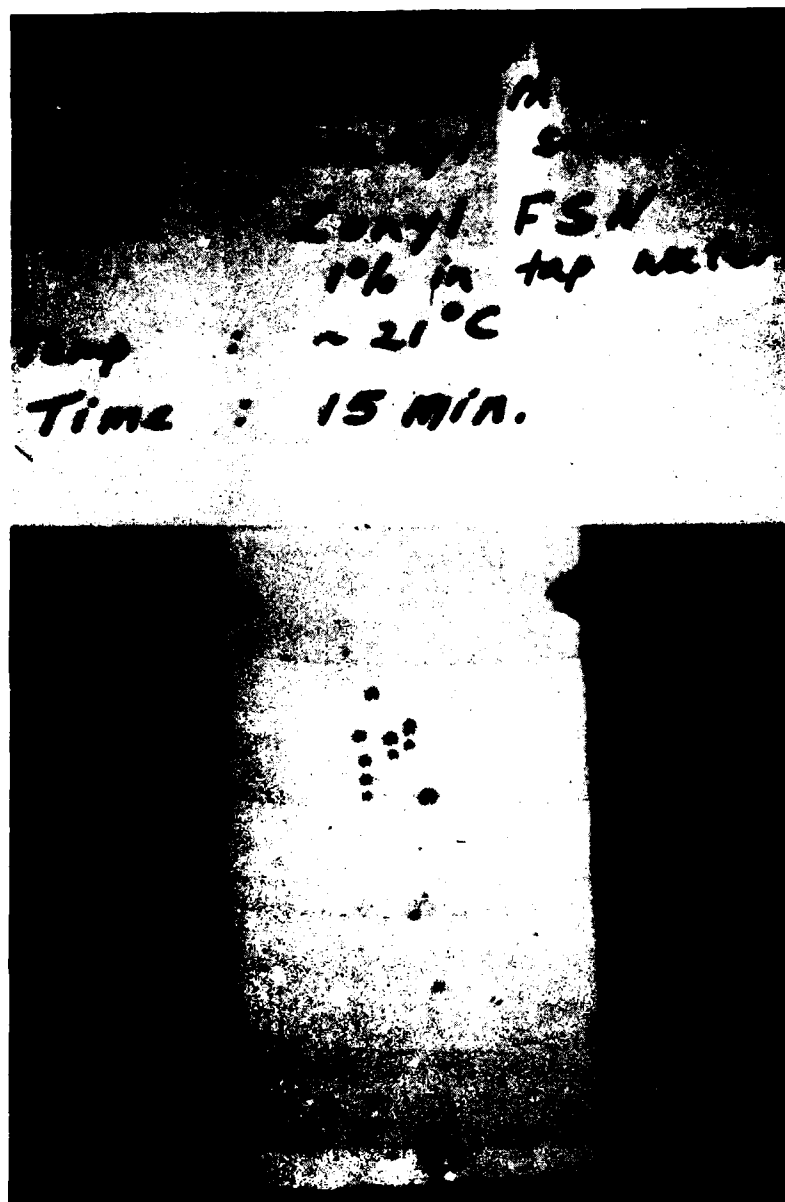
Figure 6 - Teflon substrate: Residual MST-D showing redeposition after spraying with Class B surfactant, Zonyl FSN, for 15 min
