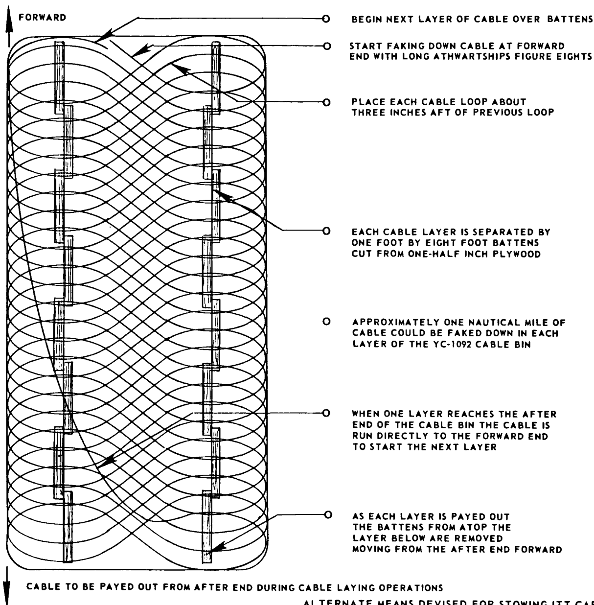
ALTERNATE MEANS DEvised FOR STOWING ITT CABLE FIGURE 19
