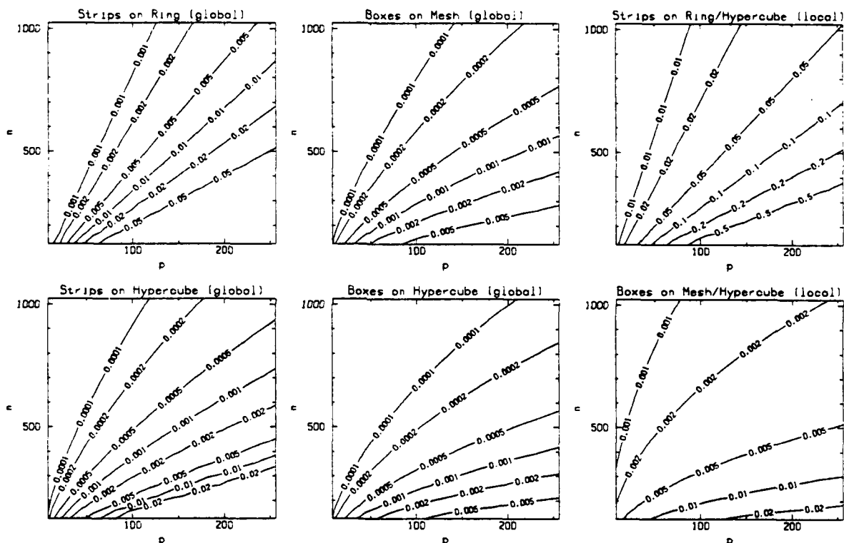
Figure 10: Contour plots of r \equiv \frac{f}{\alpha} (if global communication is dominant) or \frac{f}{\beta} (if local communication is dominant). If f/\alpha is greater than the value in the contour plot then communication takes more time than computation when global communication is dominant. Alternatively, for a given r , computation dominates above the contour, and communication below. Similarly for local communication.
