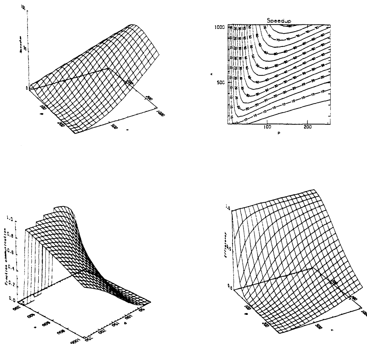
Figure 13: Theoretical parallelization measures for a ring, using strips for the domain decomposition. Communication-dominated processor.
