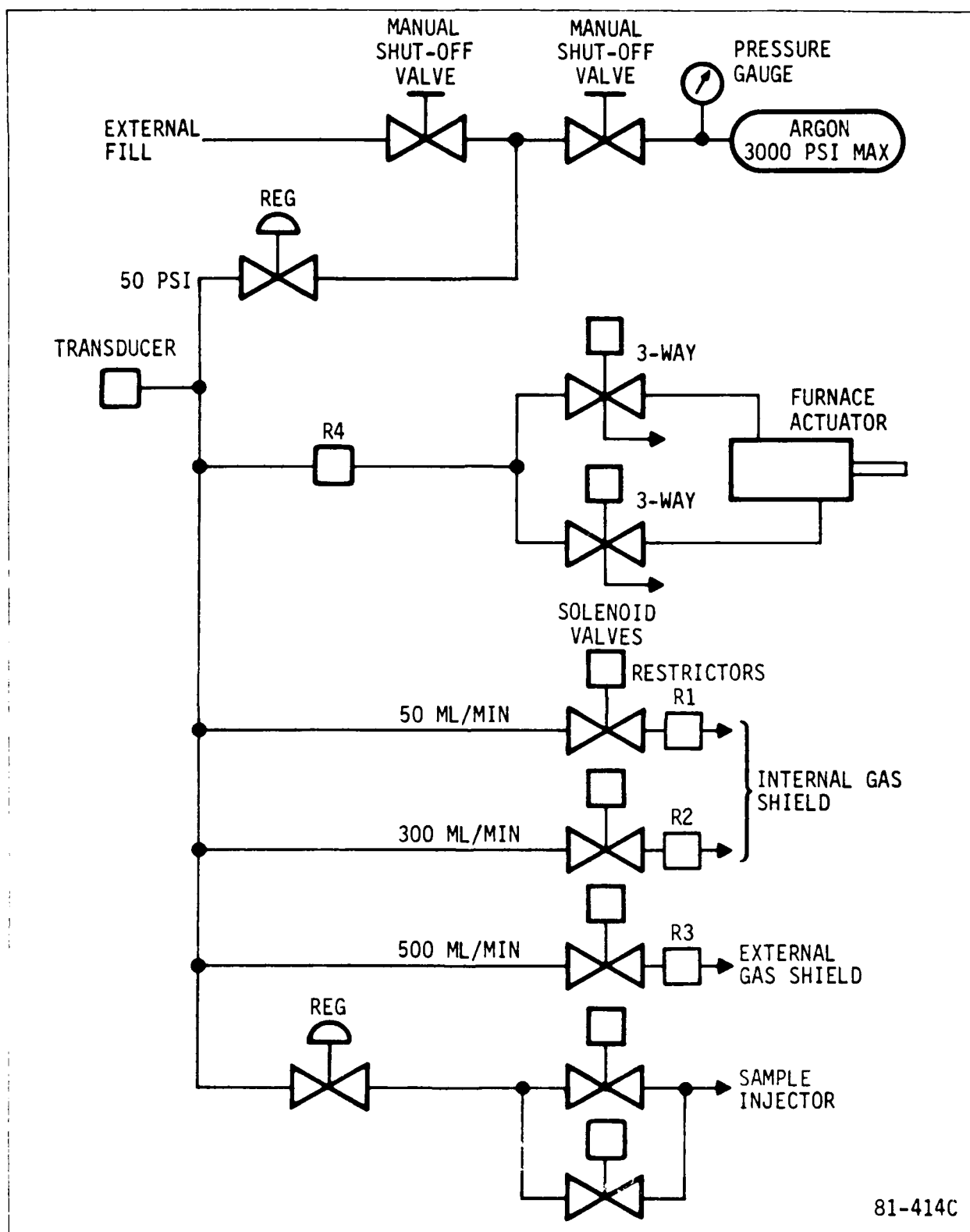
FIGURE 6. PWMA Argon Supply Schematic
