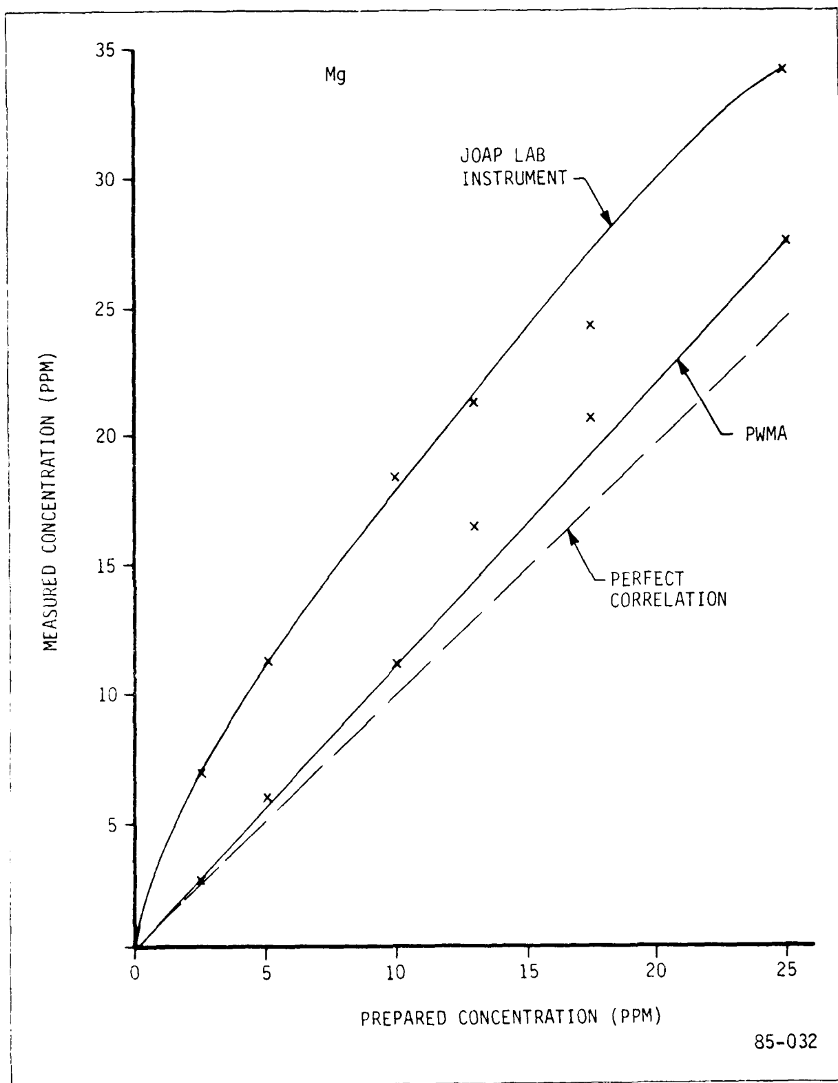
FIGURE 20. Correlation Data of Magnesium
