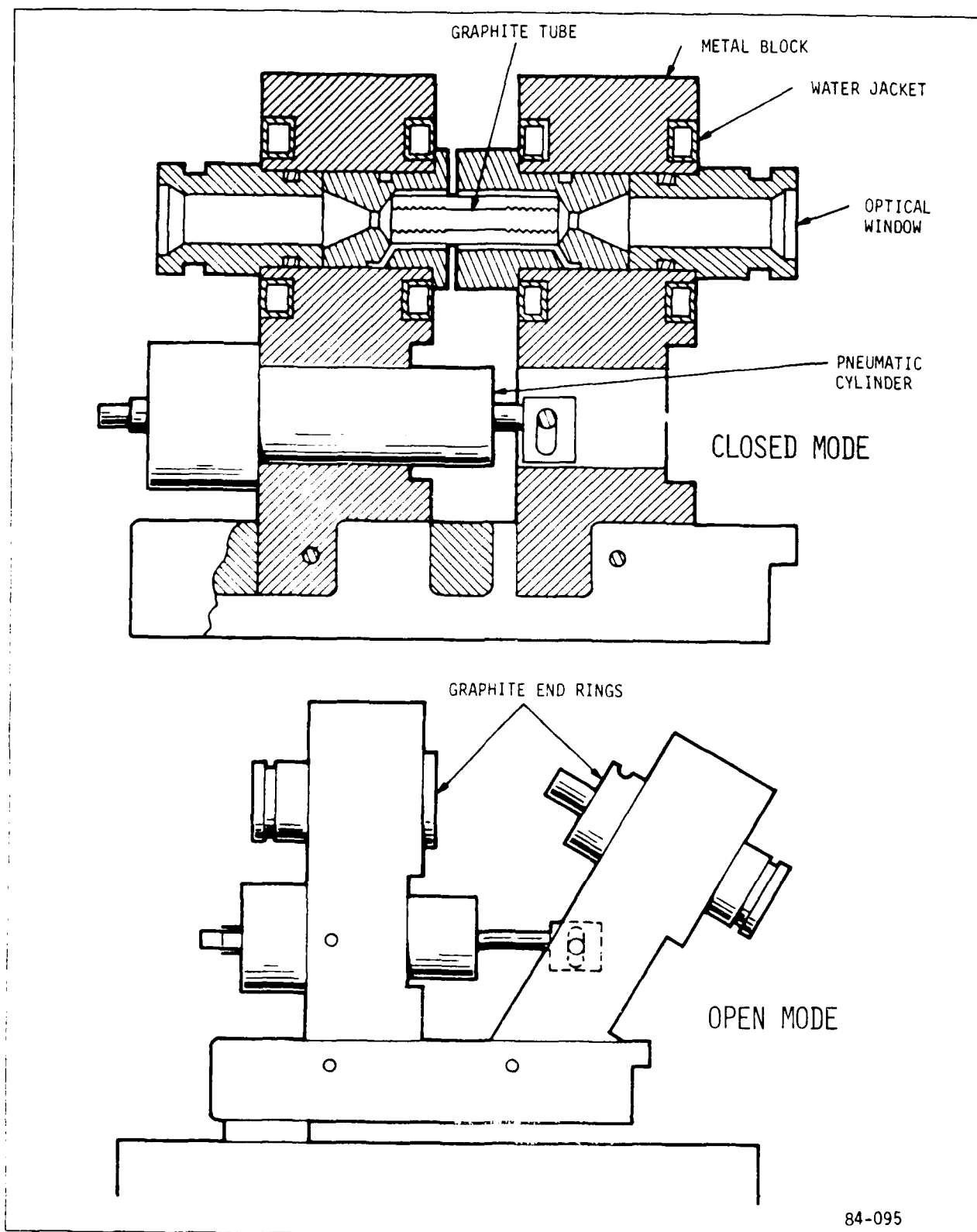
FIGURE 5a. Graphite Furnace, Cross-Sectional View
