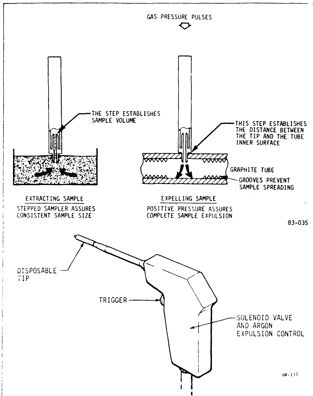
FIGURE 7. PWMA Sample Introduction System
