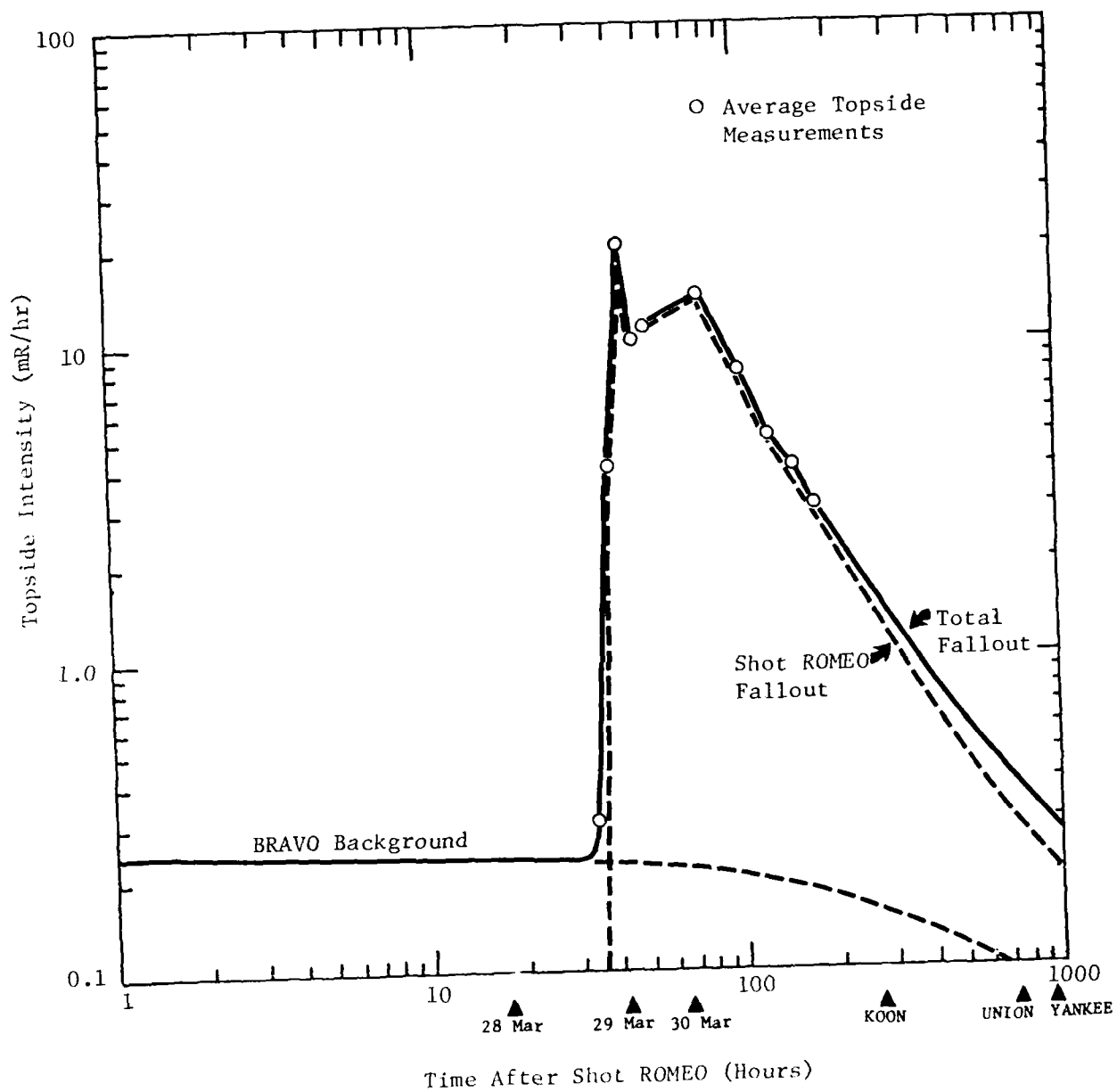
Figure 2-14. USS BELLE GROVE topside intensity following Shot ROMEO.
