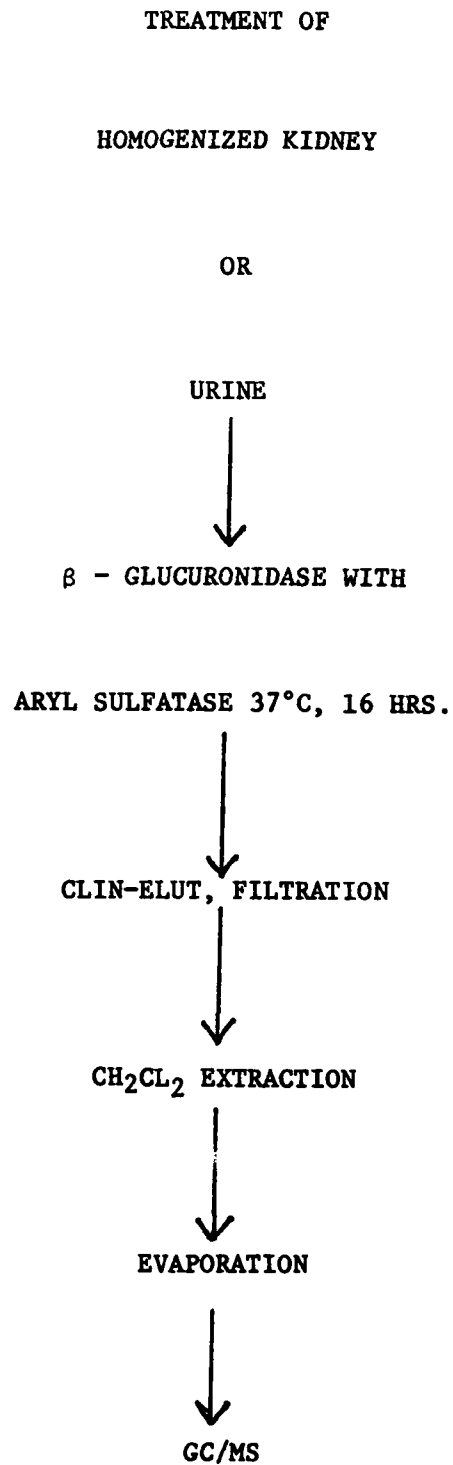
Figure 1. Analysis scheme for rat urine and rat kidney homogenate.
