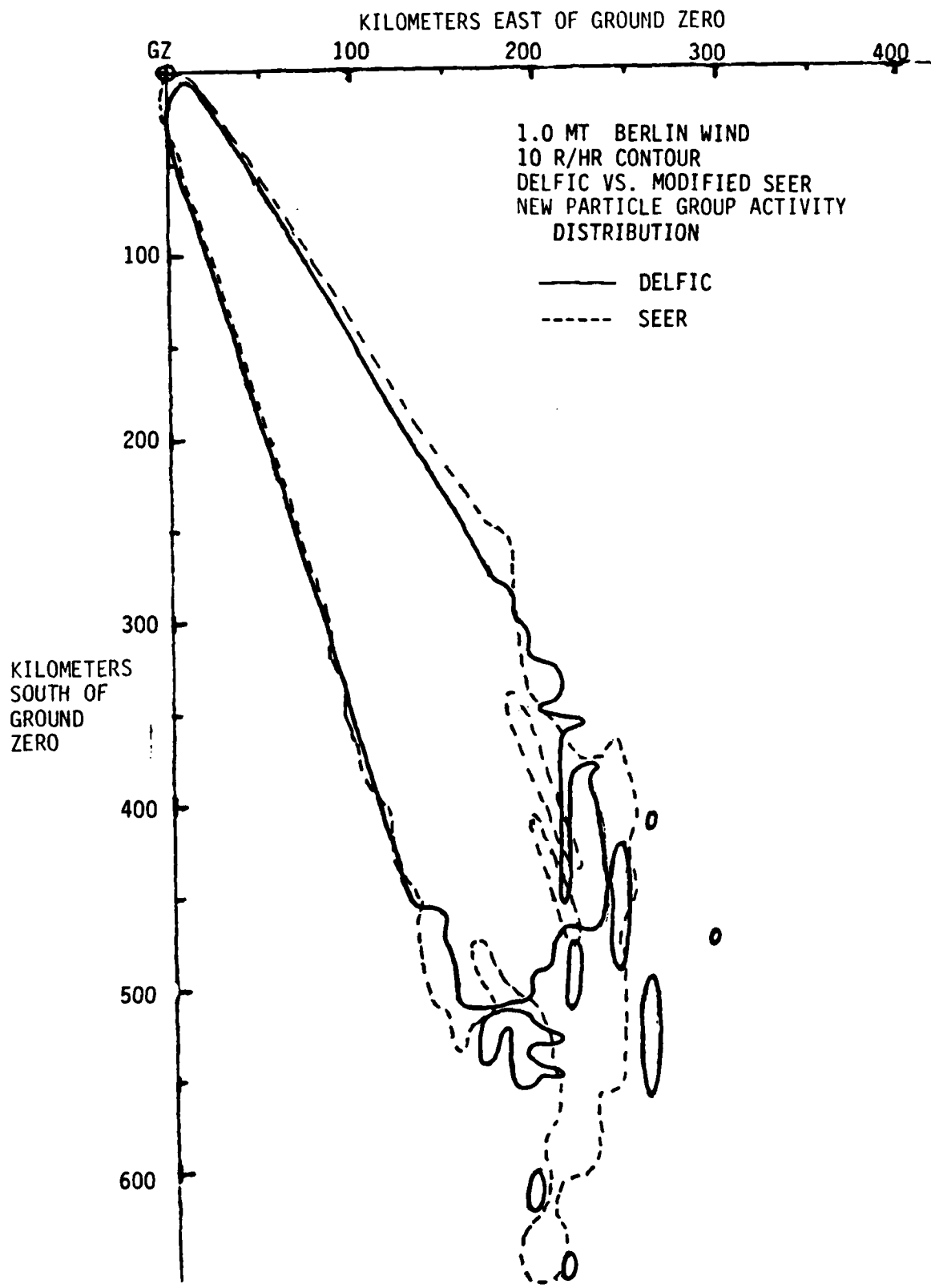
Figure 4-3. 10 r/hr contour, DELFIC vs. modified SEER, new activity distribution.
