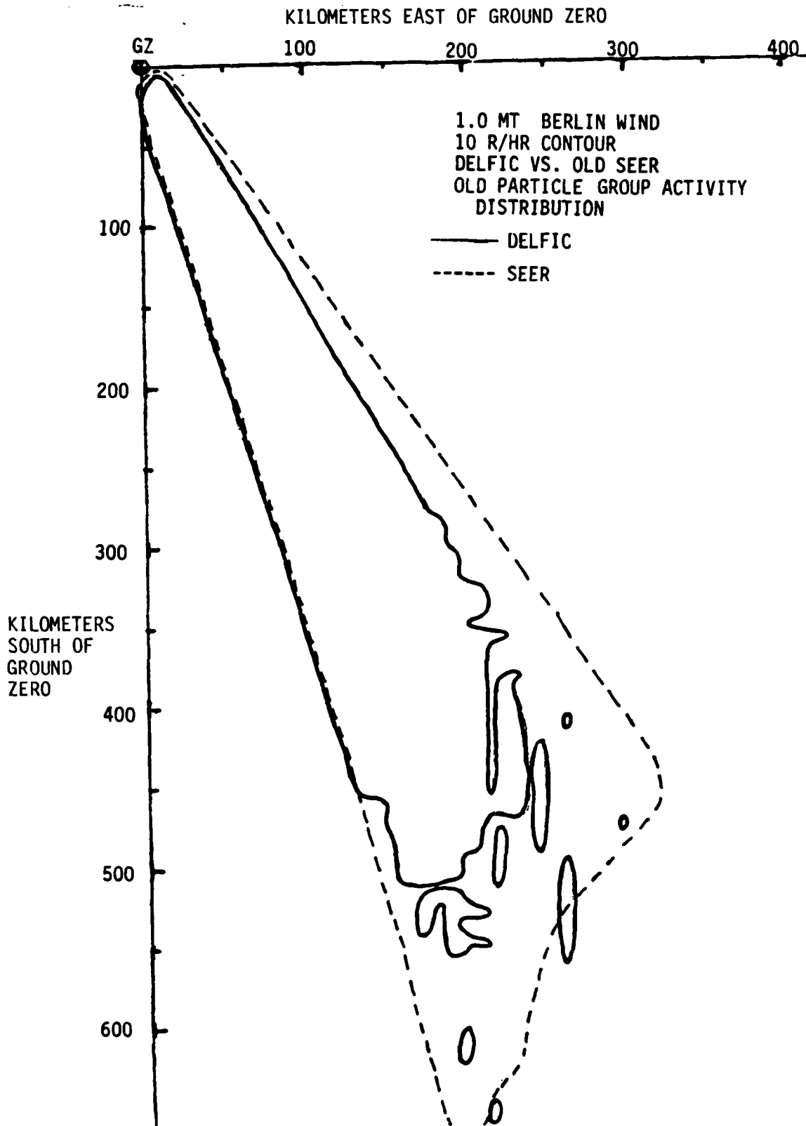
Figure 4-1. 10 r/hr contour, DELFC vs. old SEER.
