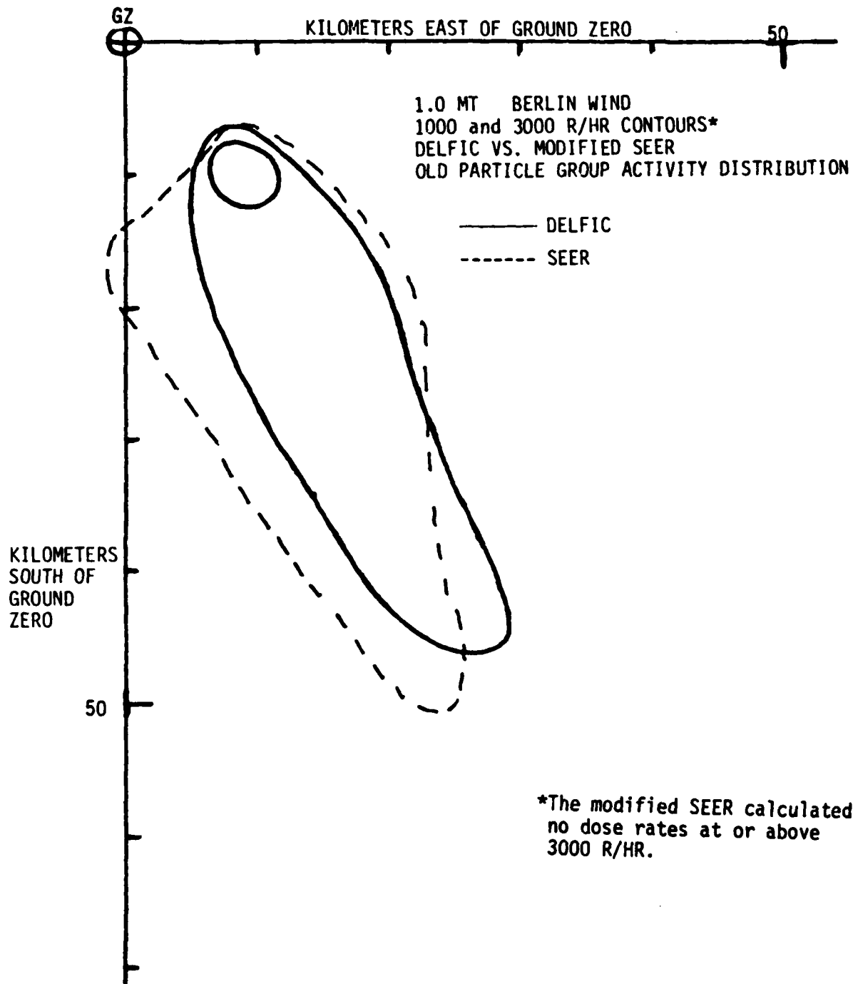
Figure 4-10. 1000 and 3000 r/hr contours, DELFC vs. modified SEER.
