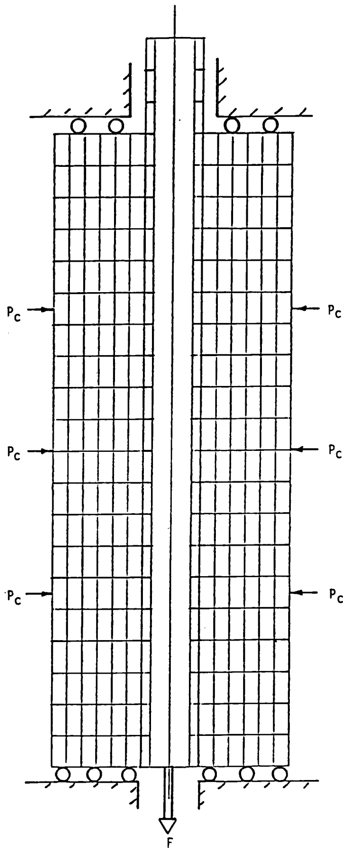
Figure D.1. Finite element idealization.
