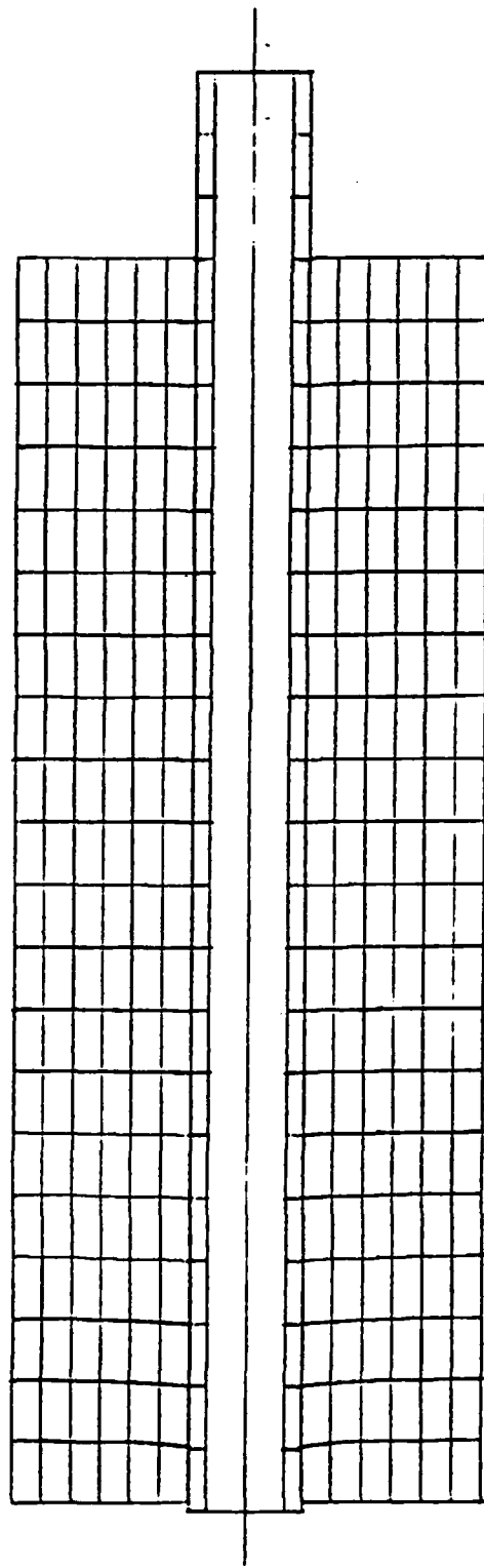
Figure D.5. Slip development along conduit at pullout load of 5.5 kN.
