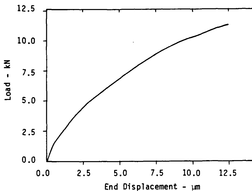
Figure D.33. End displacement versus pullout load, Run T.
