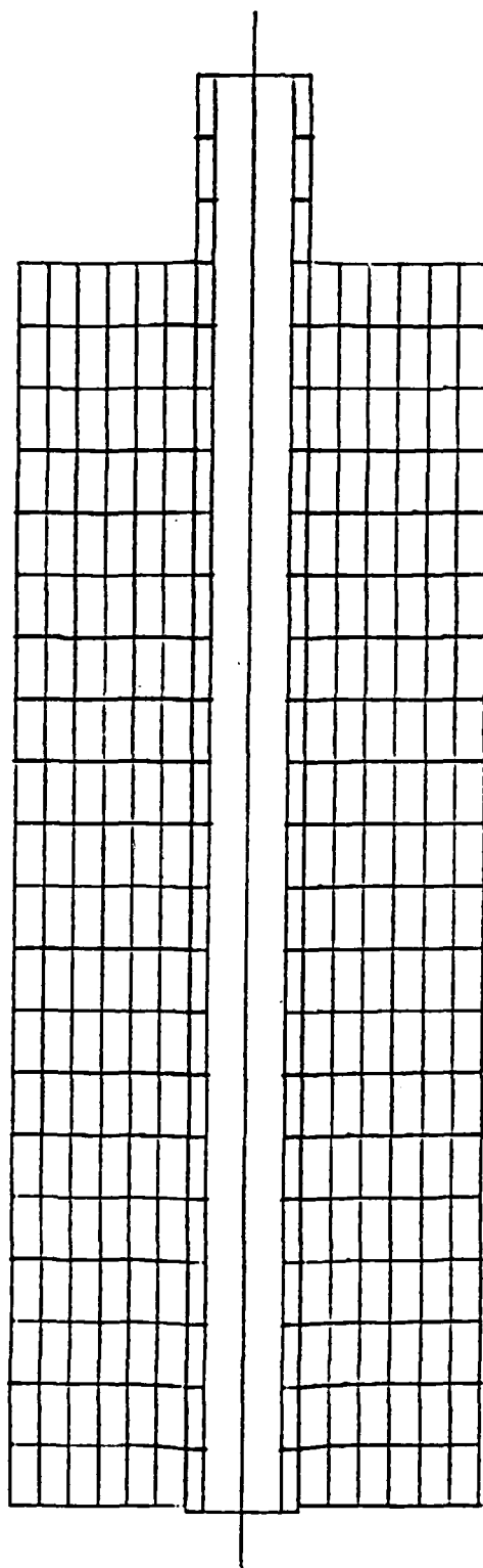
Figure D.4. Slip development along conduit at pullout load of 3.6 kN.
