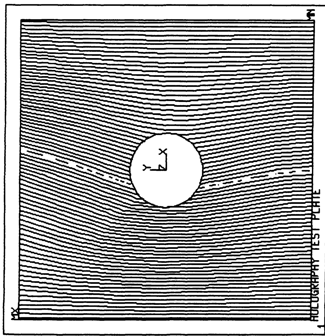
Figure 5-6. Mode Two from a Dynamic Analysis of the Clamped Plate in Figure 5-1. Linear fringes have been added.
