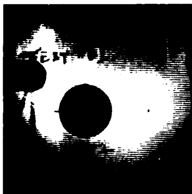
Figure 4a. Reconstructed image of double exposure hologram resulting from tipping the test plate about the x-axis between exposures
