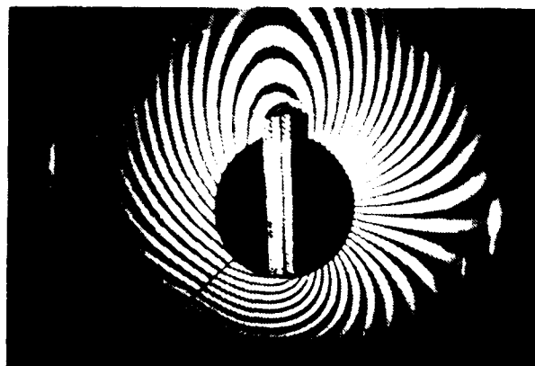
Figure 9a. Reconstructed image from double exposure hologram for the case of a stressed plate having a through cut without the addition of linear fringes
