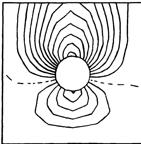
Figure 5. Computer model corresponding to Figure 4.
