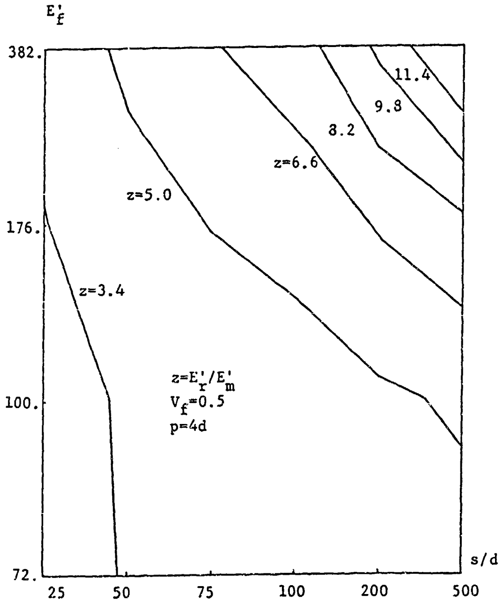
Figure 9.27: Contour Curves of E'_f/E'_m vs s/d and E'_f for Randomly Oriented Fiber Composites
