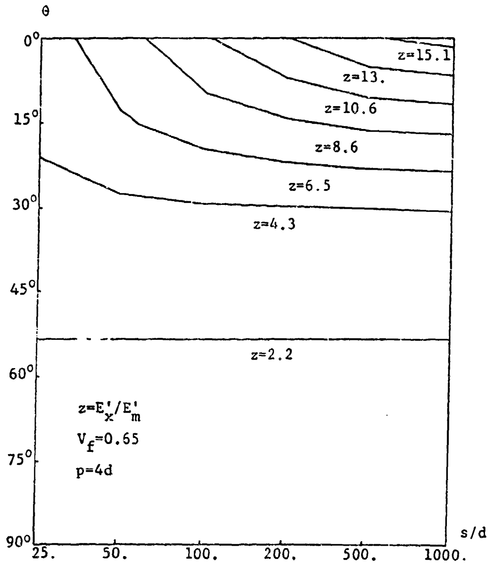
Figure 9.16: Contour Curves of E'_x/E'_m vs \theta and s/d for Unidirectional Kevlar Epoxy Composites
