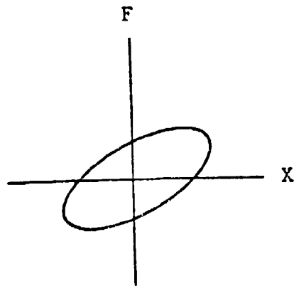
Figure 2.5: Hysteresis Loop of An Inelastic Body
