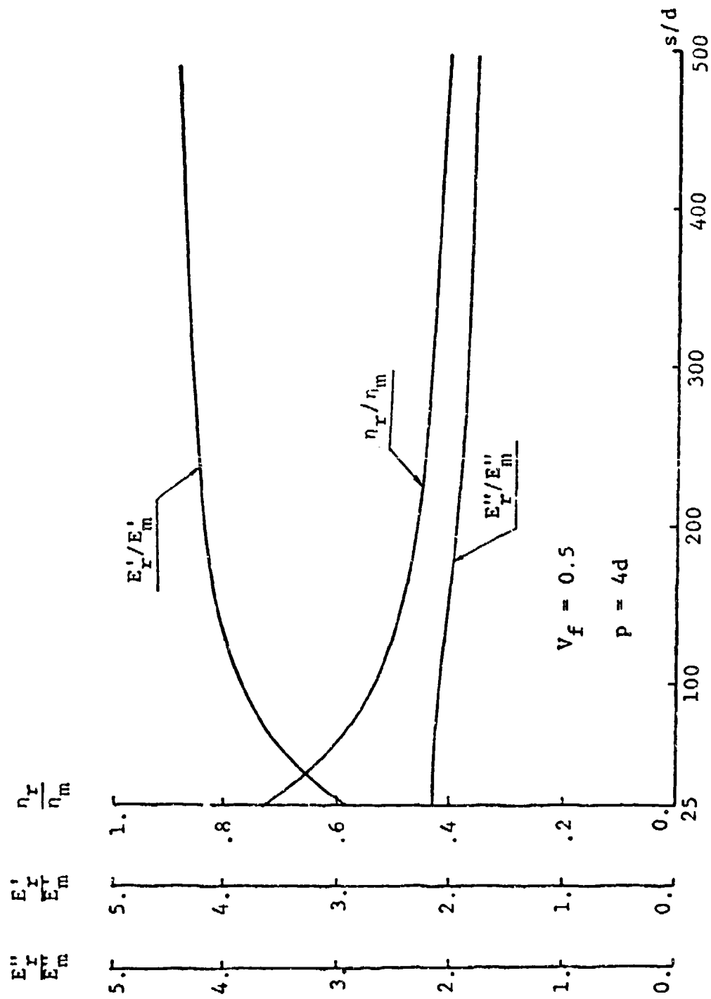
Figure 9.18: Plots of \eta_I/\eta_m , E'_I/E'_m and E''_I/E''_m vs s/d for Randomly Oriented Glass Epoxy Composites
