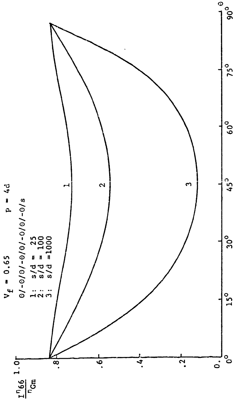
Figure 9.34: Plots of I_{\eta 66} / \eta_{Gm} vs \theta Using s/d as a Parameter for Angle Ply Graphite Epoxy Composites
