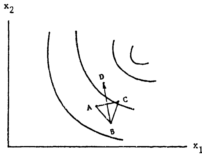
Figure 8.1: Rule 1 of Sequential Simplex method
