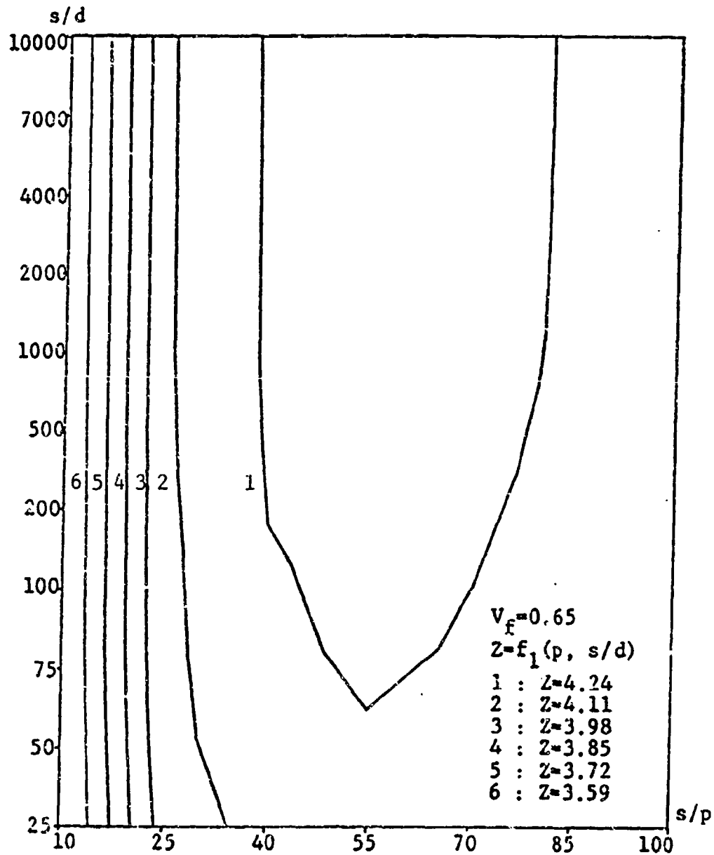
Figure 9.43: Contour Curves of Objective Function for Case One vs s/d and s/p for Graphite Epoxy Composite Plate
