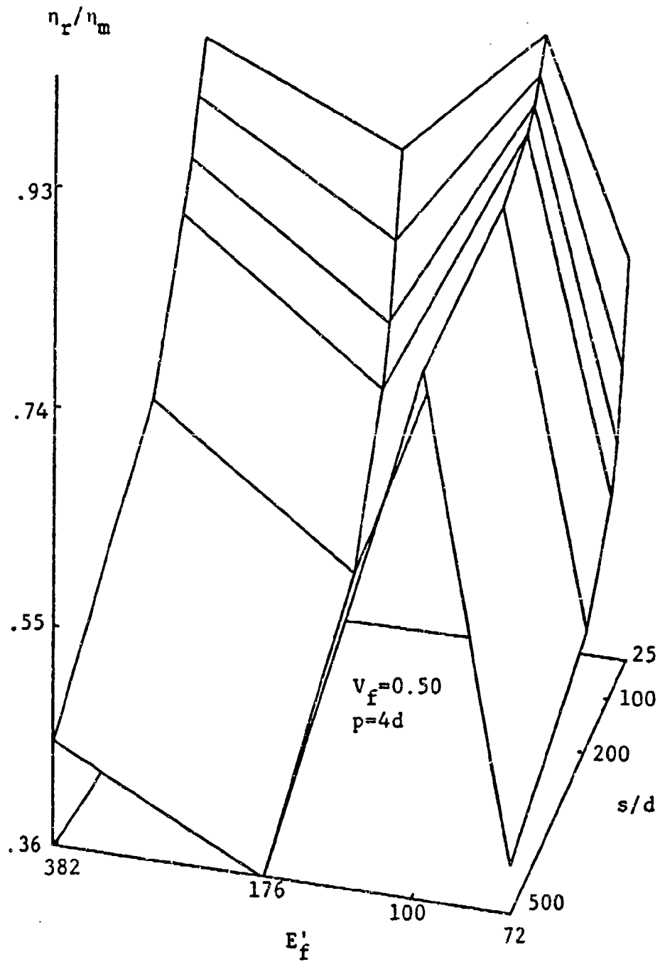
Figure 9.26: Three-Dimensional Plots of \eta_T/\eta_L vs s/d and E'_f for Randomly Oriented Fiber Composites
