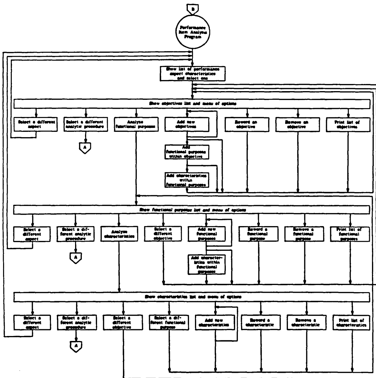
Figure 2. Simplified Flow Chart for Performance Rem Program
