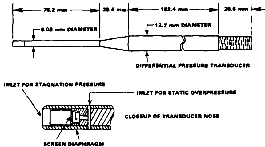
Figure 13. Configuration of the differential pressure gage for blast wave measurements.
