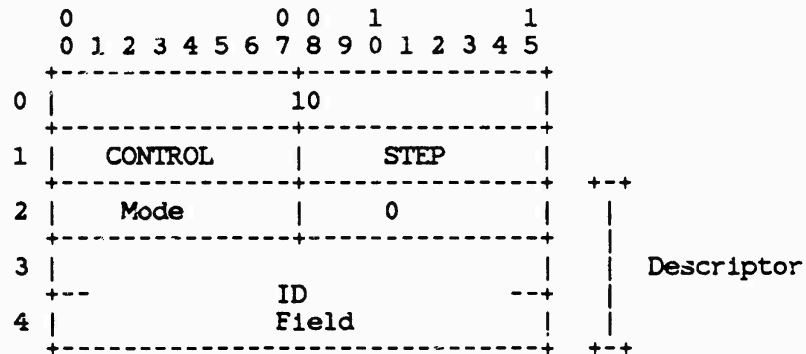
STEP Command Format Figure 38
