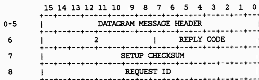
Figure 22 . LEAVE GROUP REPLY
