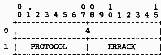
ERRACK Command Format Figure 25
