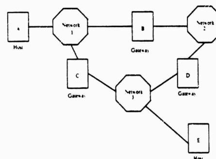
Source Routing
