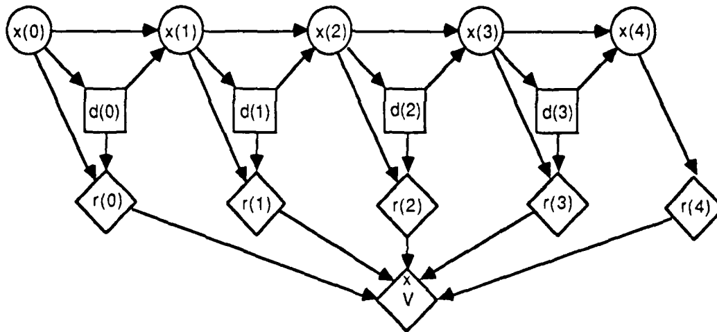
Figure 5.3. Influence diagram for a risk sensitive MDP with exponential utility function.
