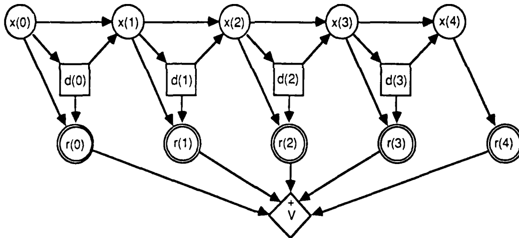
Figure 5.1a. Graph of the influence diagram for an additive MDP.
