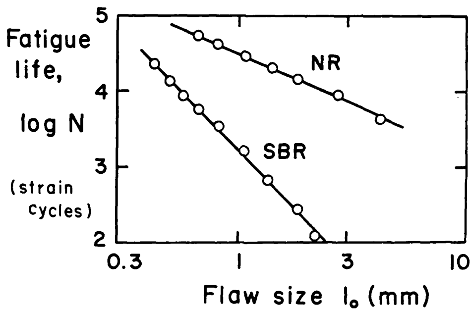
Fig. 6. Fatigue life \underline{N} of natural rubber (NR) and a butadiene-styrene rubber (SBR) plotted against the depth \underline{l}_0 of an initial edge crack (7).
