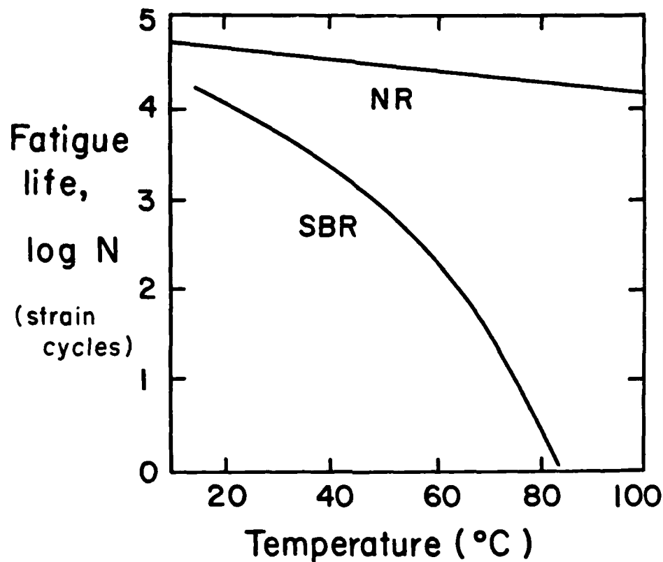
Fig. 5. Fatigue life \underline{N} of natural rubber (NR) and a butadiene-styrene rubber (SBR) plotted against the test temperature \underline{T} (7).
