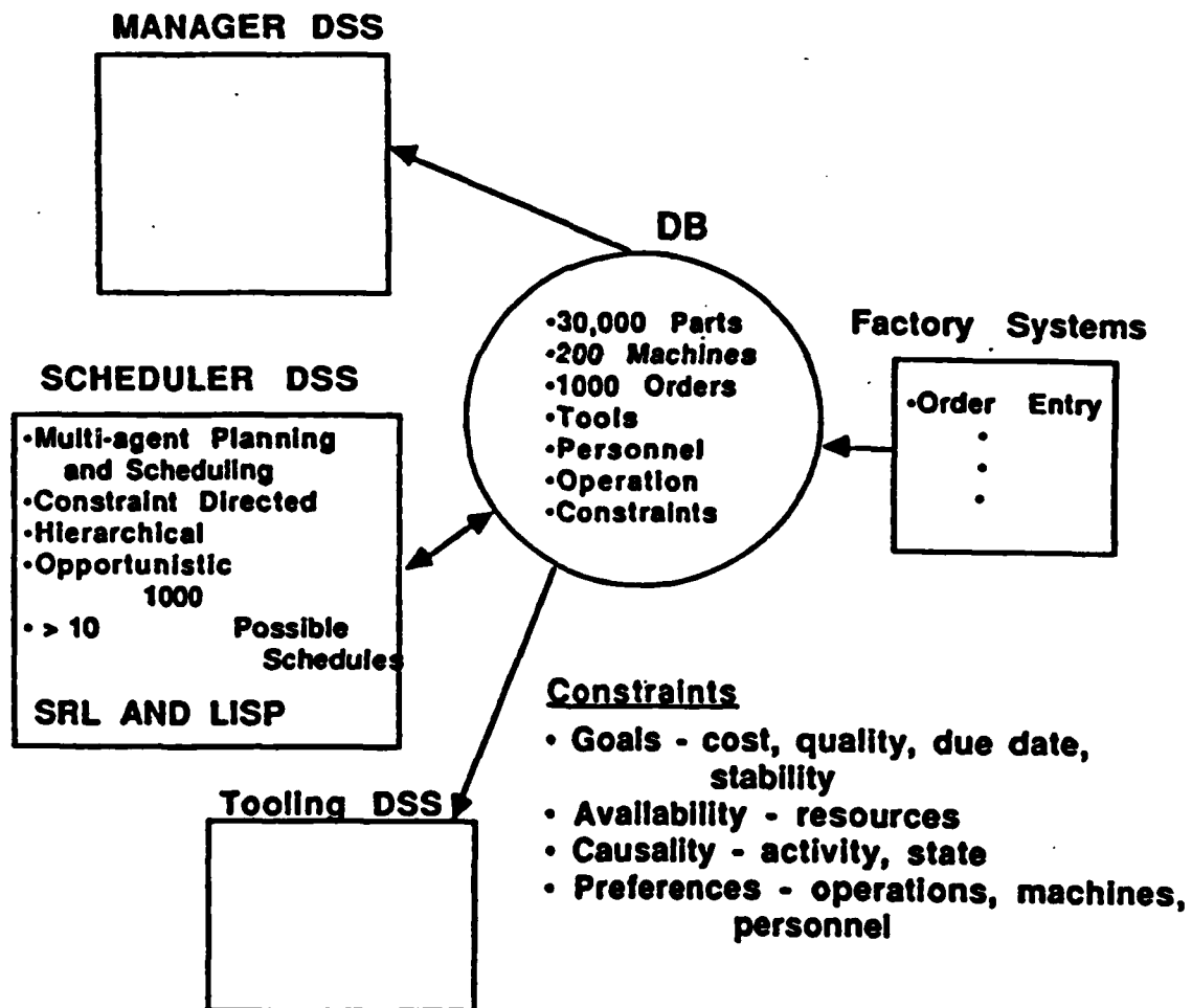
Figure 2-2: ISIS Process Architecture
