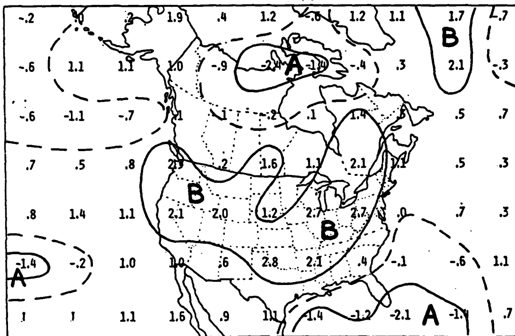
FIG. 20. January Student's t-test statistics comparing SSW cyclone frequency with non-SSW frequency for each grid box. Positive values indicate SSW frequency is less; negative values indicate cyclone frequency is greater during SSW. Dashed lines delineate areas of above and below the non-SSW normal frequency. Solid lines indicate areas of significant difference at the 90% confidence level. Below normal areas are labeled "B", whereas areas above normal are labeled "A".
