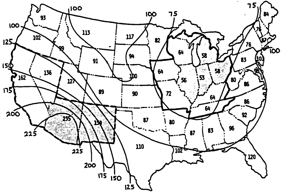
FIG. 23. As Fig. 22, except for February.
