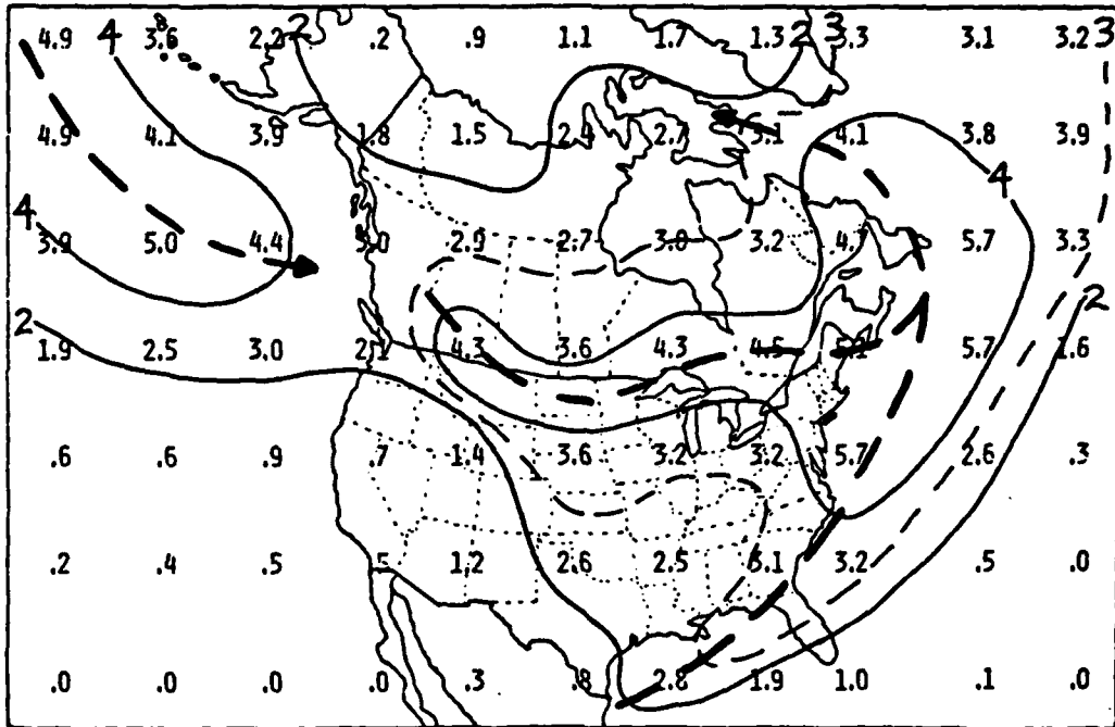
FIG. 18. Mean January storm tracks of SSW years for the period 1955 to 1980. Numbers are the mean frequency for each grid box. Dashed lines with arrows indicate the mean storm tracks and the direction of cyclone movement. Isopleth interval is two.
