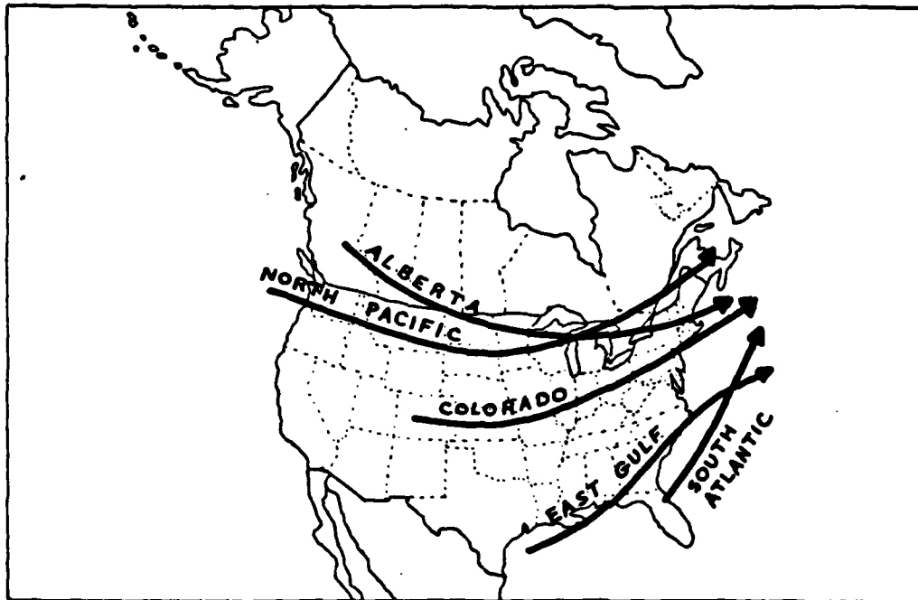
FIG. 15. Principle storm tracks of the United States(after Bowie and Weightman, 1918).
