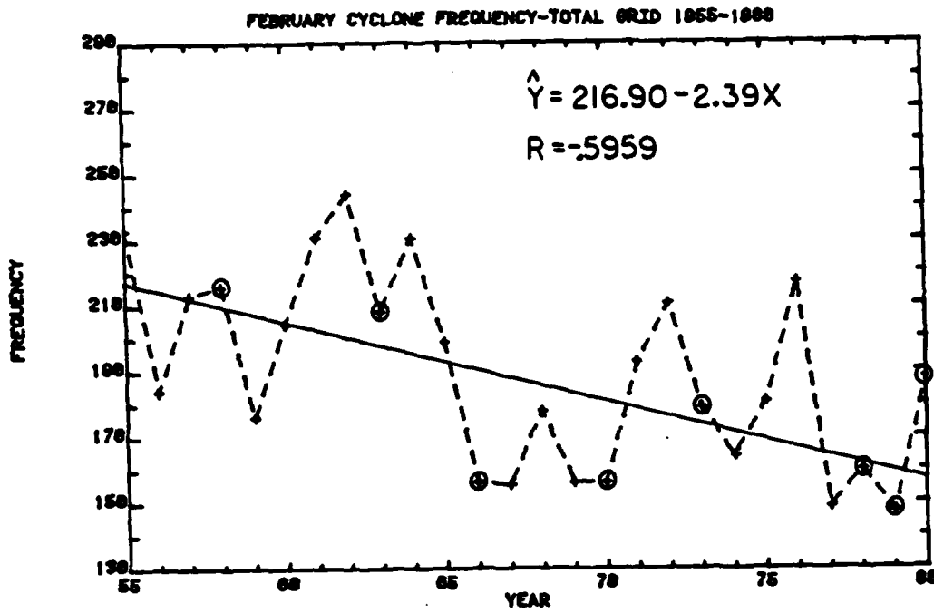
FIG. 12. As Fig. 11, except for February.
