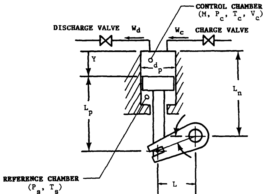
Figure A-1. Actuator schematic.
