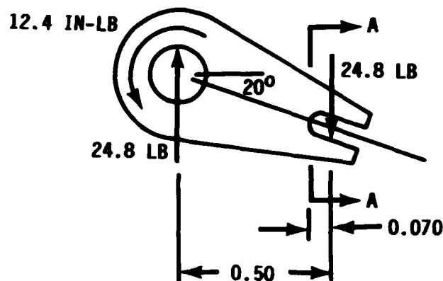
Figure 15. Crank freebody diagram.
