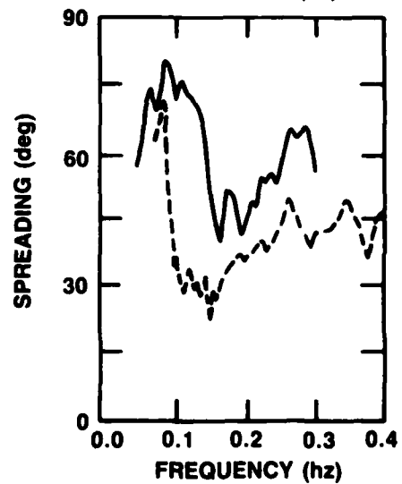
Figure 22 - Energy Densities, Mean Directions, and Spreading for Runs 36 and 38
