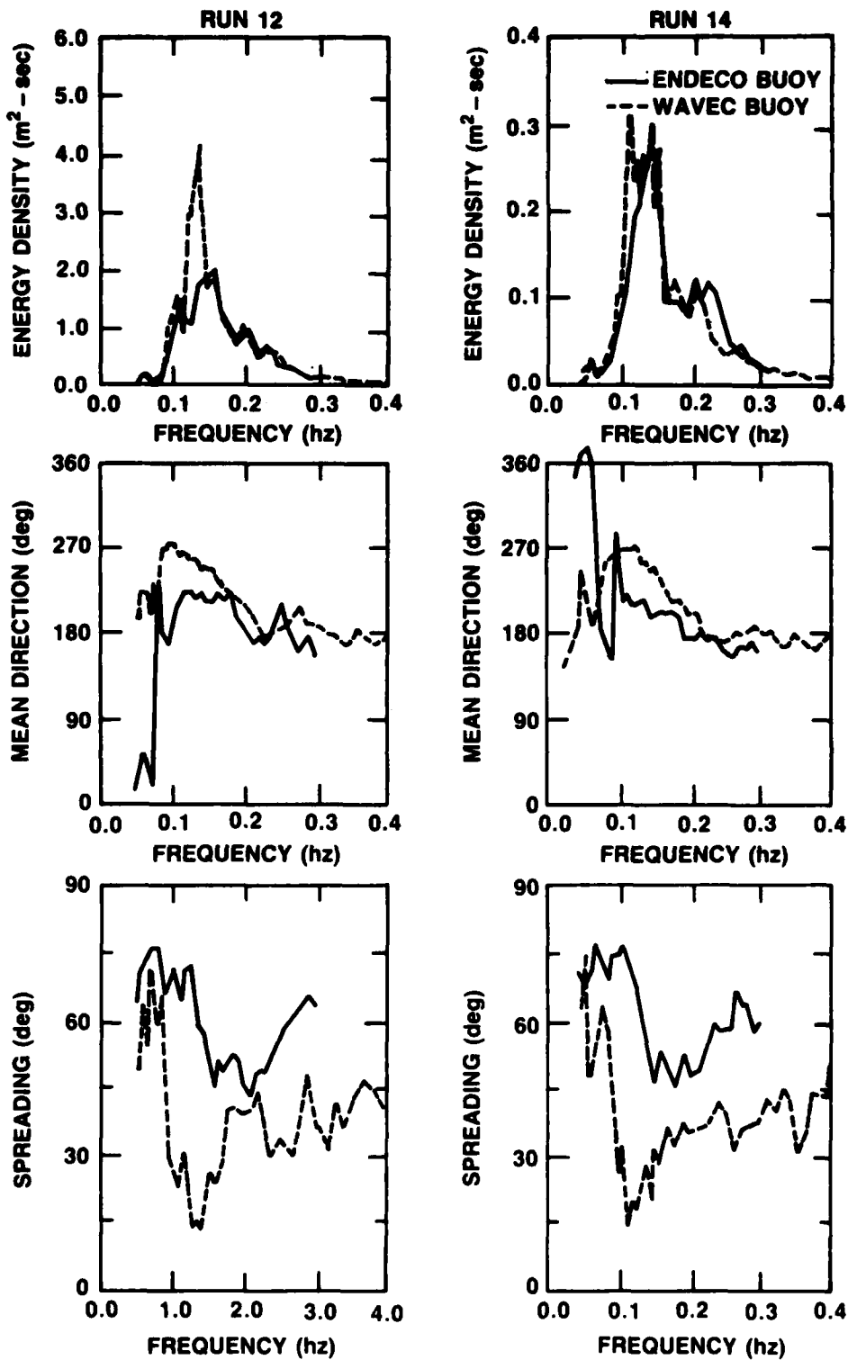
Figure 12 - Energy Densities, Mean Directions, and Spreading for Runs 12 and 14
