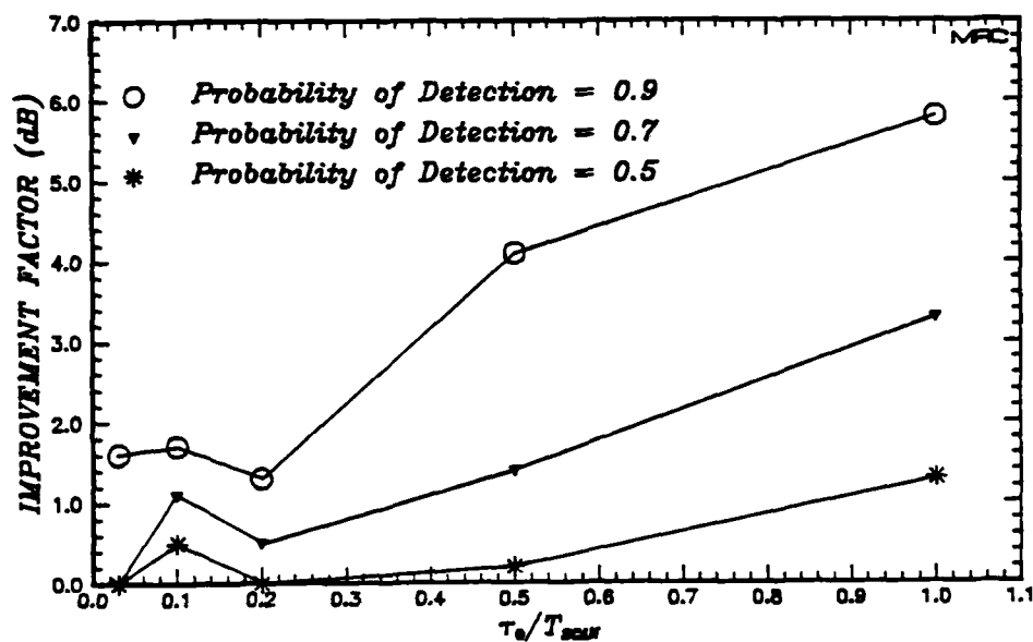
Figure 14. Improvement factor vs \tau_0/T_{SCAN} for 3 values of probability of detection.
