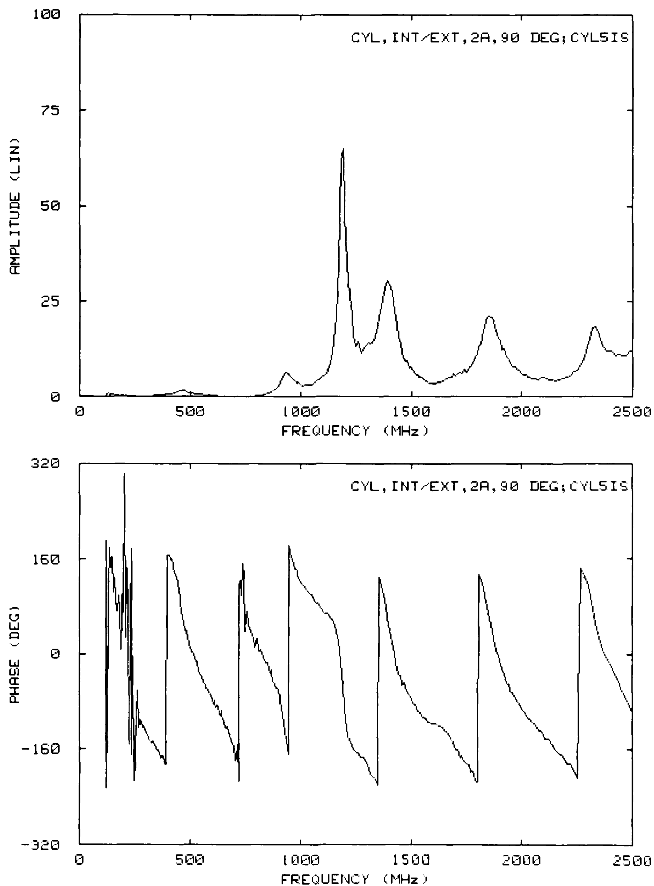
Figure 6.23. Transfer coefficients for \phi = 90^\circ , D = 2.0 A.
