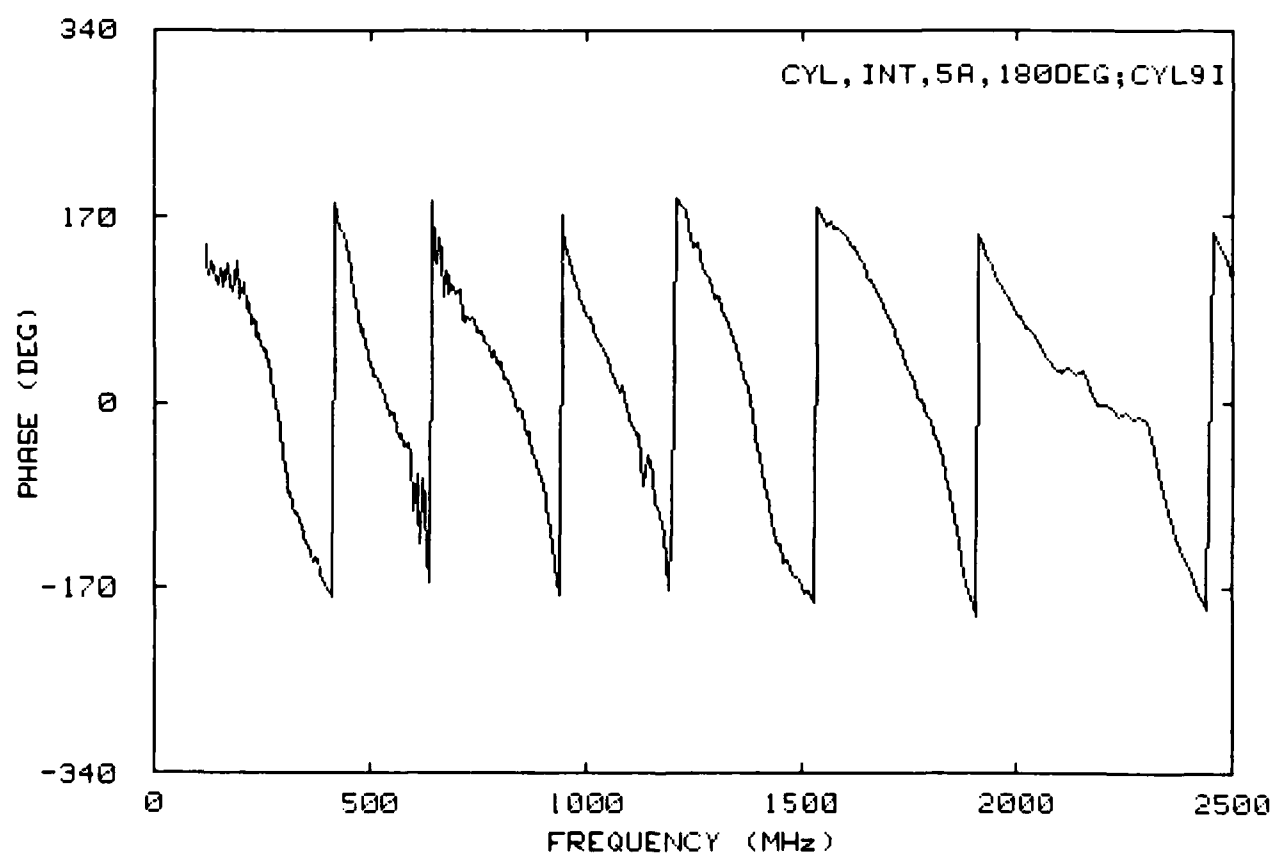
Figure 6.18. Interior coupled-field measurement at \phi = 180^\circ , D = 5.0 A.
