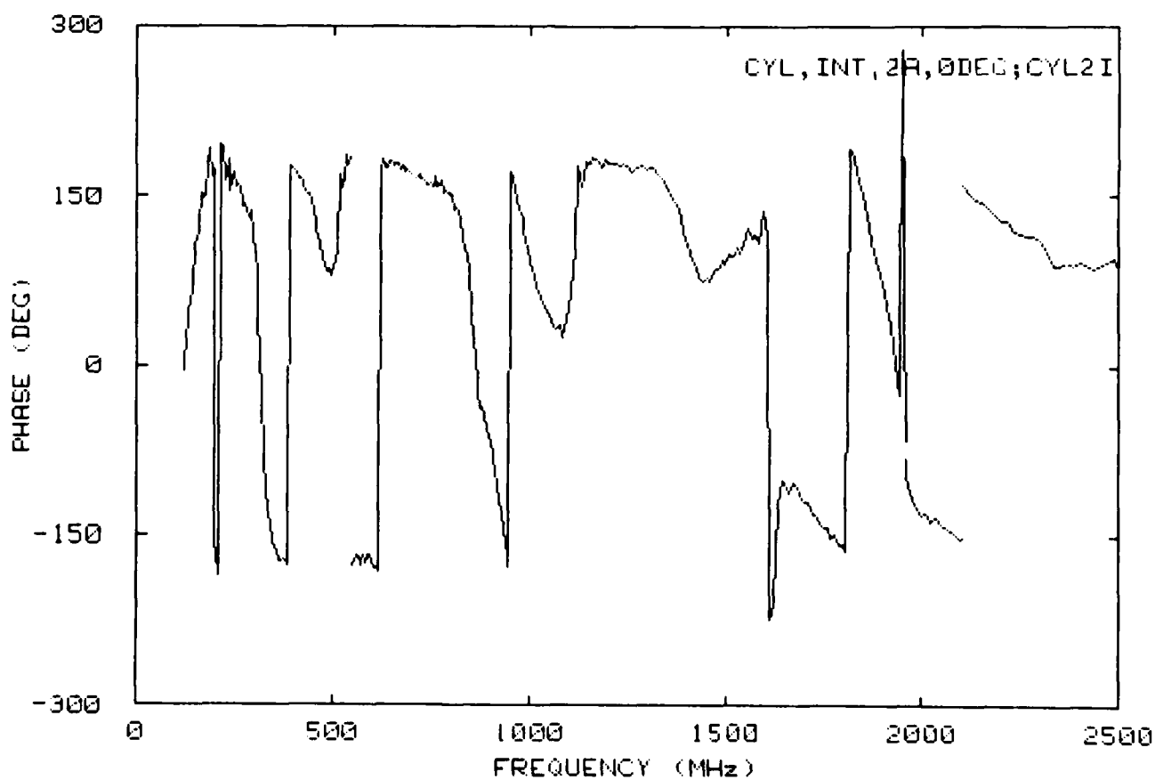
Figure 6.11. Interior coupled-field measurement at \phi = 0^\circ , D = 2.0 A.
