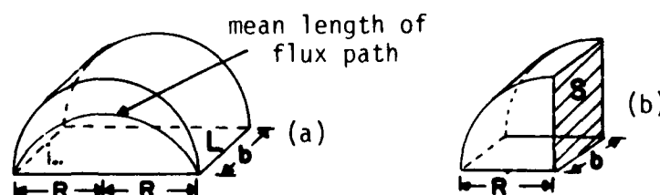
Figure A-2. Semicircular cylindrical sections.
