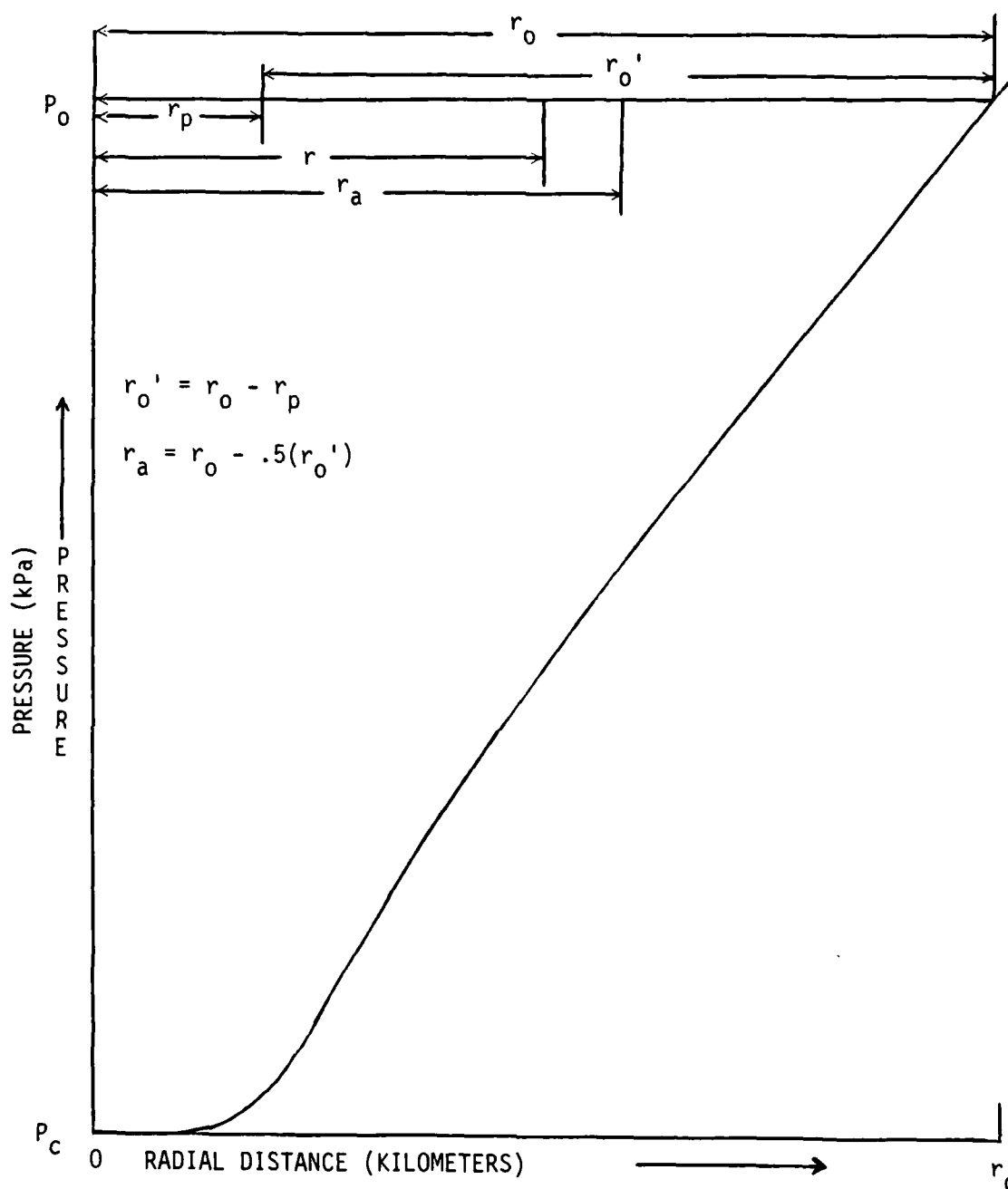
Fig. 6. Adjustment of the distance over which pressure gradient is measured ( r_o to r_o' ) and the radius of measurement ( r to r_a ). The minimum sea level pressure radius ( r_p ) represents the point on the pressure curve after which a quasi-linear approximation can be made.
