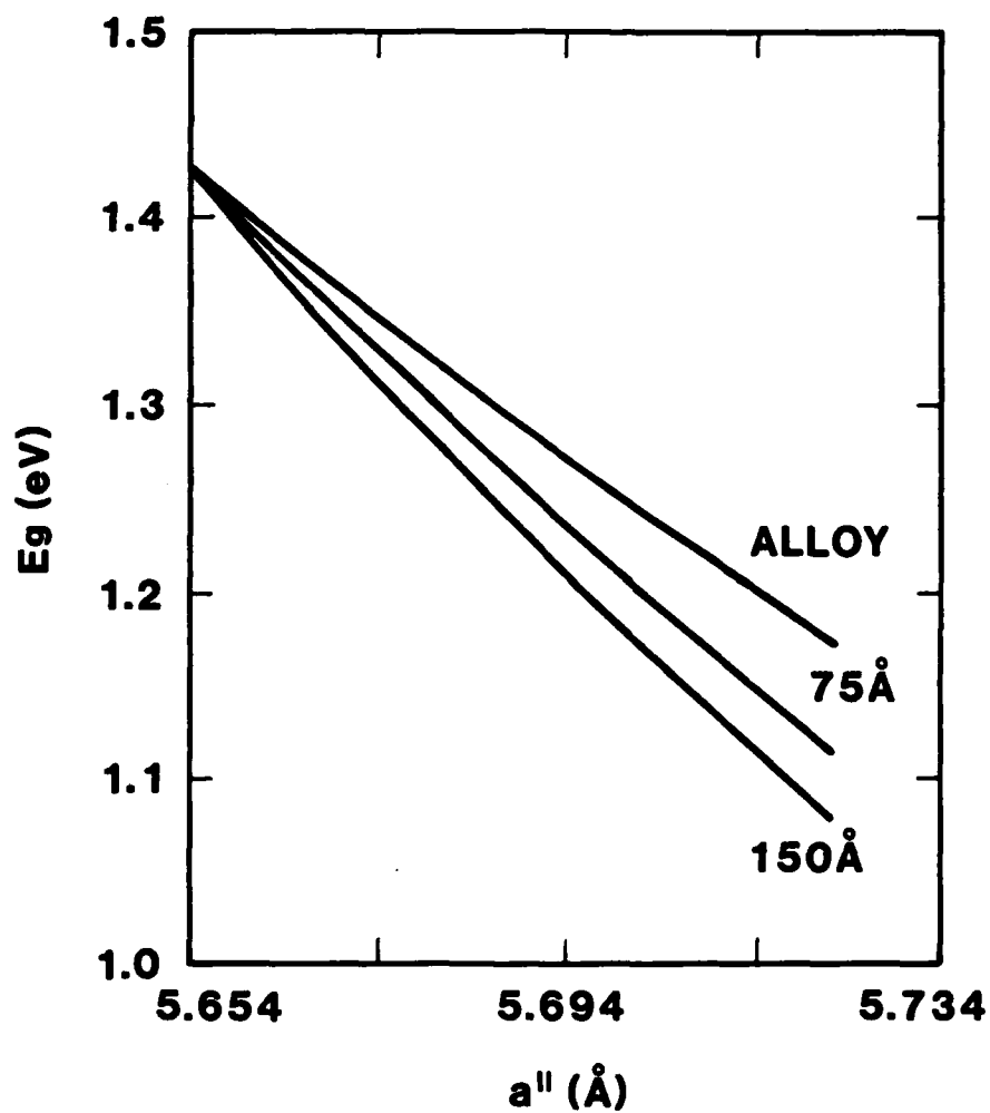
Fig. 10. Band gap of \text{GaAs-In}_x\text{Ga}_{1-x}\text{As} as a function of lattice constant parallel to the interface. The curve labeled Alloy refers to bulk InGaAs, and the dimensions listed apply to the layers of both materials (in different samples). (40)
