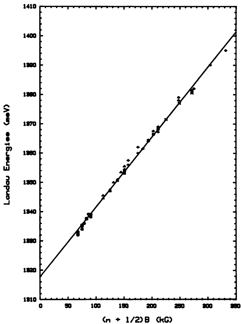
Fig. 18. Landau level energies as function of normalized magnetic field, Sample M316, at T = 4 °K, P = 1 bar.
