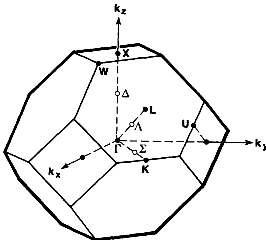
Fig. A-2. The first Brillouin zone of the face-centered cubic lattice showing selected symmetry points and axes.
