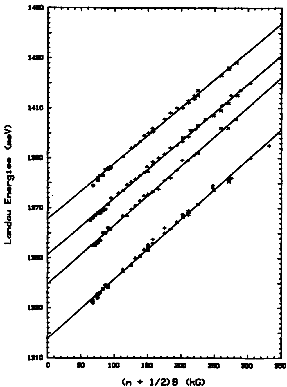
Fig. 19. Landau level energies as function of normalized magnetic field, Sample M316, at T = 4 K, P = 3.830 kbar, 3.013 kbar, 2.005 kbar, and 1 bar (top to bottom).
