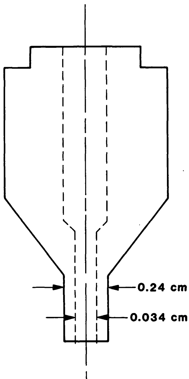
Fig. 5. The pressure plug (BeCu), encasing the optical fiber, provides the seal between the high-pressure region and the ambient atmosphere and allows optical access to the pressure region.
