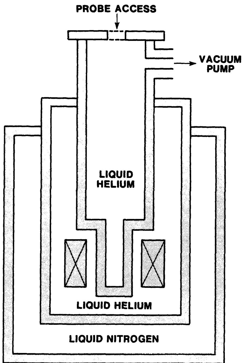
Fig. 6. Triple Dewar system showing magnet position and access ports.
