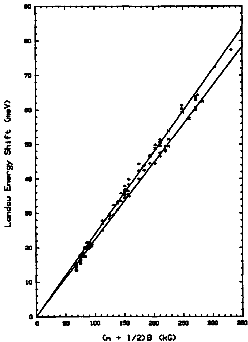
Fig. 20. Landau level energies as function of normalized magnetic field, Sample M316, at T = 4 °K, P = 1 bar (upper) and P = 3.83 kbar (lower).
