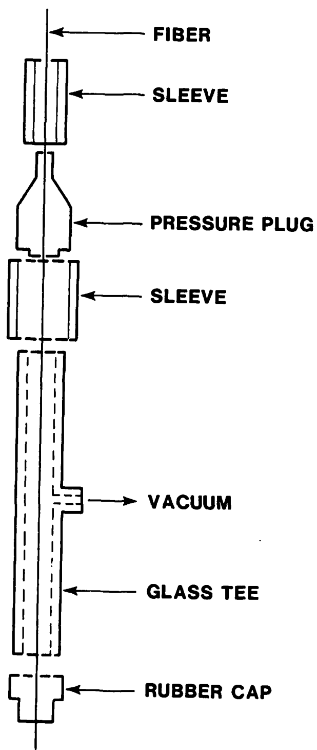
Fig. 8. Pressure plug holder used during sealing around the optical fiber.
