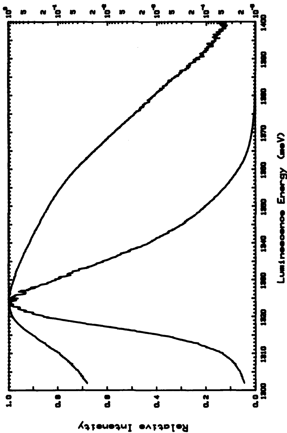
Fig. 11. Luminescence spectrum of Sample M316 with P = 1 bar, B \approx 1 kG. Broader curve represents the logarithmic intensity.
