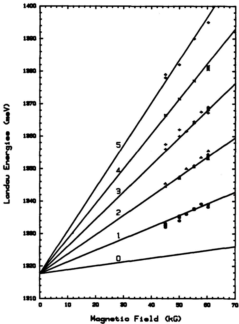
Fig. 17. Landau level energies as function of magnetic field, Sample M316, at T = 4 \text{ K} , P = 1 \text{ bar} .
