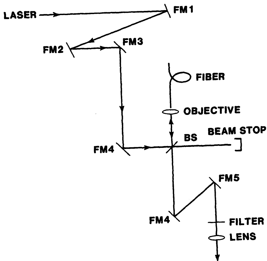
Fig. 4. Placement of optical elements. Laser beam is coupled into the optical fiber to illuminate the sample, and the return signal is directed to the monochromator.
